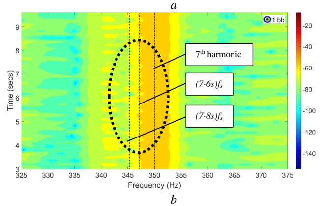
Fig. 9. Harmonics of interest for Motor #2 captured with the minimum required L_w as calculated from the proposed limit: (a) area of (5-4)s f_s and (5-6)s f_s (b) area of (7-6)s f_s and (7-8)s f_s
