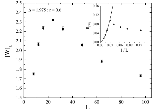
FIG. 5: Finite-size scaling of the disorder-averaged interfacial adsorption [W]_L of the random-bond Blume-Capel model at the disorder-induced continuous transition. The inset illustrates the relevant self-averaging properties in terms of the relative-variance ratio R_{[W]_L} as a function of the inverse system size.
