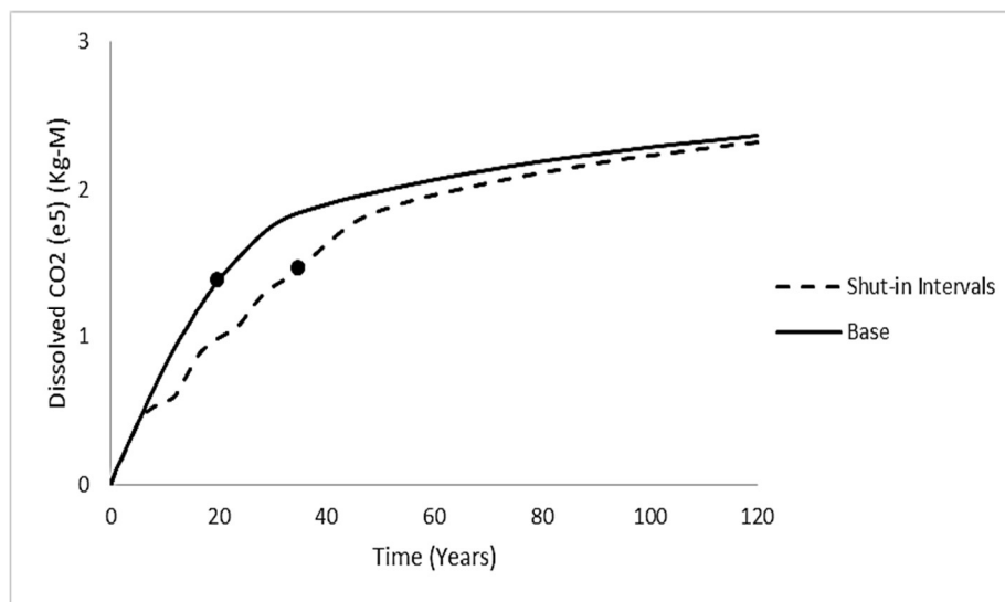
Figure 2. Simulation result for the effect of injection period on CO 2 dissolution in brine vs. time.
