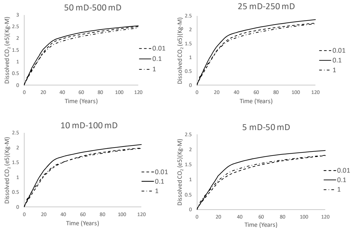
Figure 5. Control of absolute permeability on K_v/K_h ratio on CO_2 dissolution in brine (by changing K_v ).
