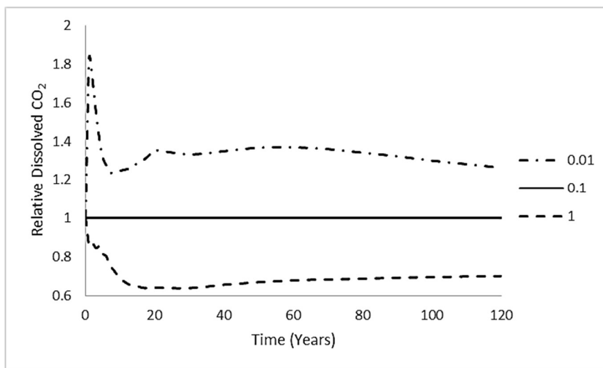
Figure 4. Simulation result for the effect of K_v/K_h ratio on CO_2 dissolution in brine vs. time by changing K_h .
