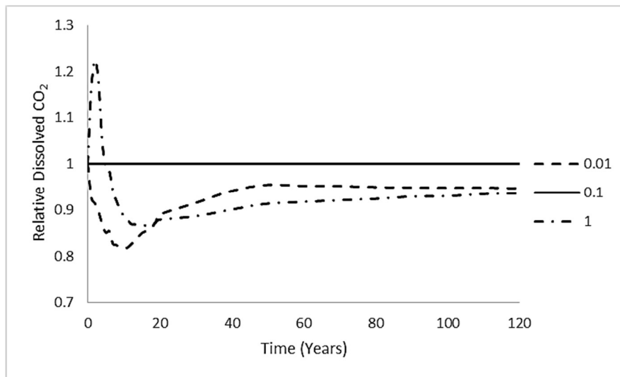
Figure 3. Simulation result for the effect of K_v/K_h ratio on the amount of dissolved CO_2 vs. time by changing K_v .
