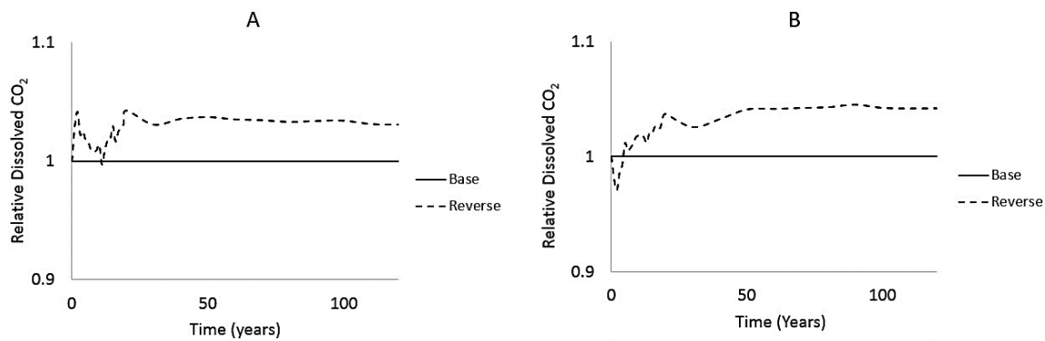
Figure 9. Effect of two layers of permeability heterogeneity on the dissolution of CO 2 in brine in two cases. (A) First simulation with the first set of heterogeneity data, (B) Second simulation with the second set of heterogeneity data.
