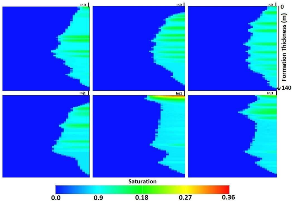
Figure 8. Gas saturation distribution after 120 years in 6 different cases.
