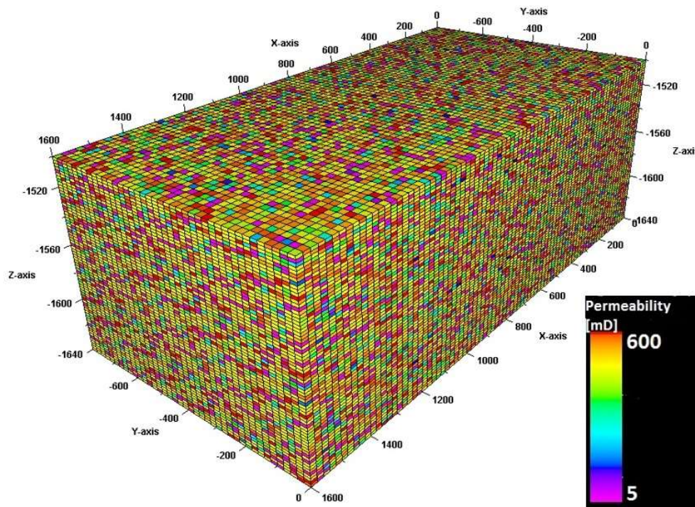
Figure 1. The 3D reservoir simulation model showing the horizontal heterogeneous permeability.
