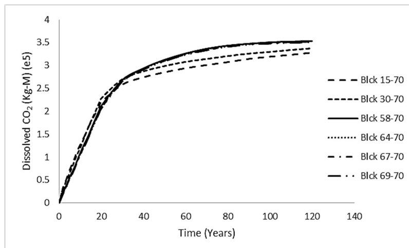
Figure 10. Simulation result for the effect of the number of grid block connections between well and reservoir.
