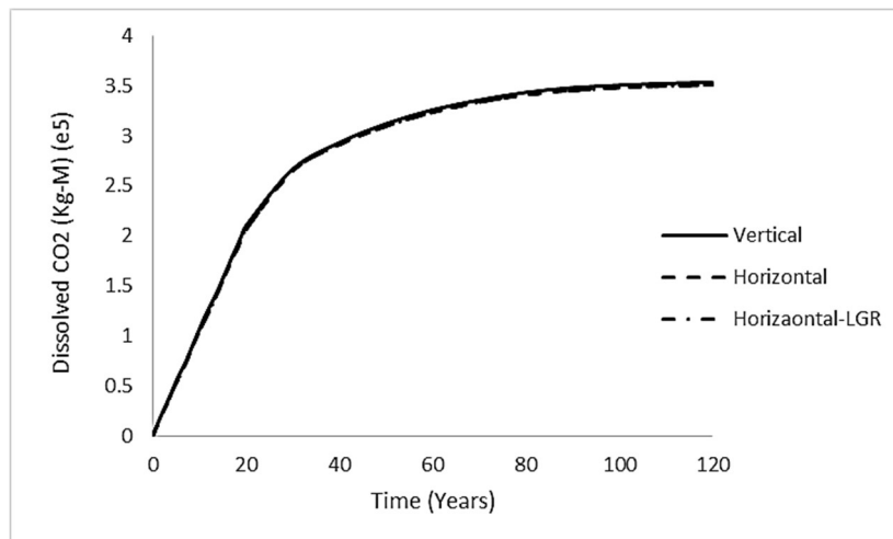
Figure 12. Simulation result for the effect of vertical and horizontal wells on CO 2 dissolution in brine.
