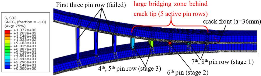
Fig.13 Simulation of a DCB specimen under tension load, showing the first three pin rows in the crack wake (current crack length 36 mm, deformation scale factor 3.0, contour map)
