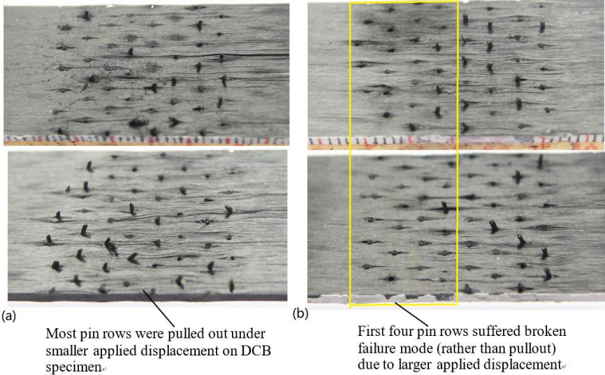
Fig. 12 After fatigue failure: (a) specimen F1-3 tested at smaller applied displacement (Group 1, at 0.8 d_{Pmax} ), (b) specimen F2-2 tested at larger applied displacement (Group 2, at 0.9 d_{Pmax} )
