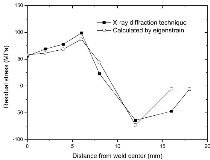
Fig. 15. Evaluated residual stress in the welded stiffened panel.
