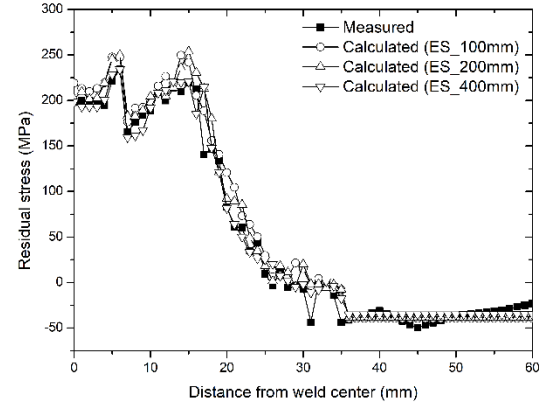
(d) Evaluated residual stress of specimen with 800 mm length
