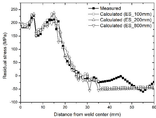
(c) Evaluated residual stress of specimen with 400 mm length
