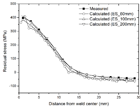
(c) Evaluated residual stress of specimen with 140 mm width
