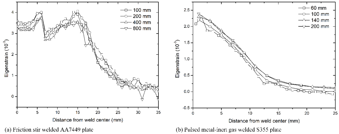
Fig. 9. Eigenstrain distributions derived from residual stresses in specimens of different lengths or widths.
