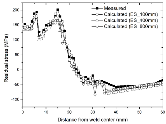
(b) Evaluated residual stress of specimen with 200 mm length
