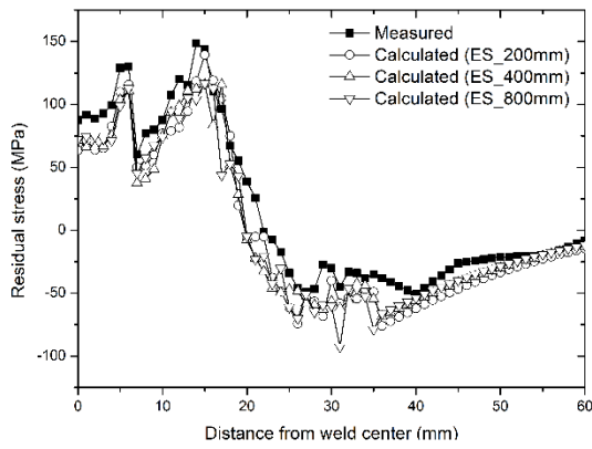
(a) Evaluated residual stress of specimen with 100 mm length
