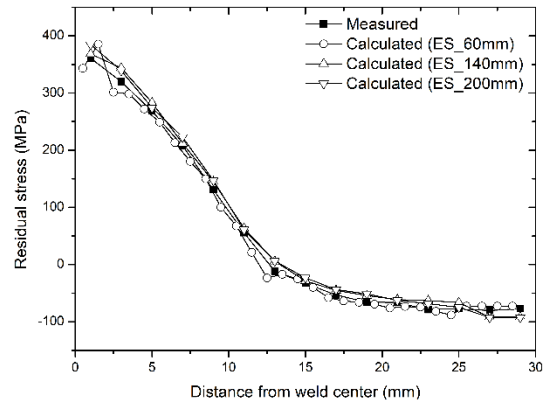
(b) Evaluated residual stress of specimen with 100 mm width
