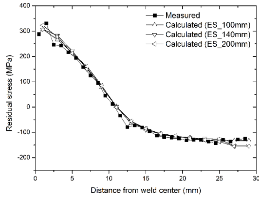
(a) Evaluated residual stress of specimen with 60 mm width
