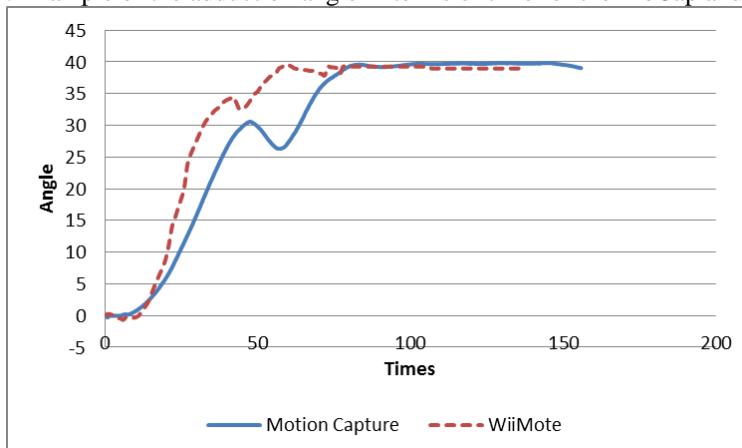
Figure 10: Example of the internal rotation angle in terms of time for the MoCap and Wiimote
