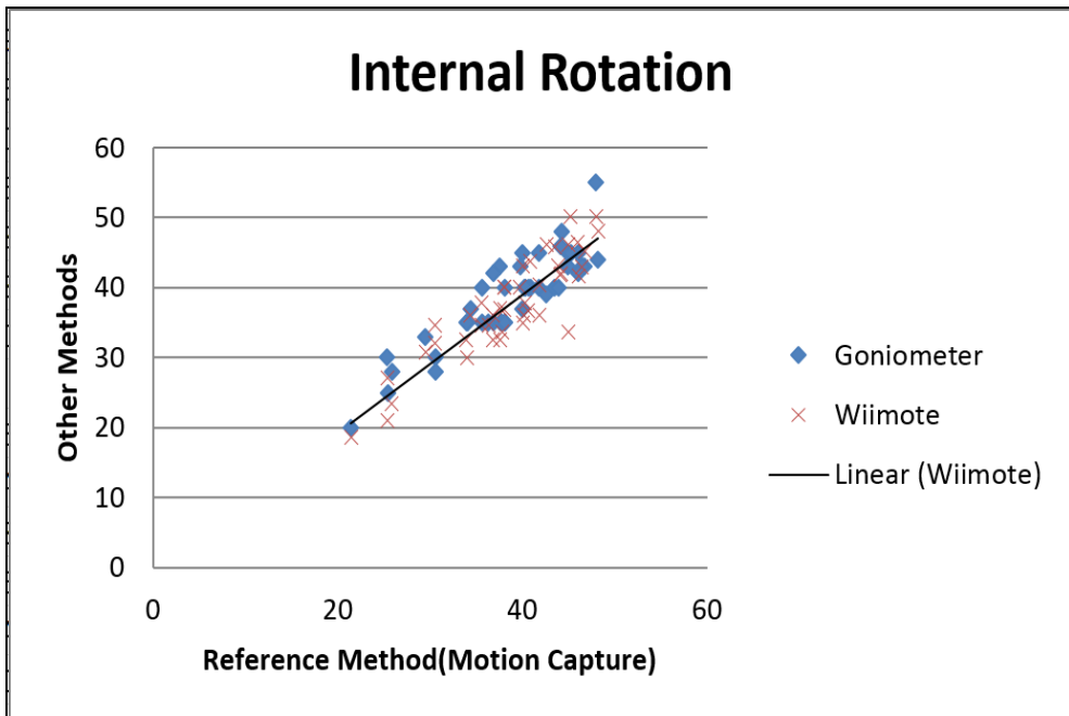
Fig 13: Correlation plot for internal rotation (Vicon MoCap was used as the reference to compare the validity of the Wiimote and the goniometer)
