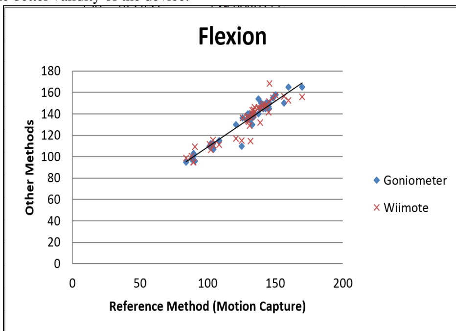
Figure 11 Correlation plot for flexion (motion capture was used as the reference to compare the validity of the Wiimote and the goniometer)
