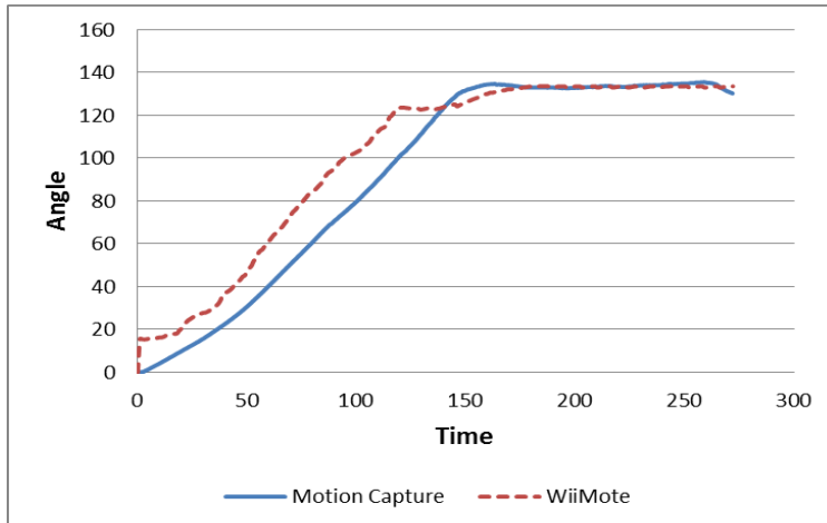
Figure 8: Example of the flexion angle in terms of time for the MoCap and Wiimote
