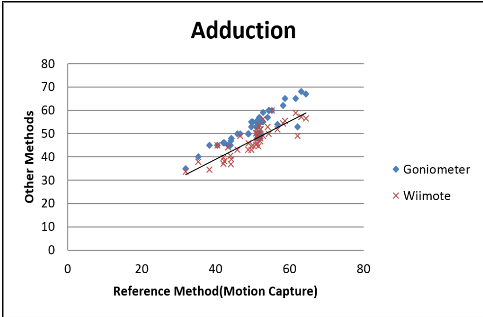
Fig 12: Correlation plot for adduction (Vicon MoCap was used as the reference to compare the validity of the Wiimote and the goniometer)
