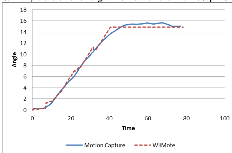
Figure 9: Example of the adduction angle in terms of time for the MoCap and Wiimote
