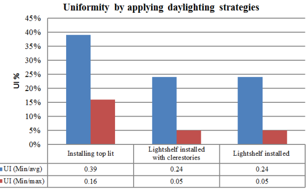
Fig. 18 Uniformity by applying daylighting strategies
