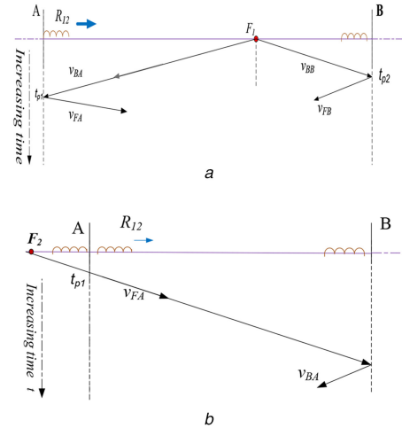
Fig. 3 Conditions for forward and reverse faults
