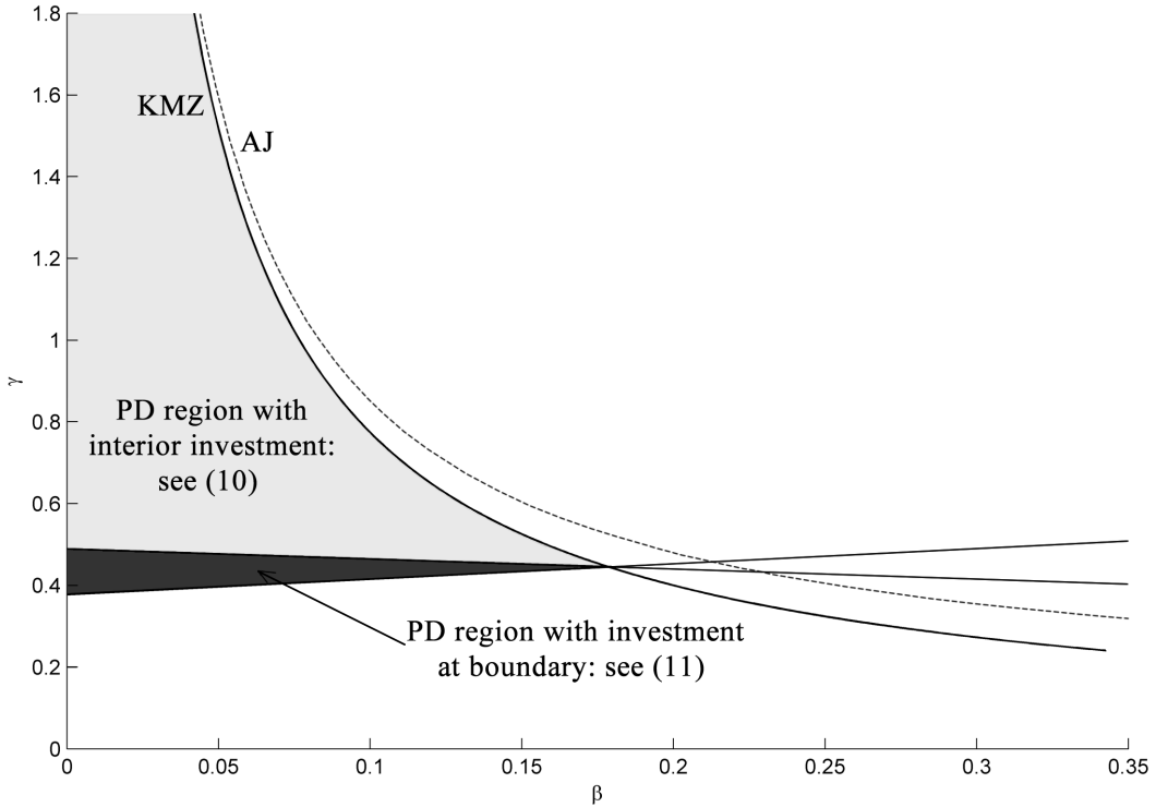
Figure 1: Prisoner's dilemma (PD) region in (\beta, \gamma) space for the KMZ (solid line) and the AJ (dashed line) model. ( a = 2.2, c = 1 and b = 1 )
