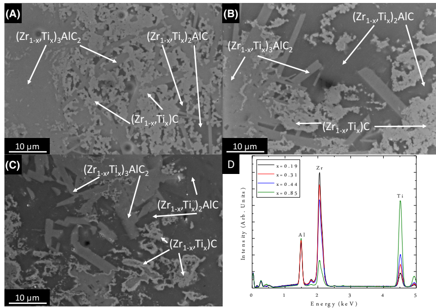
FIGURE 2 SEM micrographs of different (Zr_{1-x}Ti_x)_3AlC_2 quaternary MAX phases (A-C) and EDS spectra for different x stoichiometries; (A) Zr_2TiAlC_2 , (B) Zr_{1.5}Ti_{1.5}AlC_2 , (C) ZrTi_2AlC_2 , (D) EDS spectra. (Zr_{1-x}Ti_x)_3AlC_2 , (Zr_{1-x}Ti_x)_2AlC and (Zr_{1-x}Ti_x)C label the different phases detected in each composition. Figure 2C illustrates the presence of (Zr_{1-x}Ti_x)_2AlC in ZrTi_2AlC_2 but note that it was distributed unevenly in the microstructure [Color figure can be viewed at wileyonlinelibrary.com ]
