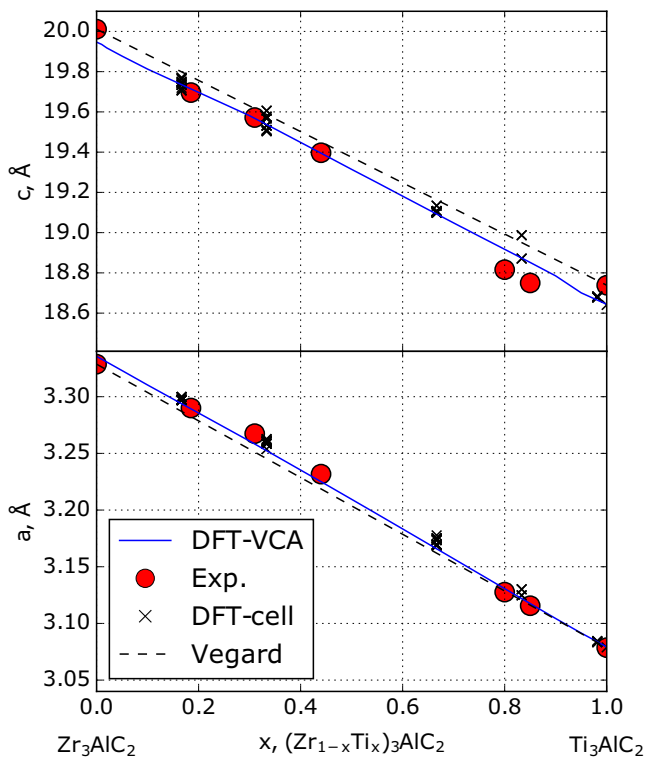
FIGURE 3 Determined and calculated lattice parameters of (Zr_{1-x}Ti_x)_3AlC_2 quaternary MAX phases. The DFT-cell data refers to point defect calculations of Ti_{Zr} and Zr_{Ti} defects [Color figure can be viewed at wileyonlinelibrary.com ]
