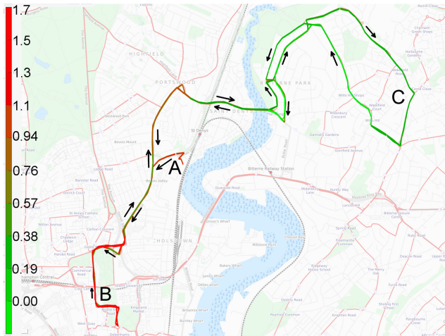
Fig. 6 Vehicle position trace recorded by the telematics unit on Test 2, Vehicle 2. The trace colour denotes \text{NO}_x from 0 g/km (green) to 1.7 g/km (red). Labelled are the bus depot (A), the main pedestrian thoroughfare in the city centre (B) and the hilly residential area (C). Driving direction is indicated by the arrows. Map data © OpenStreetMap contributors [11]
