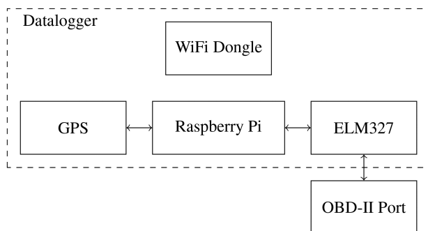
Fig. 3 Schematic of the OBD-II datalogger unit
