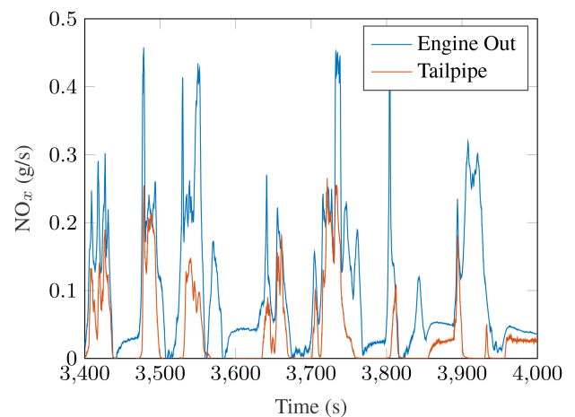
Fig. 9 Engine output \text{NO}_x and tailpipe \text{NO}_x during a period of nominal temperature operation
