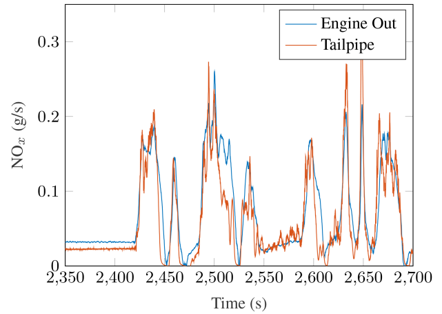
Fig. 8 Catalyst cooling reduces \text{NO}_x conversion to 14% in urban sections of the route
