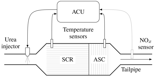
Fig. 1 Schematic of an SCR aftertreatment system, including an ASC and aftertreatment control unit (ACU)
