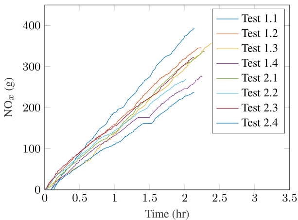
Fig. 5 Cumulative NO x output during each of the eight tests, where test x , y refers to vehicle x , test number y in Table 1
