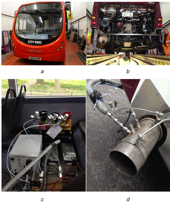
Fig. 2 Vehicles used in this work and the PEMS equipment (a) Wrightbus Streetlite DF, (b) Engine bay, (c) Horiba OBS-2200, (d) Exhaust sample pipe
