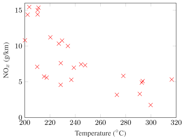
Fig. 10 Mean SCR outlet gas temperature versus mass of NO x emitted per kilometre on Test 2, Vehicle 2
