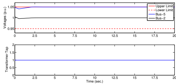
Figure 6. Bus voltages (top) and tap position (bottom) scenario for case-3
