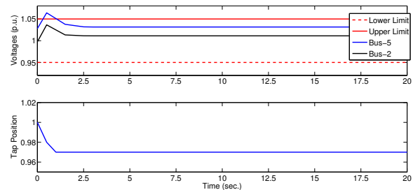
Figure 4. Bus voltages (top) and tap position (bottom) scenario for case-2
