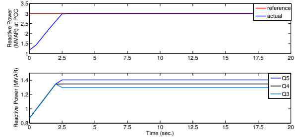
Figure 5. Reactive power exchange at PCC (top) and contribution of each SWF's (bottom) for case-2
