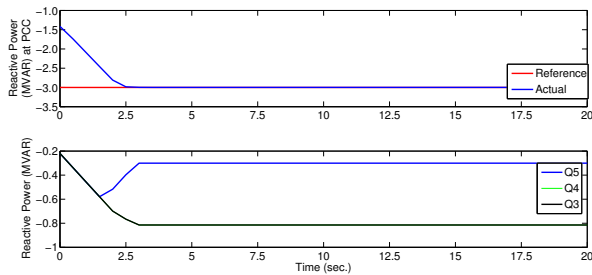
Figure 7. Reactive power exchange at PCC (top) and contribution of each SWF's (bottom) for case-3
