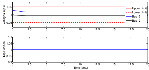
Figure 2. Bus voltages (top) and Tap position (bottom) scenario for case-1
