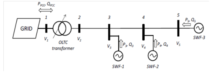
Figure 1. 5-bus test system
