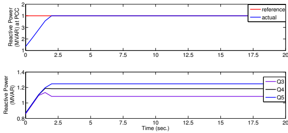
Figure 3. Reactive power exchange at PCC for case-1 (top) and each SWF's contribution (bottom)
