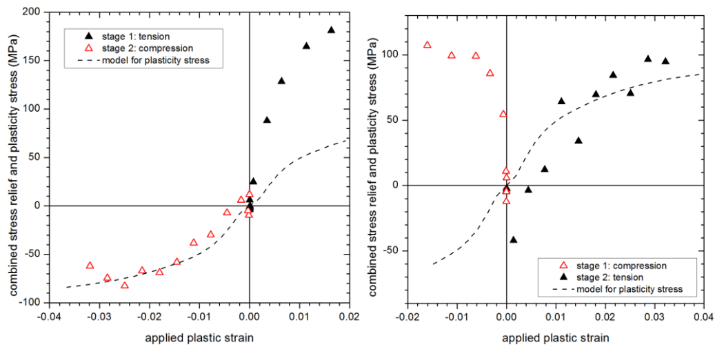
Figure 9. The development of an apparent plasticity stress as a function of plastic strain at 20°C. (a) The tension-first test. Solid symbols are for the initial tension and open symbols for the subsequent compression. (b) The compression-first test. Open symbols are for the initial compression and closed symbols for the subsequent tension. In both (a) and (b) the dashed lines are from Figure 8 assuming tension/compression symmetry.
