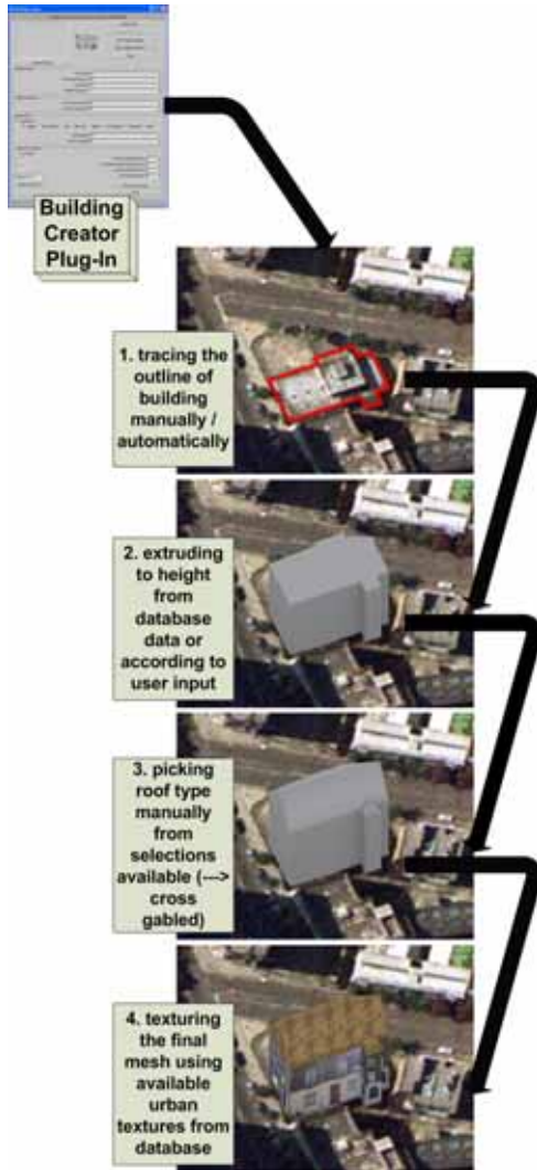
Figure 6: step-by-step operation of the Building Creator script, creating a random building from a real-world map
