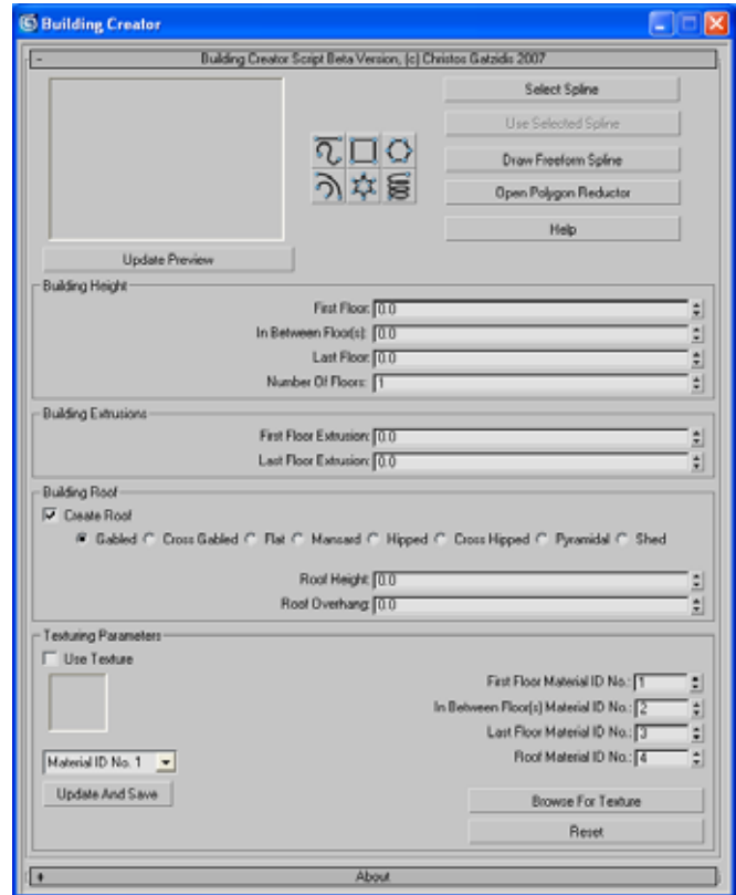
Figure 5: Building Creator script interface
