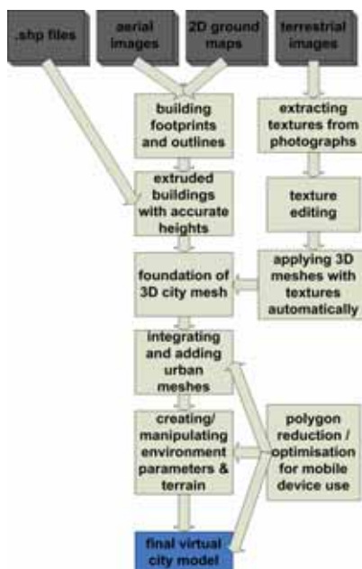
Figure 1: framework diagram of Virtual City Maker
