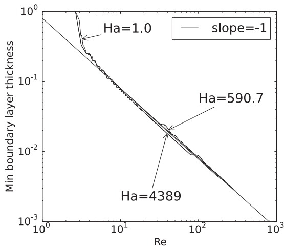
FIG. 6. Boundary layer thicknesses for Ha \approx 1.0, 590.7, \text{ and } 4389 .
