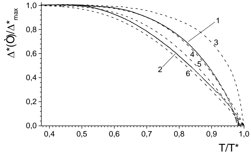
Fig. 3. The temperature dependence of the PG for the \text{YBa}_2\text{Cu}_{3-y}\text{Al}_y\text{O}_{7-\delta} single crystal, in \Delta^*(T)/\Delta_{\max} versus T/T^* coordinates, where \Delta_{\max} is the \Delta^* value in the plateau, away from T^* . The numbering of the curves corresponds to the numbers in the Fig. 1. Dotted lines for the \Delta^*(T)/\Delta(0) versus T/T^* dependence were calculated according Eq. (2) and (3) for the values of the crossover parameters \mu/\Delta(0)=10 (limit of the BCS, curve 3) and \mu/\Delta(0) = -2, -5, -10 (limit of the BEC, curves 4-6).
