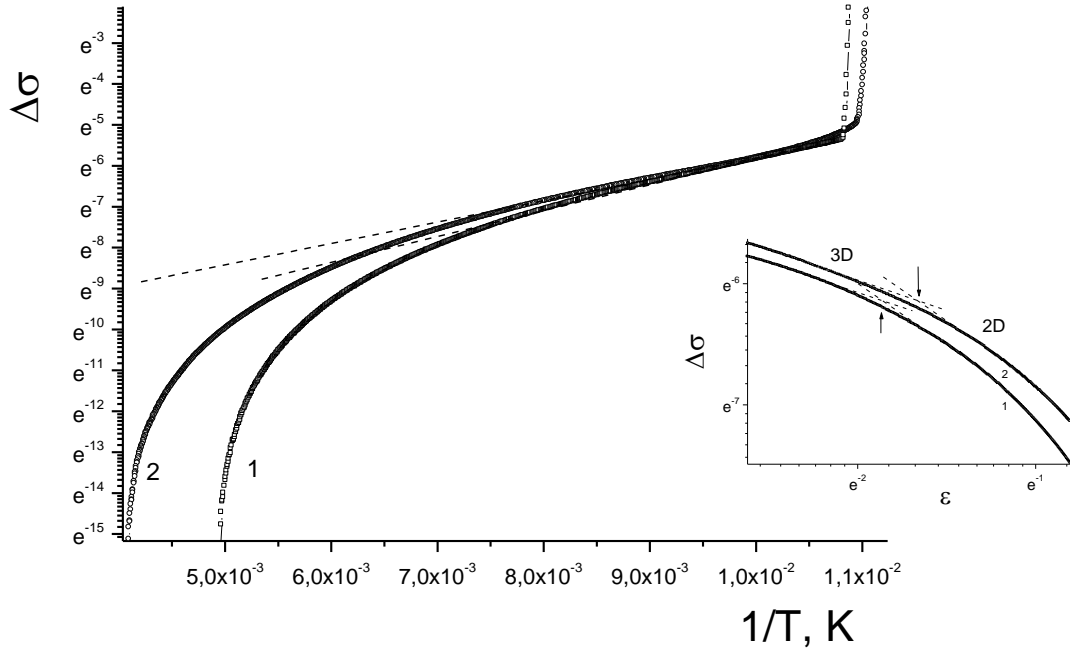
Fig. 2. The temperature dependence of the excess conductivity in the ab-plane for the \text{YBa}_2\text{Cu}_{3-y}\text{Al}_y\text{O}_{7-\delta} single crystal in \ln\Delta\sigma - 1/T versus \ln\Delta\sigma - \ln\varepsilon coordinates (inset). The names (notation) of the curves is relevant to the figure 1. The dashed lines in figure 2 shows the approximation of equation (5), and in the inset, the straight lines – the approximation with a slope \text{tg}\alpha_1 \approx -0.5 (3D regime) and \text{tg}\alpha_2 \approx -1.0 (2D regime). The arrows show the point of the 2D-3D crossover.
