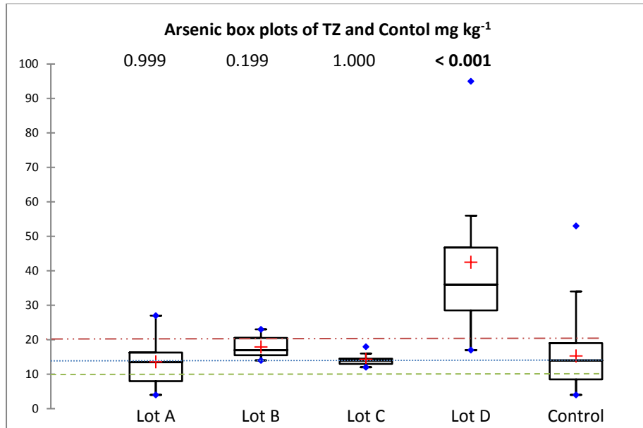
Figure 2 Box plots for arsenic concentrations in the soil of the transpiration zones of lots A, B, C and D and the non-irrigated controls as well as the probability values of each lot compared to the control samples using the Kruskal-Wallis test. Bold p values indicate significant differences to the control samples. (See Figure 1 for box plot description). The dotted line represents the median of the control samples in relation to all lots. The dashed line represents the BG. The dashed and dotted line represents the CCL.
