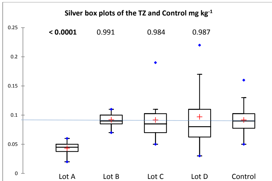
Figure 12 Box plots for silver concentrations in the soil of the transpiration zones of lots A, B, C and D and the non-irrigated controls as well as the probability values of each lot compared to the control samples using the Kruskal-Wallis test. Bold p values indicate significant differences to the control samples. (See Figure 1 for box plot description). The dotted line represents the median of the control samples in relation to all lots. The soil line is not represented as the CEQG is 20 mg kg -1 .
