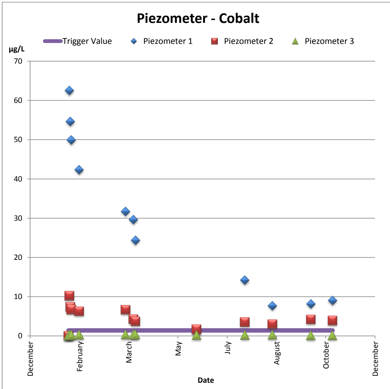
Figure 6 groundwater Cobalt concentrations ( \mu\text{g L}^{-1} ) and the Australian and New Zealand freshwater quality guideline default trigger value for ecosystem protection
