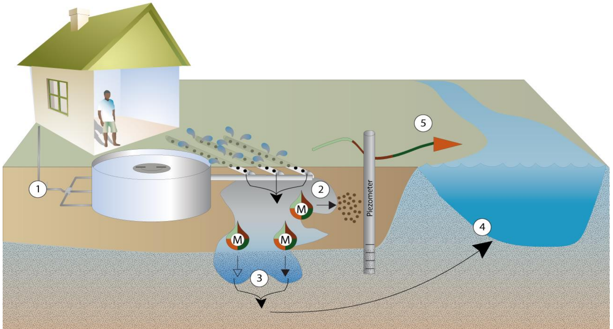
Figure 1 Conceptual diagram of greywater irrigation and metal movement; Household sources of metals (1) stored in a concrete tank then distributed via greywater sub-surface irrigation resulting in direct and indirect metal transportation (metal soil adsorption - direct (2); metal leaching - direct and indirect (3)); lateral movement of contaminated groundwater to surface water (4); and surface runoff with soil erosion - (not assessed in this study (5)) and the impacts in three connected environmental compartments: soil; groundwater (via sampling at the piezometer(s); and surface water.
