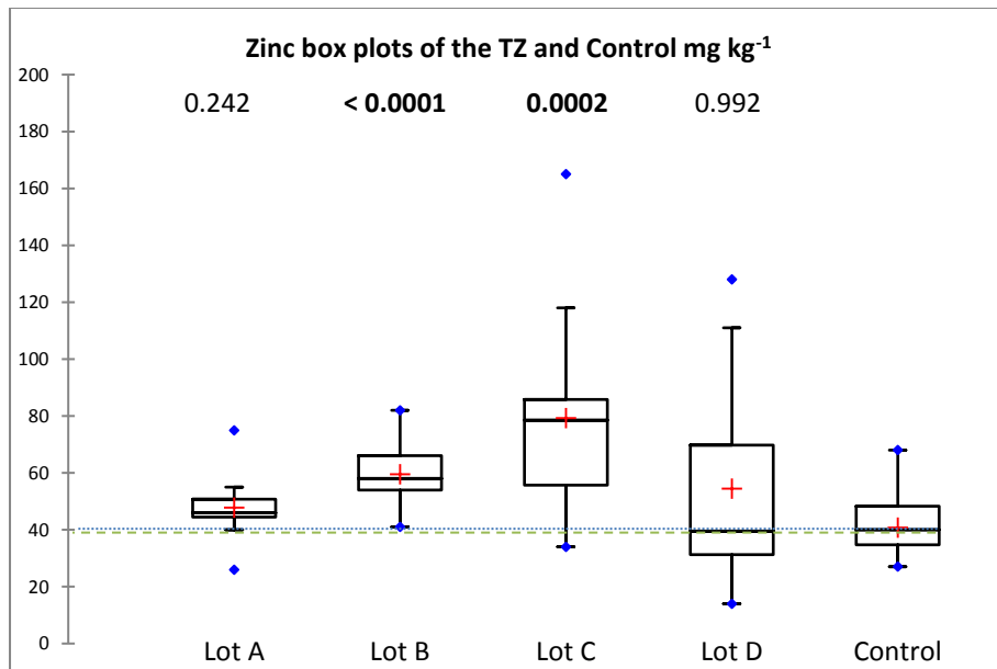
Figure 13 Box plots for zinc concentrations in the soil of the transpiration zones of lots A, B, C and D and the non-irrigated controls as well as the probability values of each lot compared to the control samples using the Kruskal-Wallis test. Bold p values indicate significant differences to the control samples. (See Figure 1 for box plot description). The dotted line represents the median of the control samples in relation to all lots. The dashed line represents the BG. The dashed and dotted line is not represented as the CCL is 300 mg kg -1 .
