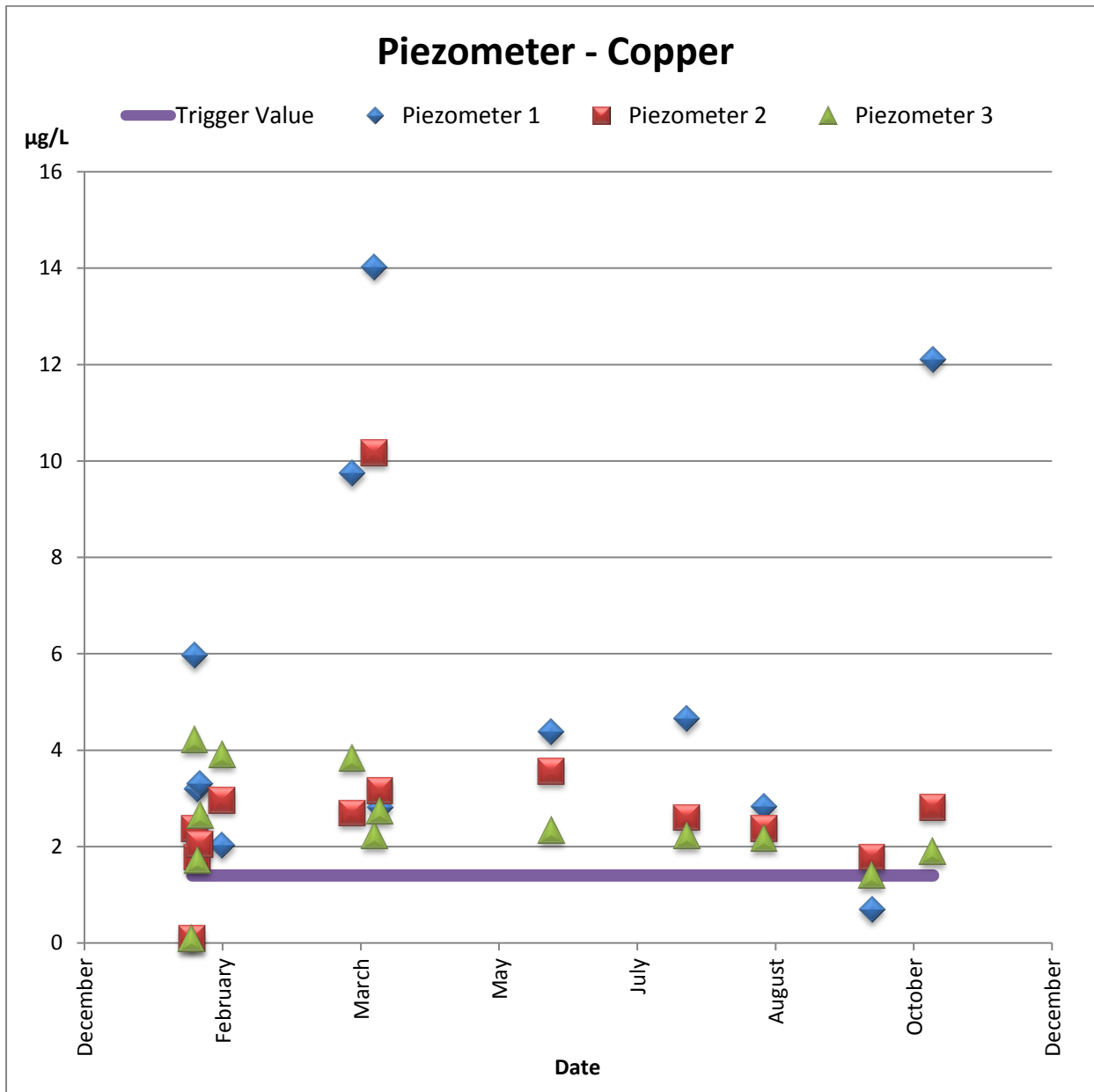
Figure 7 groundwater Copper concentrations ( \mu\text{g L}^{-1} ) and the Australian and New Zealand freshwater quality guideline default trigger value for ecosystem protection
