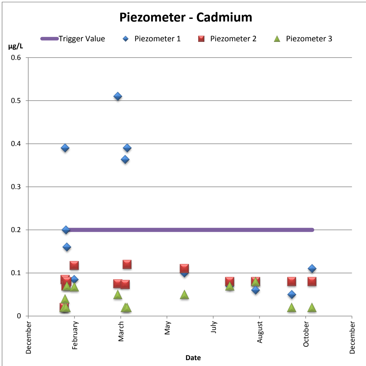
Figure 4 groundwater Cadmium concentrations ( \mu\text{g L}^{-1} ) and the Australian and New Zealand freshwater quality guideline default trigger value for ecosystem protection
