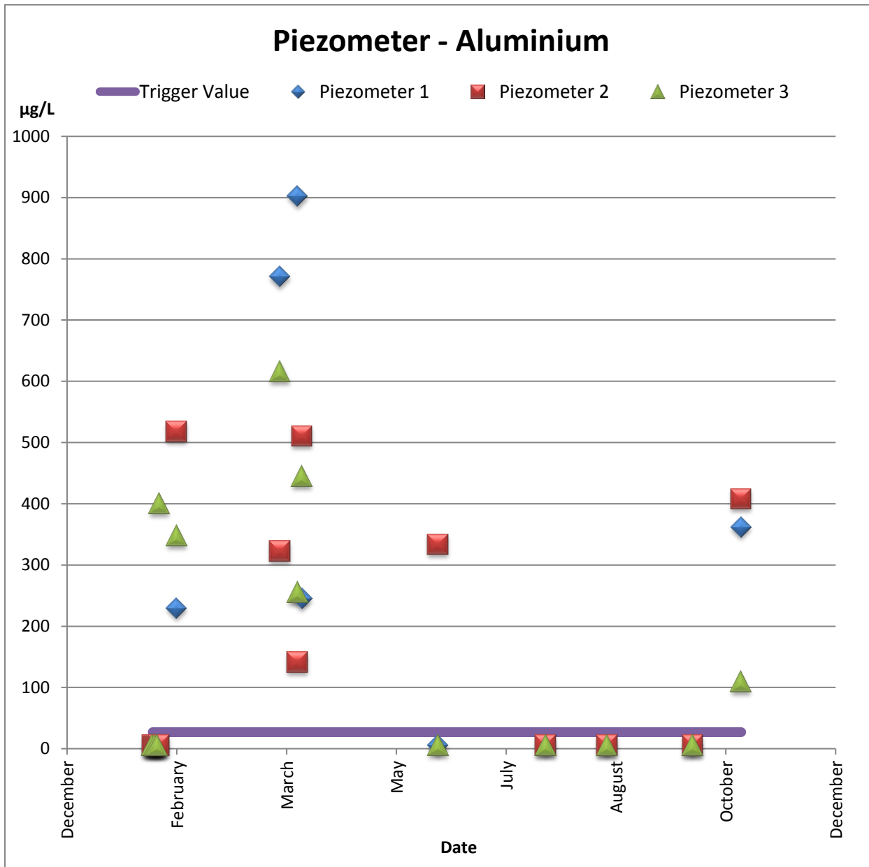
Figure 1 groundwater aluminium concentrations ( \mu\text{g L}^{-1} ) and the Australian and New Zealand freshwater quality guideline default trigger value for ecosystem protection
