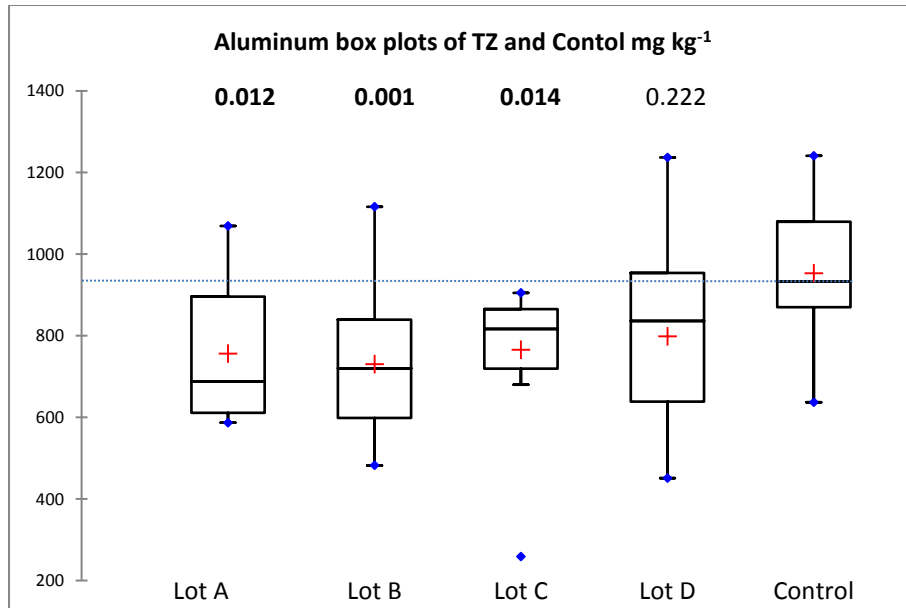
Figure 1 Box plots for aluminum concentrations in the soil of the transpiration zones (TZ) of lots A, B, C and D and the non-irrigated controls as well as the probability values of each lot compared to the control samples using the Kruskal-Wallis test. Bold p values indicate significant differences to the control samples. (The lower and upper ends of each box are the 1st quartile and 3rd quartile of the data. The line within each box is the median while the red cross is the mean. The whiskers displayed at both ends of the “box” represent values which are beyond first and third quartiles while the diamonds are the minimum and maximum values. All subsequent TZ and control box plot figures are represented the same way.). The dotted line represents the median of the control samples in relation to all lots.
