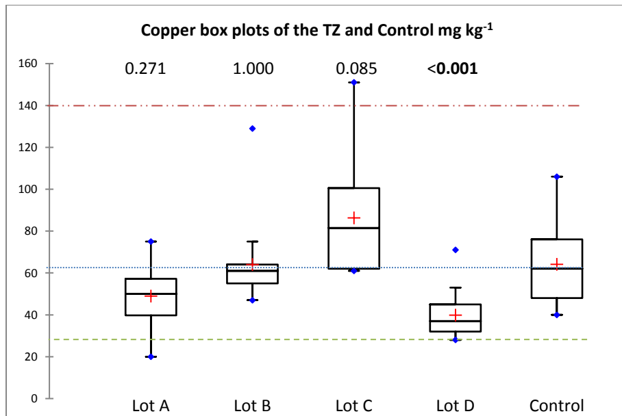
Figure 7 Box plots for copper concentrations in the soil of the transpiration zones of lots A, B, C and D and the non-irrigated controls as well as the probability values of each lot compared to the control samples using the Kruskal-Wallis test. Bold p values indicate significant differences to the control samples. (See Figure 1 for box plot description). The dotted line represents the median of the control samples in relation to all lots. The dashed line represents the BG. The dashed and dotted line represents the CCL.
