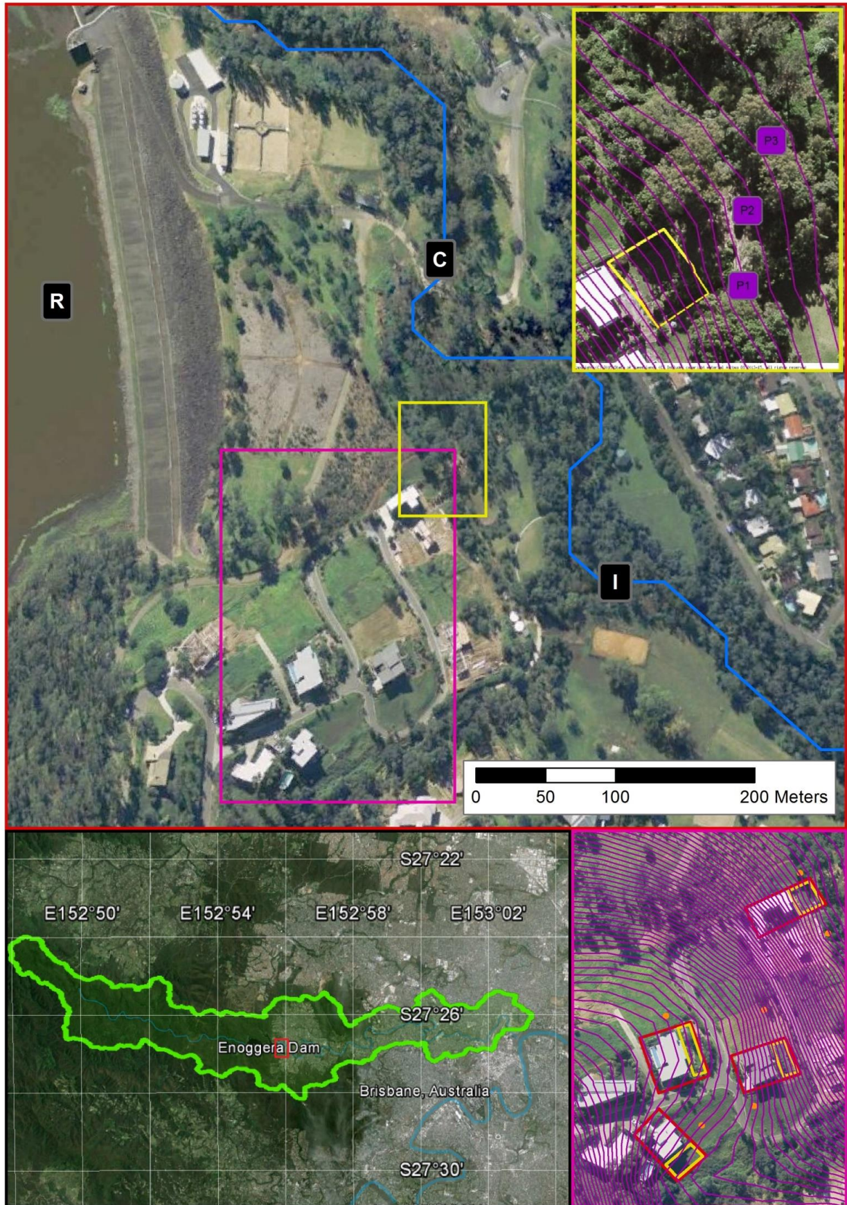
Figure 2 Ariel photograph with four zoom levels showing: Zoom 1 (in black box); location of study area at the base of the High Ecological Valve - Enoggera Catchment 10 km west of Brisbane. Zoom 2 (red box); study site and Enoggera Creek location (blue line) with the surface water sites marked (black and grey boxes); reference site (R) in Enoggera Dam, upstream control (C) site and downstream impact (I) site. Zoom 3 (pink box); indicates the general topography (pink contours) of the four selected greywater irrigated lots for detailed investigation (red outline), transpiration zones (yellow outline) and control (vacant non-irrigated) sampling sites (orange circles). Zoom 4 (yellow box); lot D with the location of transpiration zone (yellow outline) and the piezometers (purple numbered P1 to P3). FIGURE 2
