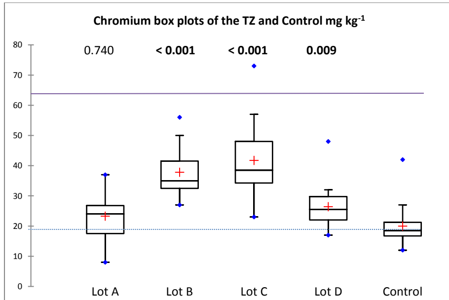
Figure 5 Box plots for chromium concentrations in the soil of the transpiration zones of lots A, B, C and D and the non-irrigated controls as well as the probability values of each lot compared to the control samples using the Kruskal-Wallis test. Bold p values indicate significant differences to the control samples. (See Figure 1 for box plot description). The dotted line represents the median of the control samples in relation to all lots. The solid line represents the CEQG - only used when there are no BG or CCL.
