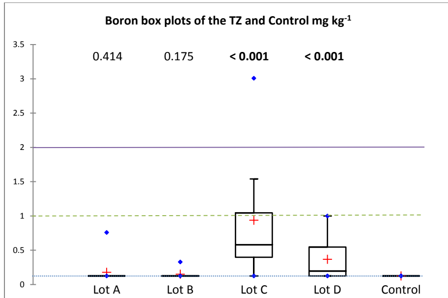
Figure 3 Box plots for boron concentrations in the soil of the transpiration zones of lots A, B, C and D and the non-irrigated controls as well as the probability values of each lot compared to the control samples using the Kruskal-Wallis test. Bold p values indicate significant differences to the control samples. (See Figure 1 for box plot description). The dotted line represents the median of the control samples in relation to all lots. The dashed line represents the BG. The solid line represents the CEQG - only used when there are no BG or CCL.
