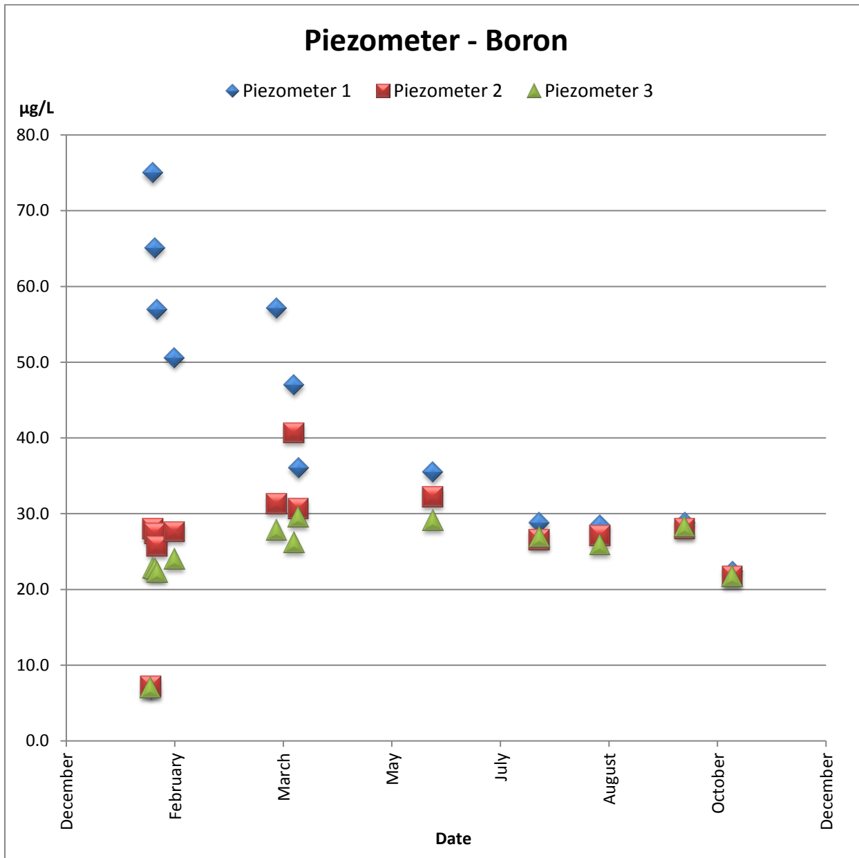
Figure 3 groundwater Boron concentrations ( \mu\text{g L}^{-1} ) and the Australian and New Zealand freshwater quality guideline default trigger value for ecosystem protection
