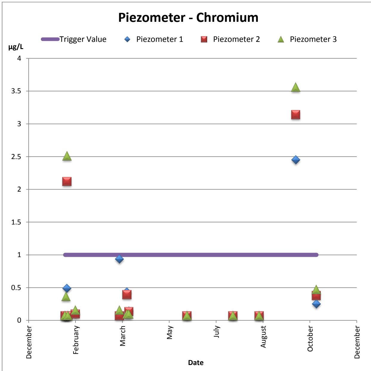
Figure 5 groundwater Chromium concentrations ( \mu\text{g L}^{-1} ) and the Australian and New Zealand freshwater quality guideline default trigger value for ecosystem protection
