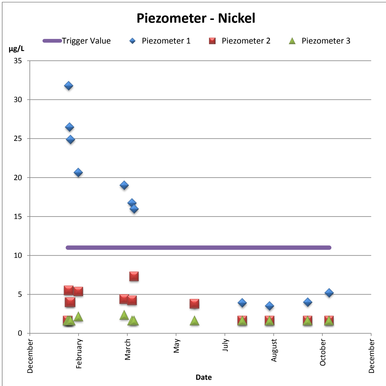
Figure 11 groundwater Nickel concentrations ( \mu\text{g L}^{-1} ) and the Australian and New Zealand freshwater quality guideline default trigger value for ecosystem protection
