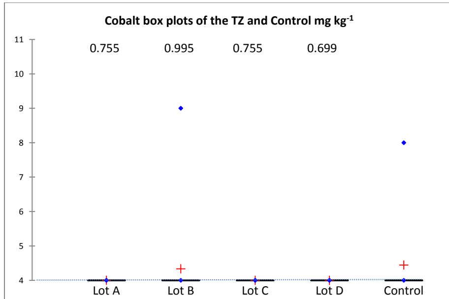
Figure 6 Box plots for cobalt concentrations in the soil of the transpiration zones of lots A, B, C and D and the non-irrigated controls as well as the probability values of each lot compared to the control samples using the Kruskal-Wallis test. Bold p values indicate significant differences to the control samples. (See Figure 1 for box plot description). The dotted line represents the median of the control samples in relation to all lots. The dashed line is not represents as the BG is 27 mg kg -1 . The solid line is not represented as the CEQG is 50 mg kg -1 .
