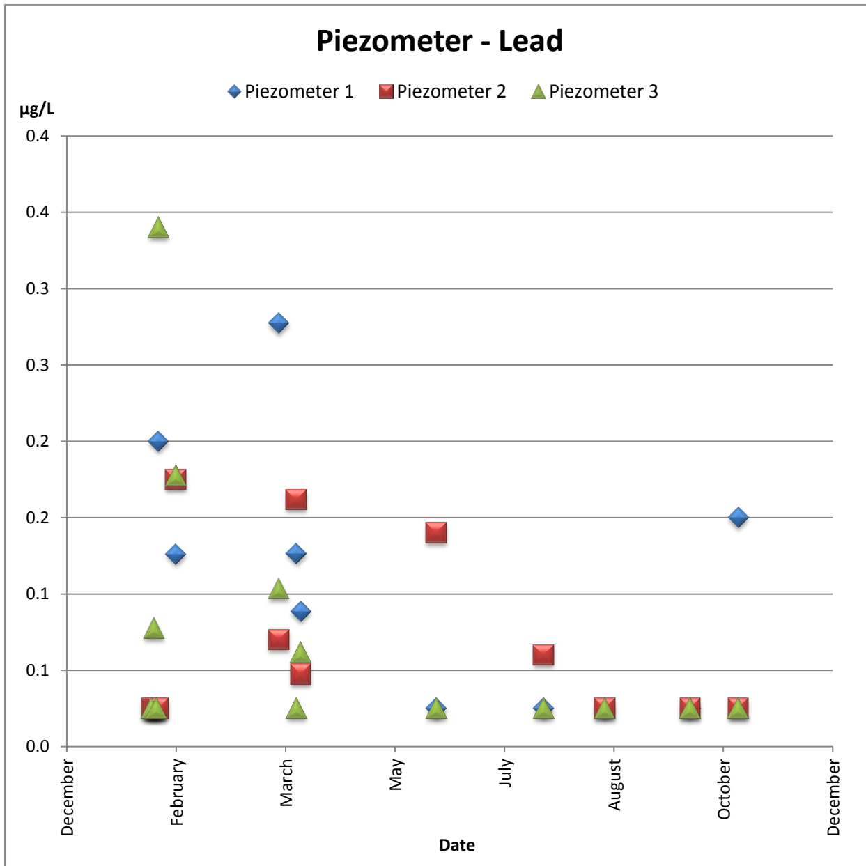
Figure 9 groundwater Lead concentrations ( \mu\text{g L}^{-1} ) and the Australian and New Zealand freshwater quality guideline default trigger value for ecosystem protection
