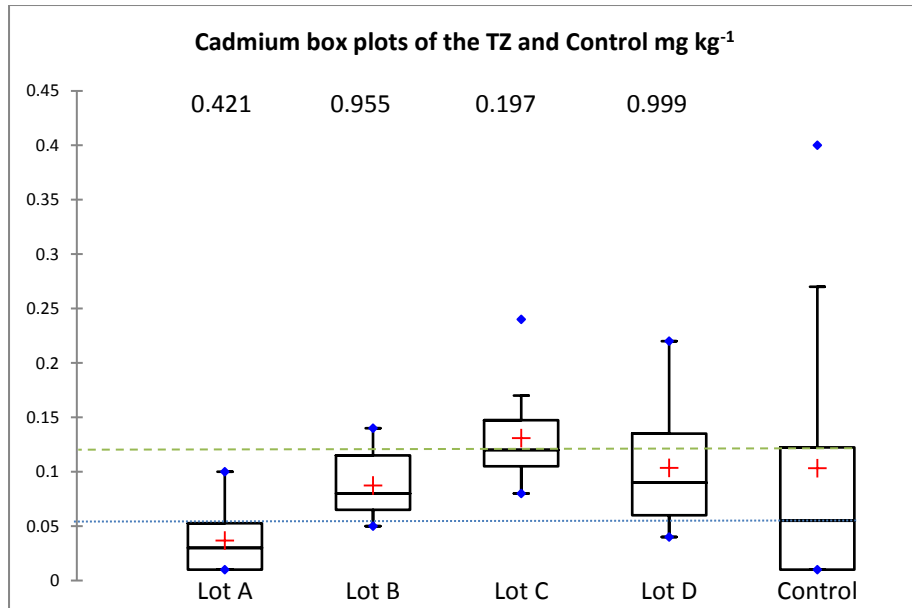
Figure 4 Box plots for cadmium concentrations in the soil of the transpiration zones of lots A, B, C and D and the non-irrigated controls as well as the probability values of each lot compared to the control samples using the Kruskal-Wallis test. Bold p values indicate significant differences to the control samples. (See Figure 1 for box plot description). The dotted line represents the median of the control samples in relation to all lots. The dashed line represents the BG. The dashed and dotted line is not represented as the CCL is 2 mg kg -1 .
