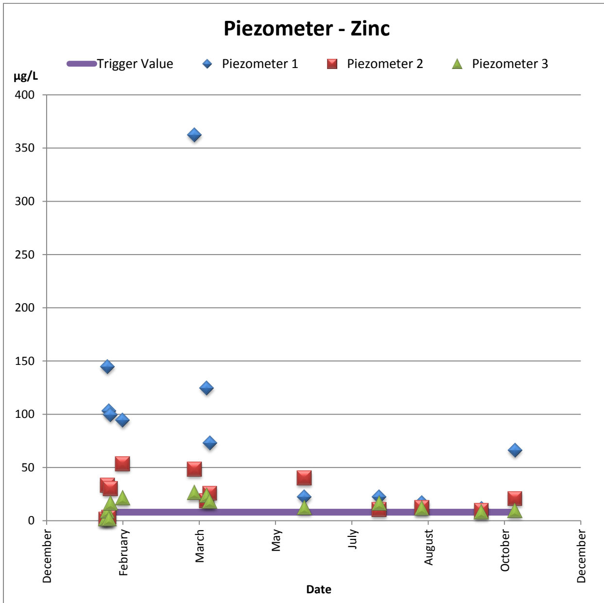
Figure 12 groundwater Zinc concentrations ( \mu\text{g L}^{-1} ) and the Australian and New Zealand freshwater quality guideline default trigger value for ecosystem protection
