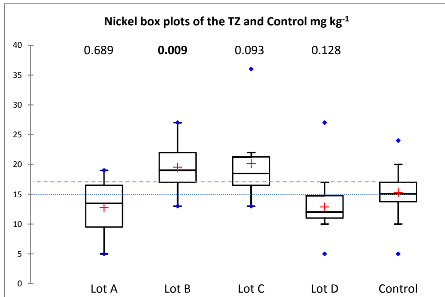
Figure 11 Box plots for nickel concentrations in the soil of the transpiration zones of lots A, B, C and D and the non-irrigated controls as well as the probability values of each lot compared to the control samples using the Kruskal-Wallis test. Bold p values indicate significant differences to the control samples. (See Figure 1 for box plot description). The dotted line represents the median of the control samples in relation to all lots. The dashed line represents the BG. The dashed and dotted line is not represented as the CCL is 85 mg kg -1 .
