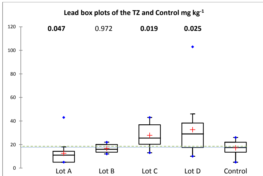
Figure 9 Box plots for lead concentrations in the soil of the transpiration zones of lots A, B, C and D and the non-irrigated controls as well as the probability values of each lot compared to the control samples using the Kruskal-Wallis test. Bold p values indicate significant differences to the control samples. (See Figure 1 for box plot description). The dotted line represents the median of the control samples in relation to all lots. The dashed line represents the BG. The dashed and dotted line is not represented as the CCL is 260 mg kg -1 .
