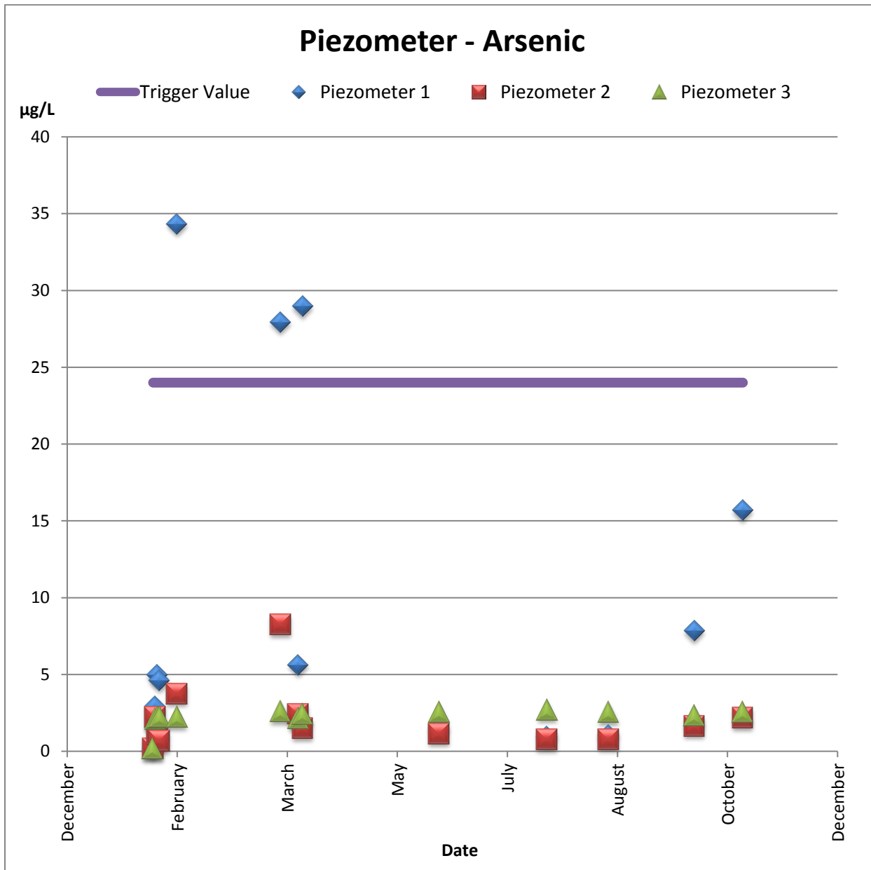
Figure 2 groundwater Arsenic concentrations ( \mu\text{g L}^{-1} ) and the Australian and New Zealand freshwater quality guideline default trigger value for ecosystem protection
