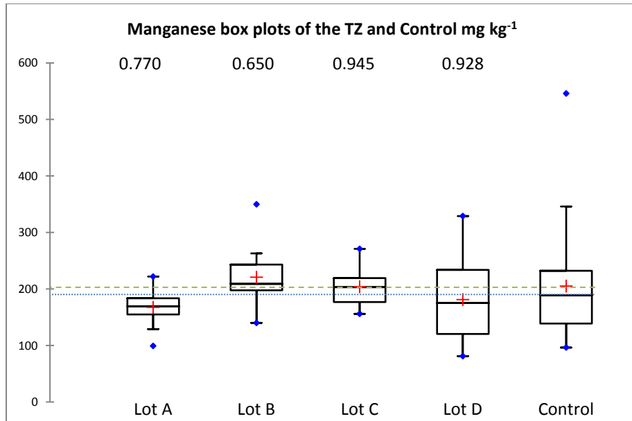
Figure 10 Box plots for manganese concentrations in the soil of the transpiration zones of lots A, B, C and D and the non-irrigated controls as well as the probability values of each lot compared to the control samples using the Kruskal-Wallis test. Bold p values indicate significant differences to the control samples. (See Figure 1 for box plot description). The dotted line represents the median of the control samples in relation to all lots. The dashed line represents the BG.
