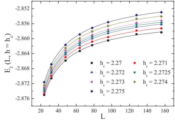
FIG. 4. (Color online) FSS behavior of the bond part of the energy density at the seven candidate values of the critical random-field strength h_c . The lines are fittings of the form (4).
