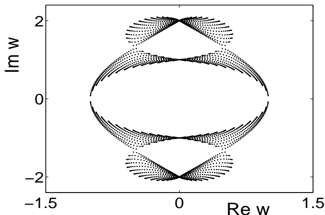
Figure 2: The partition function zeroes in the complex w = 2 \sinh(2\beta) plane for the anisotropic ( J_2 = 3J_1 ) L = M = 2N = 40 Ising model with Brascamp-Kunz boundary conditions.
