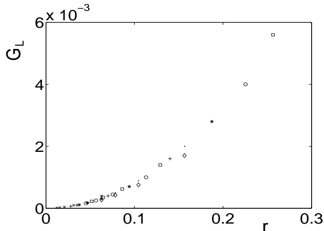
Figure 11: The distribution of zeroes near the physical critical point 1/2\kappa = 2 for free Wilson fermions with L = 50 - 250 and j = 1 - 2 ( \times ), j = 3 - 6 ( + ), j = 7 - 8 ( * ), j = 9 - 12 ( \circ ), j = 13 - 16 ( \square ), j = 17 - 18 ( \diamond ), j = 19 - 23 ( \bullet ).
