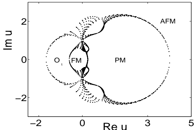
Figure 7: The partition function zeroes in the u = \exp(-2\beta) plane for the bathroom-tile Ising model (3.6) with L = M = N = 40 . Here AFM, PM, FM and O_1 indicate the anti-ferromagnetic, paramagnetic, ferromagnetic and unphysical phases, respectively.
