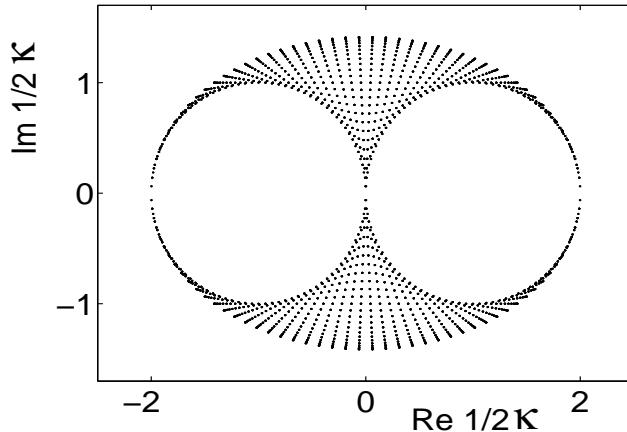
Figure 10: The partition function zeroes for the L = 50 free Wilson fermions in the complex 1/2\kappa plane.
