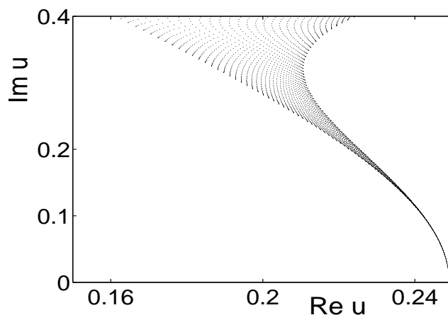
Figure 8: The bathroom-tile Ising zeroes near the ferromagnetic critical point u = 0.2490384\dots for L = M = N = 200 .
