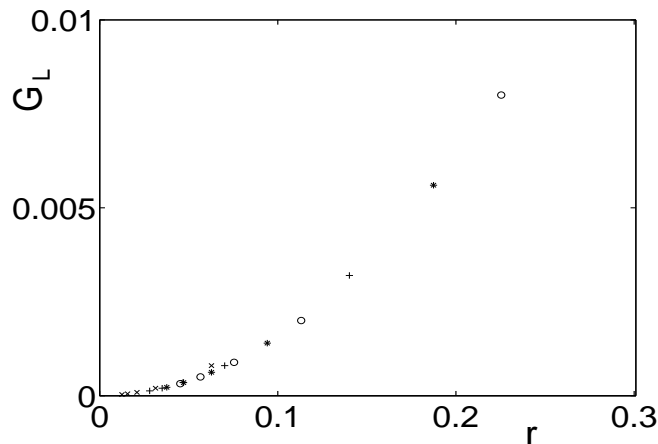
Figure 12: The distribution of zeroes near the artefactual critical point 1/2\kappa = 0 for free Wilson fermions with L = 50 - 250 and j = 1 - 2 ( \times ), j = 3 - 6 ( + ), j = 7 - 8 ( * ), j = 9 - 12 ( \circ ).
