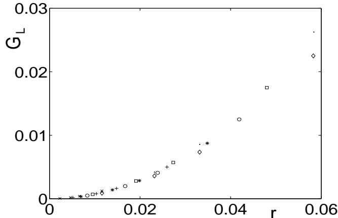
Figure 9: The distribution of zeroes for the bathroom-tile Ising model with L = M = N = 40 - 200 and j = 1 - 4 ( \times ), j = 5 - 12 ( + ), j = 13 - 16 ( * ), j = 17 - 24 ( \circ ), j = 25 - 32 ( \square ), j = 33 - 40 ( \diamond ), j = 41 - 44 ( \bullet ).
