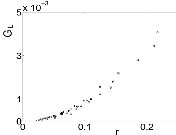
Figure 3: The distribution of zeroes near w = 1 for the anisotropic Ising model with anisotropy ratio R = 3 subject to Brascamp-Kunz boundary conditions for L = 40 - 140 and j = 1 ( \times ), j = 2 ( + ), j = 3 ( * ), j = 4 ( \circ ), j = 5 ( \square ), j = 6 ( \diamond ), j = 7 ( \bullet ), j = 8 ( \star ).
