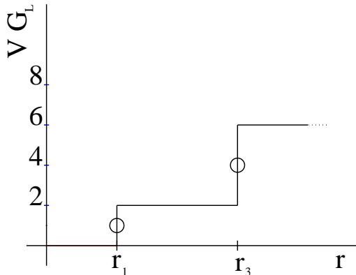
Figure 1: Schematic plot of cumulative density of zeroes as defined by (2.12). In this example, where the volume, V , is fixed, r_1 = r_2 are 2-fold degenerate, while r_3 = \dots = r_6 are 4-fold degenerate.
