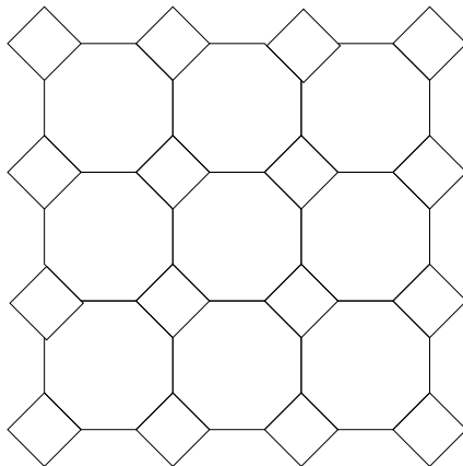
Figure 6: The bathroom tile lattice.
