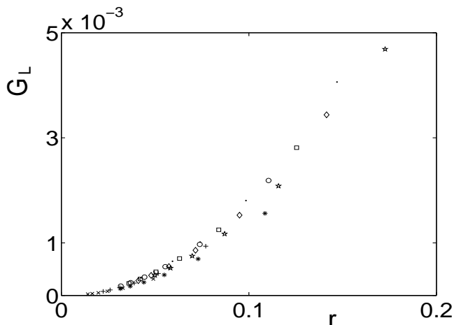
Figure 5: The distribution of zeroes near w = 1 for the Ising model with anisotropy ratio R = 2 subject to Brascamp-Kunz boundary conditions for L = 40 - 140 and j = 1 ( \times ), j = 2 ( + ), j = 3 ( * ), j = 4 ( \circ ), j = 5 ( \square ), j = 6 ( \diamond ), j = 7 ( \bullet ), j = 8 ( \star ).
