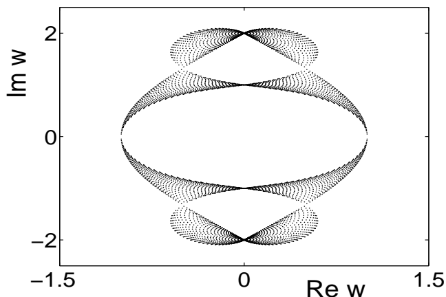
Figure 4: The partition function zeroes in the complex w = 2 \sinh(2\beta) plane for the anisotropic ( J_2 = 2J_1 ) L = M = 2N = 40 Ising model with Brascamp-Kunz boundary conditions.
