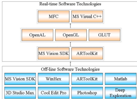
Figure 2: Software technologies
