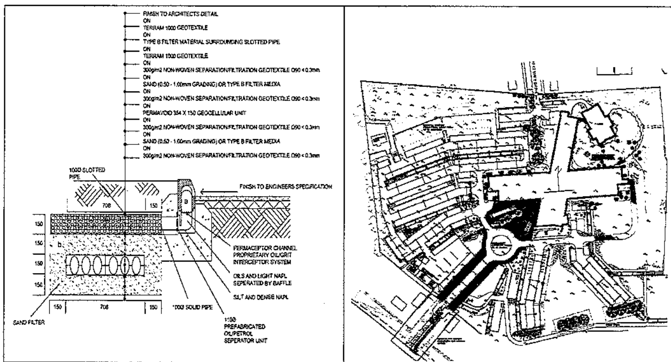
Figure 8: Permakerb & Infiltrating sandfilter
