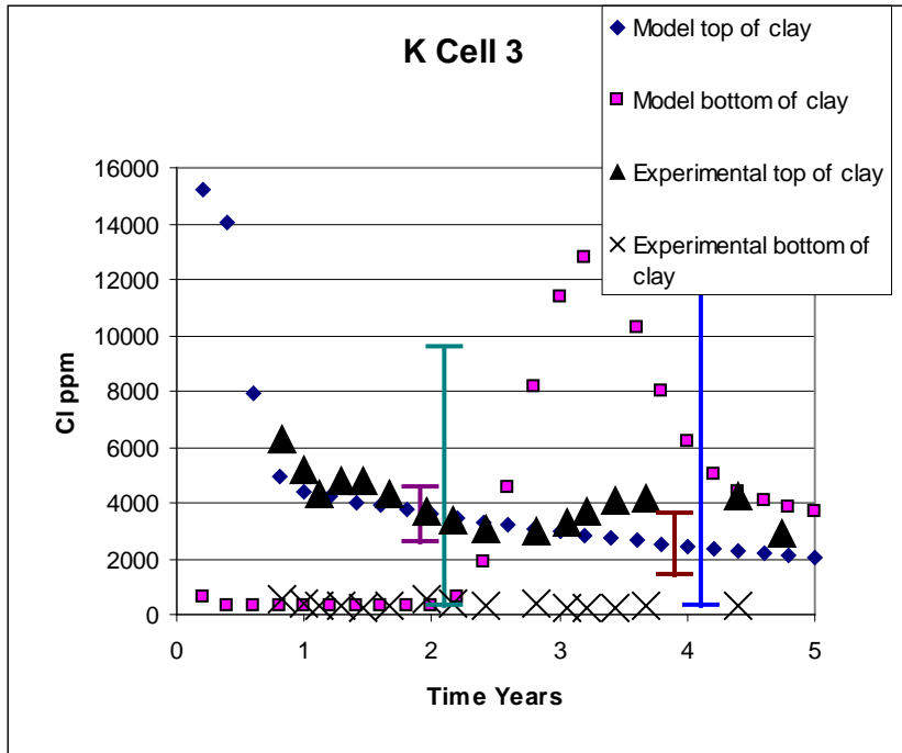
Figure 15. Concentrations of potassium in site trial cell 3
