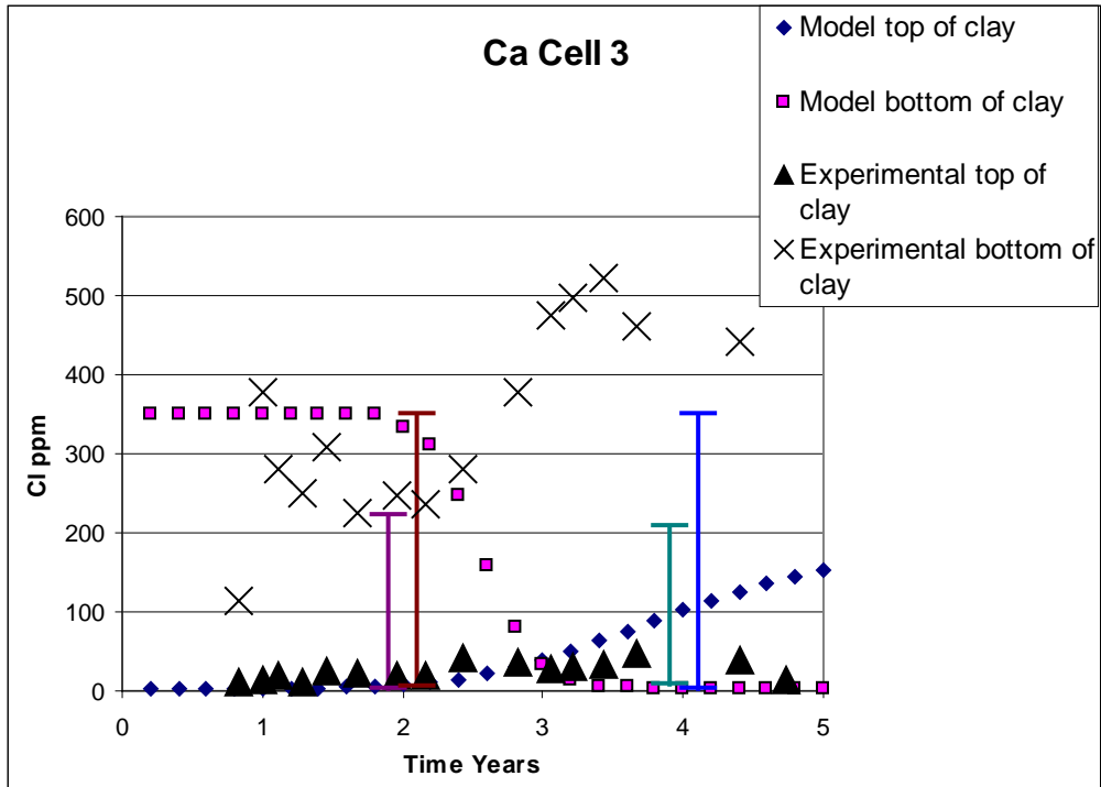
Figure 13. Concentrations of calcium in site trial cell 3
