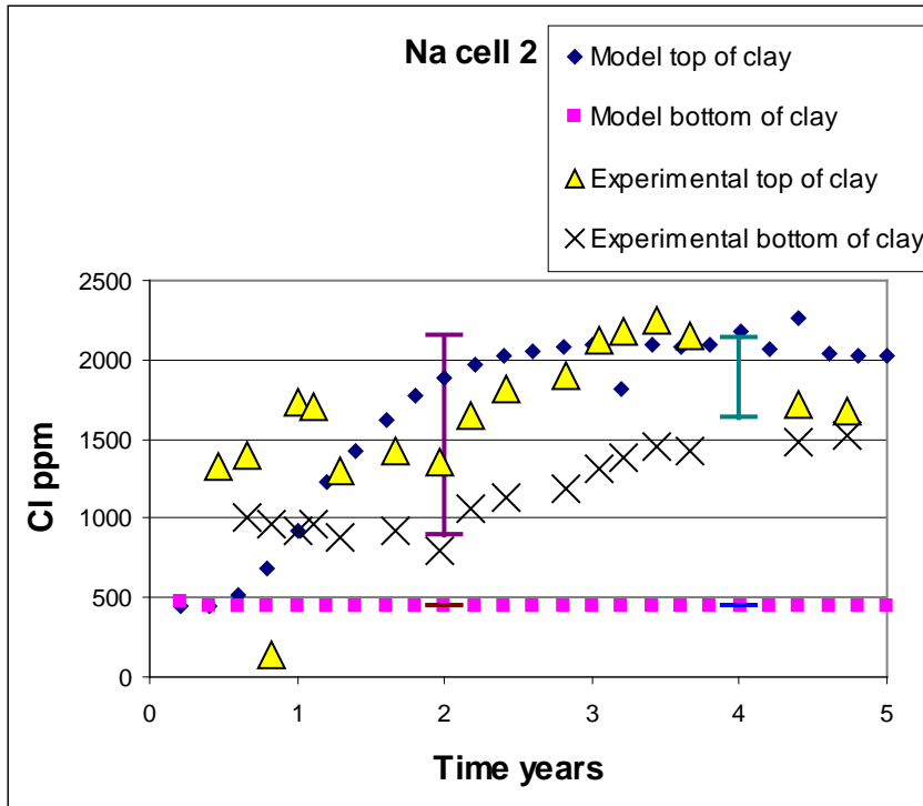
Figure 11. Concentrations of sodium in site trial cell 2
