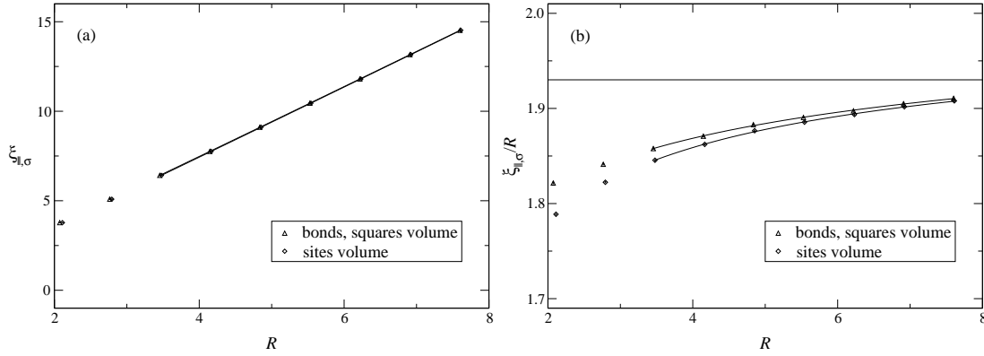
Fig. 1. – (a) FSS plot for the spin-spin correlation length \xi_{||,\sigma}(R) . (b) Scaling of the amplitudes \xi_{||,\sigma}/R . The continuous lines show fits described in the text and the horizontal line indicates the conjectured amplitude A_{\sigma}^{\text{conj}} = 1.9298(13) .
