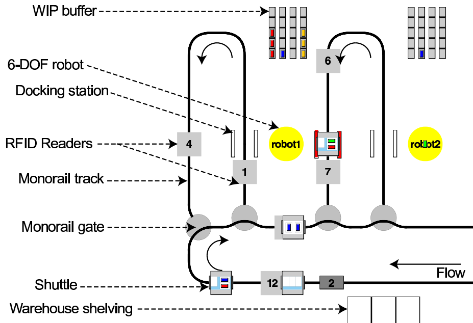
Fig. 7. Plan (schematic) view of part of the gift-box packing system.
