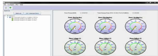
Fig.6 User Interface
