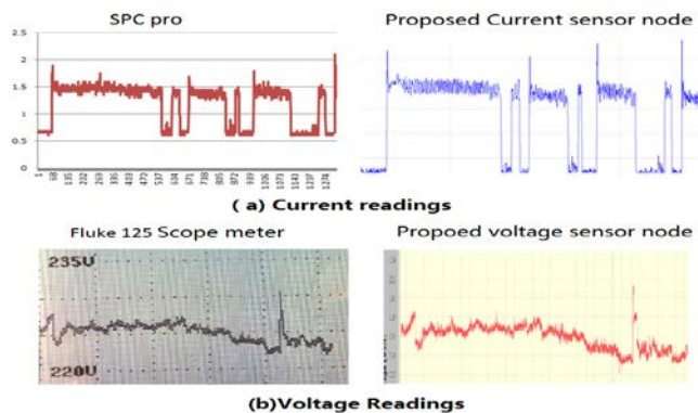
Fig.8 The comparison results of current and voltage measurement
