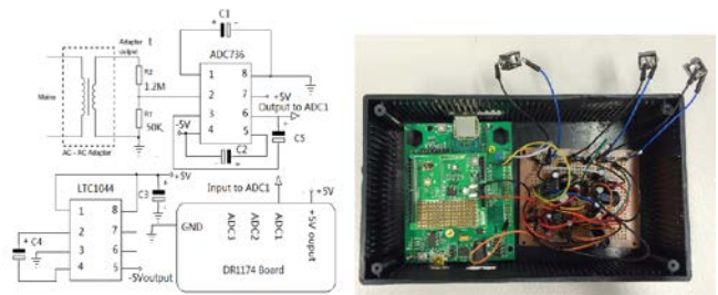
Fig.5 Schematic and hardware design of voltage sensor node
