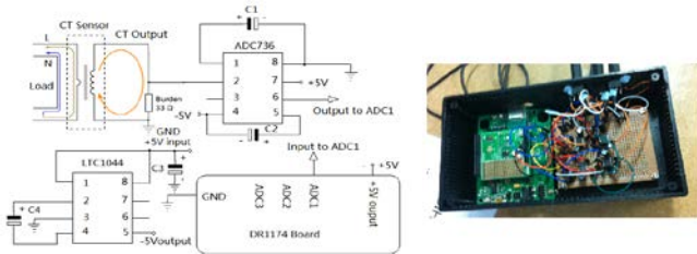
Fig.4 Schematic and hardware design of current sensor node
