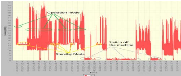
Fig.10 Power pattern
