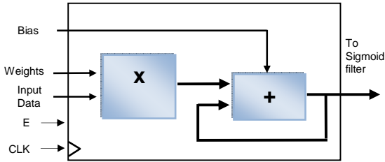
Fig. 5. Schematic of the linear part of a hidden/output neuron (sum of products, SOP module).
