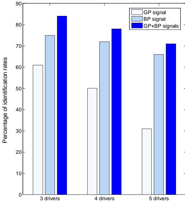
Fig. 2. Comparison of driver identification rates obtained with driving behavior signals (GP: gas pedal pressure, and BP: brake pedal pressure) using the developed model for different number of drivers.
