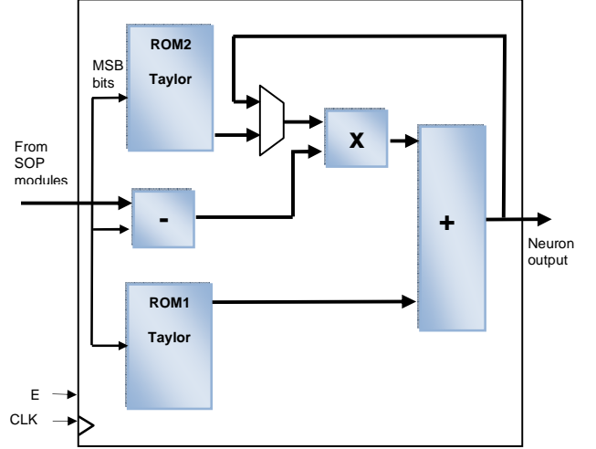
Fig. 6. Schematic of the Sigmoid circuit. It is based on a second order Taylor approximation of the function.
