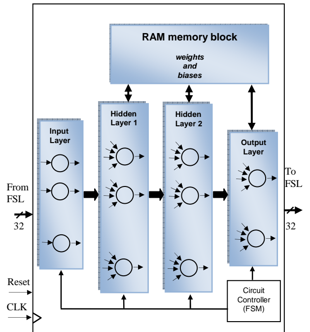
Fig. 4. Internal architecture of the neural classifier.
