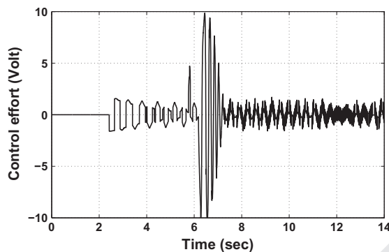
Fig. 13. Experimental results (swing-up and stabilization): control input.
