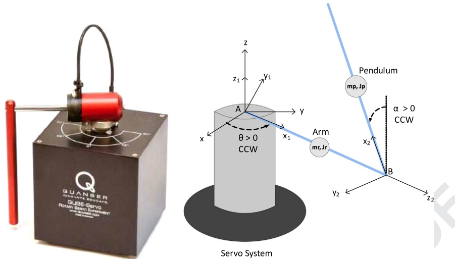
Fig. 6. Quanser QUBE-Servo inverted pendulum system [27].
