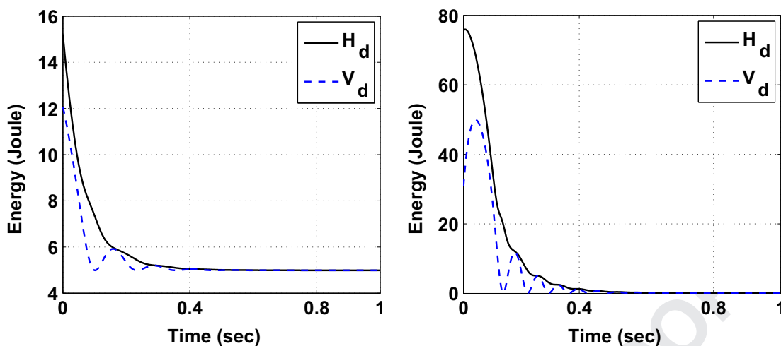
Fig. 7. The total energy of the rotary inverted pendulum. Left: q_{10} = 45^\circ . Right: q_{10} = 180^\circ .
