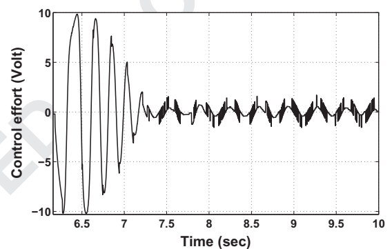
Fig. 15. Experimental results (stabilization): control input.
