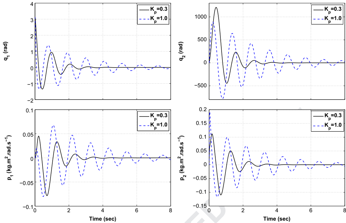
Fig. 2. Trajectories of the IWP for different values of K_p .
