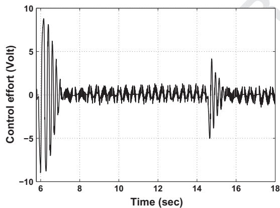
Fig. 17. Experimental results (robustness): control input.
