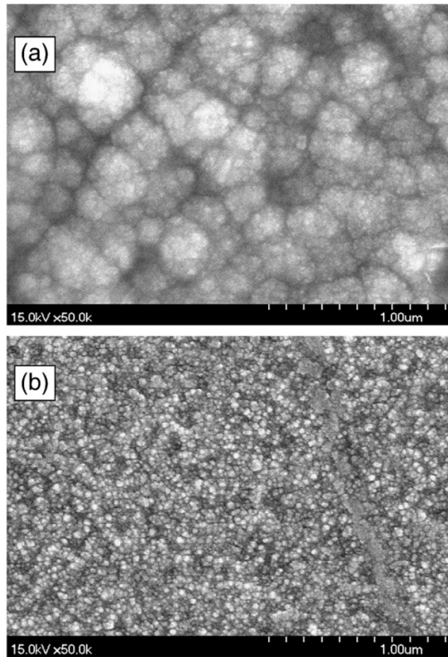
Figure 5. Surface morphologies of Ni/SiC composite films prepared under different conditions: (a) mechanical dispersion and (b) mechanical and ultrasonic dispersion. Adapted from Ref. [47], with permission from Elsevier.
