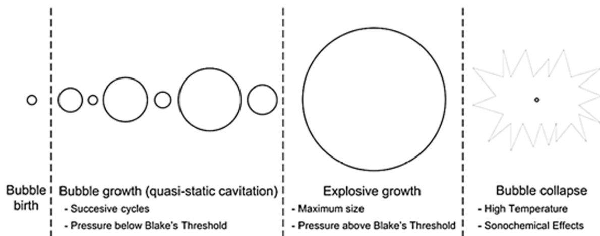
Figure 1. Bubble growth and implosion in a liquid irradiated with ultrasound. Adapted from Ref. and [7], with permission from the Multidisciplinary Digital Publishing Institute.
