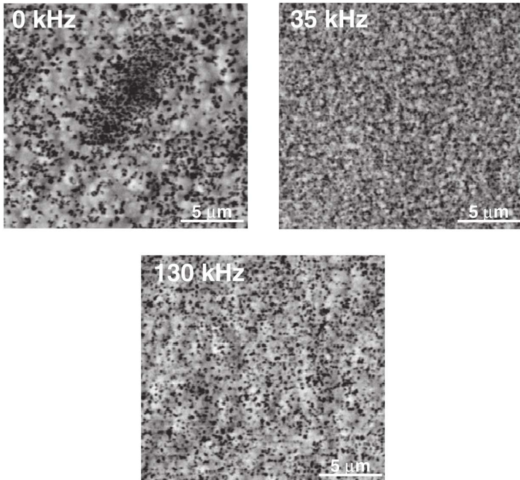
Figure 7. SEM (BSE) images of surface morphology of Ni-W/Al 2 O 3 composite coatings electrodeposited at a rotating speed of 340 rpm under different ultrasonic frequencies. Adapted from Ref. [58], with permission from Elsevier.
