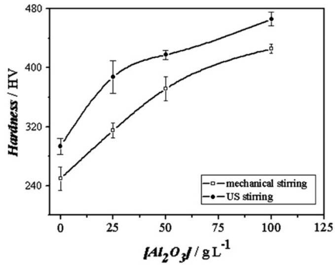
Figure 6. Effect of Al_2O_3 concentration in the electrolyte on the hardness of Ni/ Al_2O_3 composite coating obtained under mechanical stirring and ultrasound. Adapted from Ref. [38], with permission from Elsevier.
