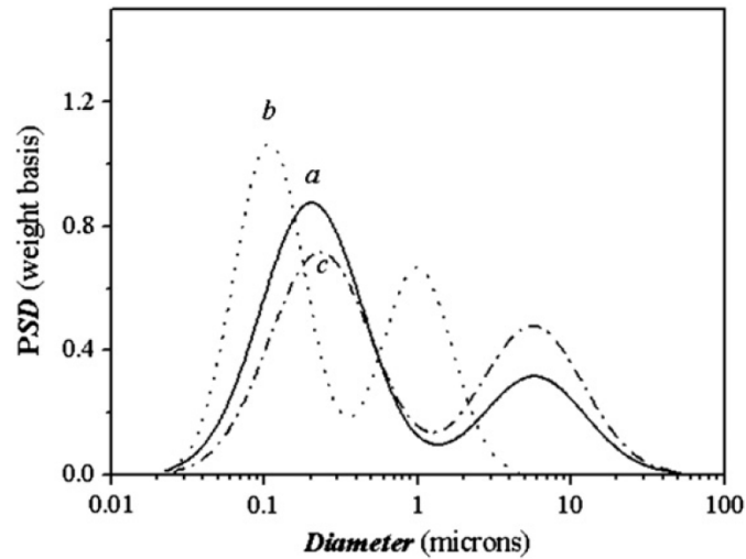
Figure 3. Particle size distribution of \text{Al}_2\text{O}_3 particles ( 50 \text{ g L}^{-1} ) dispersed in a Ni Watts bath. The experiments were carried out (a) after 24 h of magnetic stirring; (b) after 24 h of magnetic stirring+10 min of US treatment; (c) same as b after one hour. Adapted from Ref. [38], with permission from Elsevier.
