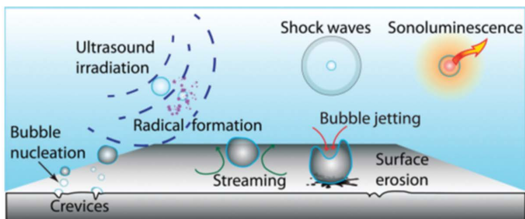
Figure 2. Schematic representation of the main effects of cavitation induced by ultrasound irradiation. Adapted from Ref. [9], with permission of The Royal Society of Chemistry.
