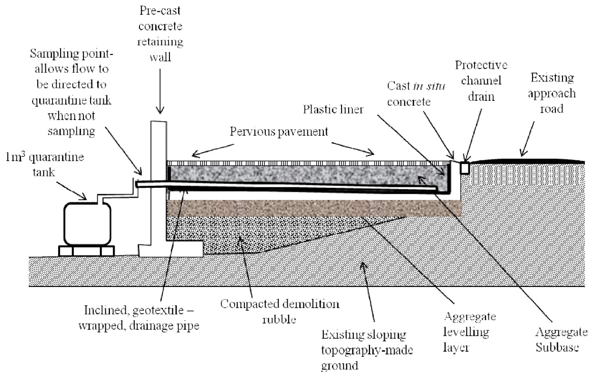
Figure 1 Schematic cross section of test rig (not to scale).
