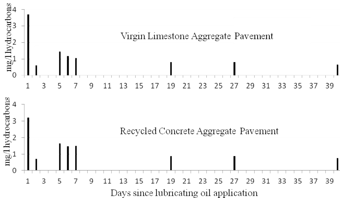
Figure 4: Mean daily concentrations days L1-L40 n=20 day L1, n=8 day L2, n=4 days L5-L27, n=11 day L40
