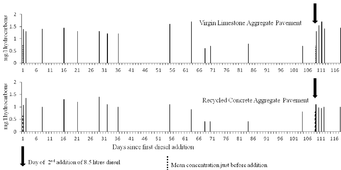
Figure 5: Mean daily oil concentration mg/l days from 1st diesel addition (days D1-D119)
