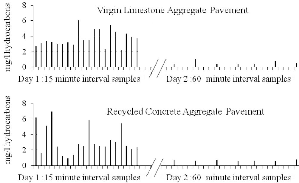
Figure 3: Hydrocarbon concentrations in effluent. First 2 days after of lubricating oil addition (nominal time series over 28 hours days L1 & L2).
