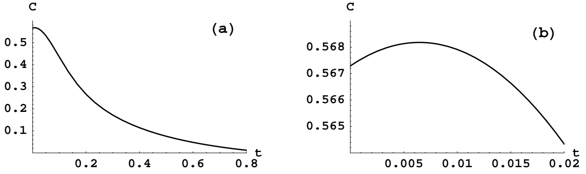
Figure 2: (a) The behavior of the specific heat on \mathcal{M} \times \mathcal{N} lattices with even \mathcal{M} = 16 and odd \mathcal{N} = 17 . (b) The behavior of the specific heat on the same lattice for small t .
