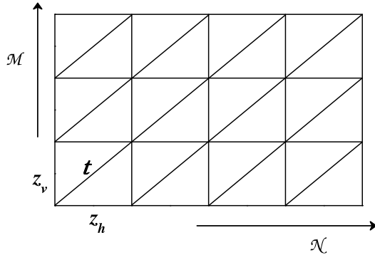
Figure 1: The \mathcal{M} \times \mathcal{N} triangular lattice with dimer weights z_h in the horizontal direction, z_v in the vertical direction, and t in the diagonal direction.
