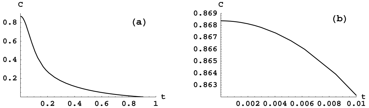
Figure 4: (a) The behavior of the specific heat on M \times N lattices with even M = 16 and N = 16 . (b) The behavior of the specific heat on the same lattice for small t .
