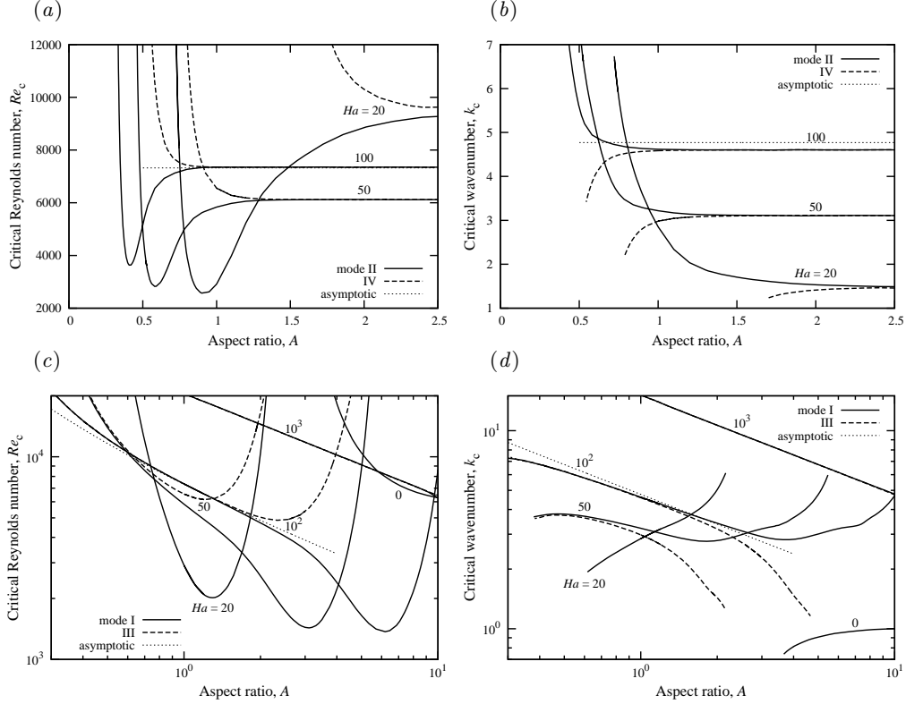
FIGURE 9. The critical Reynolds number (a,c) and the wavenumber (b,d) versus the aspect ratio for modes II/IV in a horizontal magnetic field (a,b) and for modes I/III in a vertical magnetic field (c,d) at various Hartmann numbers.
