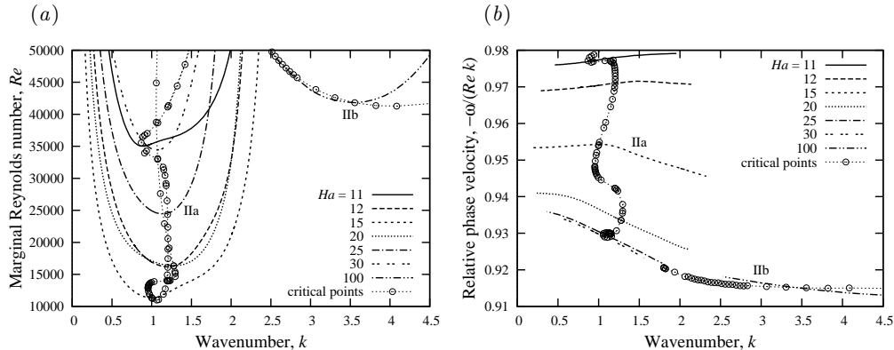
FIGURE 4. The marginal Reynolds number (a) and the relative phase velocity (b) versus the wavenumber for neutrally stable modes of type II in a square duct ( A = 1 ) subject to a vertical magnetic field at various Hartmann numbers.
