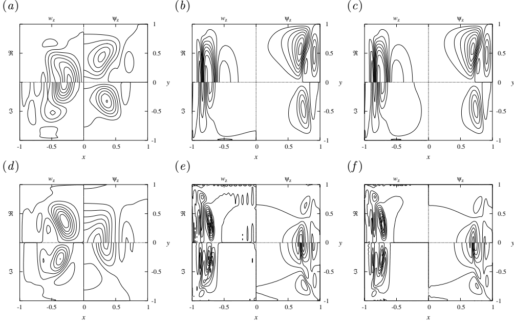
FIGURE 7. Amplitude distributions of the real ( y > 0 ) and imaginary ( y < 0 ) parts of \hat{w} ( x < 0 ) and \hat{\psi}_z ( x > 0 ) of the critical perturbations over one quadrant of duct cross-section for instability modes I (a,b), IIa (d,e), III(c) and IV(f) at Ha = 15 (a,d) and Ha = 100 (b,c,e,f).
