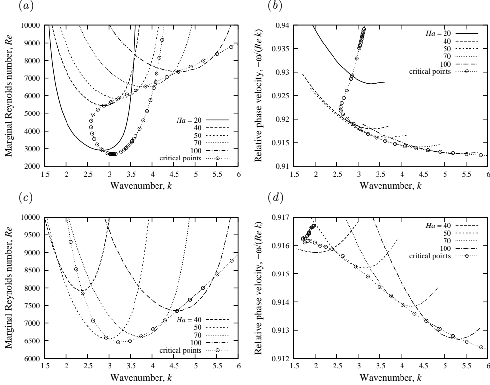
FIGURE 5. The marginal Reynolds number (a,c) and the relative phase velocity (b,d) versus the wavenumber for neutrally stable modes of type I (a,b) and type III (c,d).
