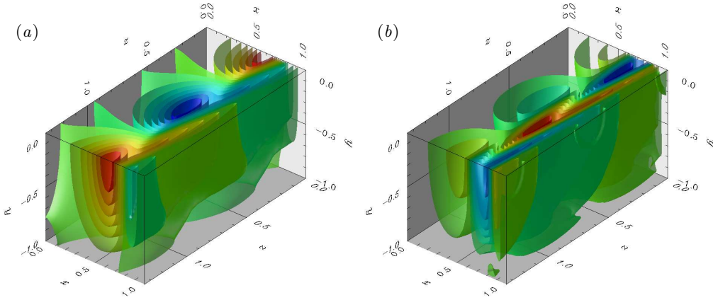
FIGURE 8. Isosurfaces of \hat{\psi}_y (a) and longitudinal velocity \hat{w} (b) perturbations over wavelength in one quadrant of the duct cross-section for instability mode I at Ha = 100 in a vertical magnetic field.
