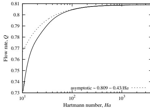
FIGURE 3. Numerically calculated flow rate in one quarter of a square duct ( A = 1 ) against the Hartmann number.
