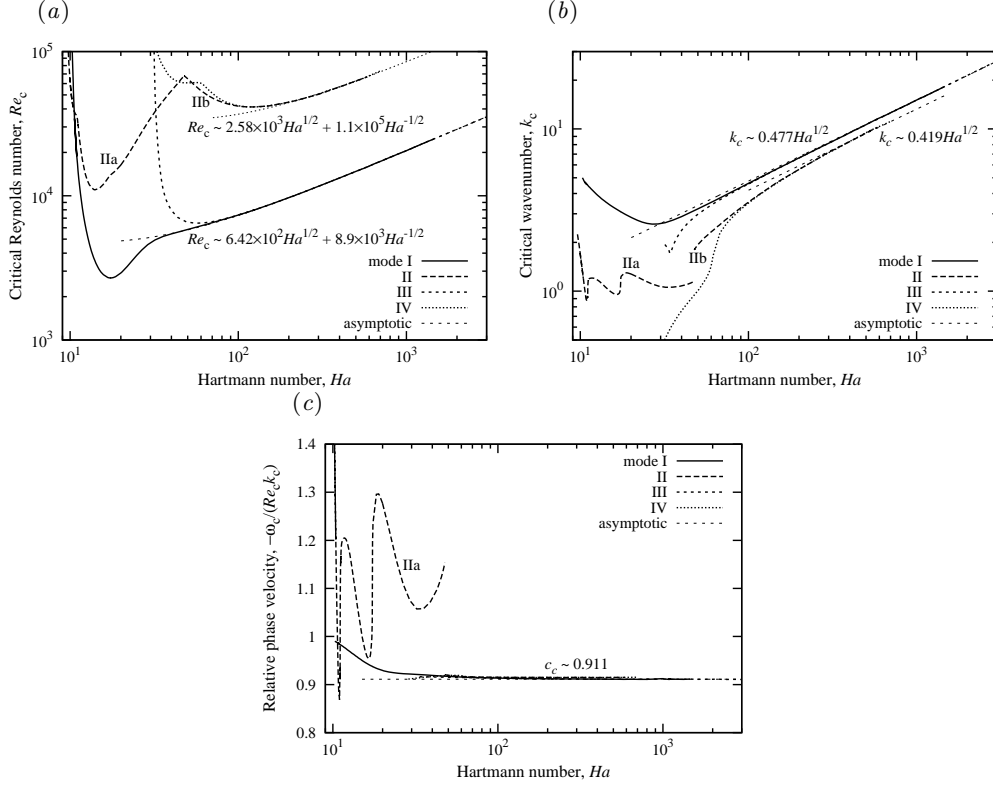
FIGURE 6. The critical Reynolds number (a), wavenumber (b) and relative phase velocity (c) against the Hartmann number.
