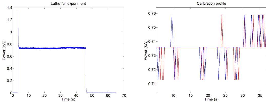
Fig 6. a) Measure of the power used by the lathe in the whole experiment. b) Comparison of the measures of power consumption of the lathe by the SPC data logger (red line) and the pcDuino (blue line).
