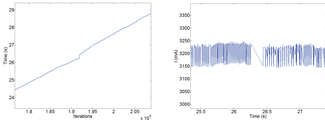
Fig 5. a) Abnormal time conversion b) Absence of data collection during data dump
