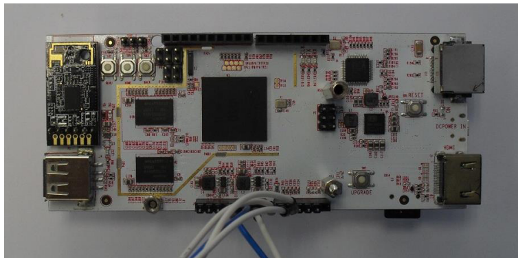
Fig 2. Single board PC used for in the smart sensor: pcDuino V2.
