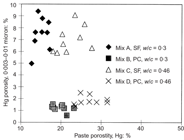
Fig. 6. Mercury intrusion porosity in the 0.003–0.01 \mu\text{m} pore size range vs total mercury intrusion porosity
