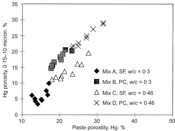
Fig. 5. Mercury intrusion porosity in the 0.01–0.15 \mu\text{m} pore size range vs total mercury intrusion porosity
