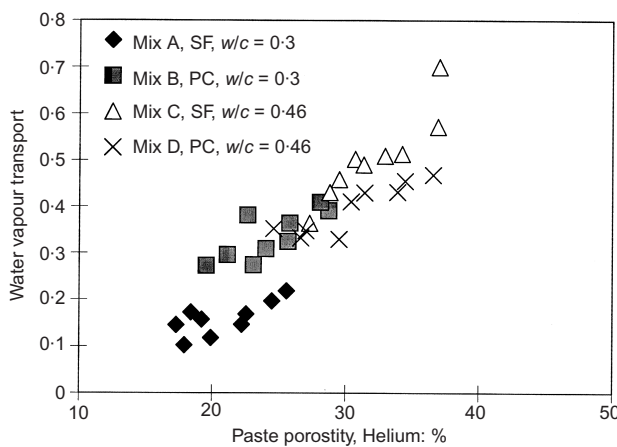
Fig. 13. Water vapour transport (relative units) vs. helium intrusion porosity
