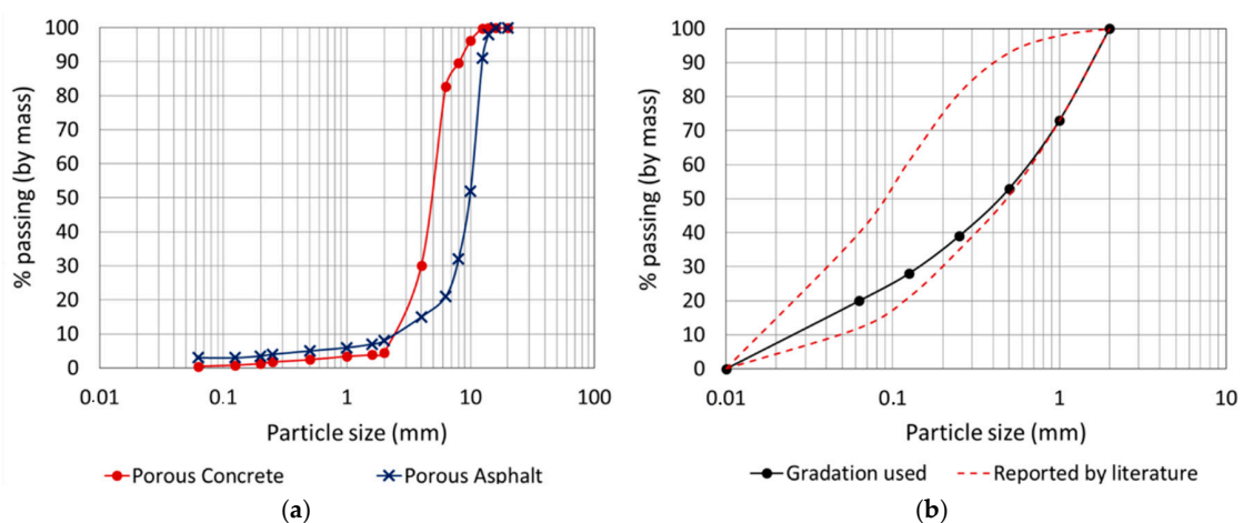
Figure 1. (a) Gradation of aggregates used in porous concrete (PC) and porous asphalt (PA) mixtures; and (b) Gradation of clogging sediments used and range of particle sizes reported by the literature [30–33].
