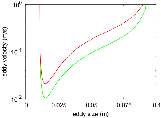
Figure 7: The minimum amplitude of a turbulent eddy as a function of eddy size predicted by Batchelor that will lead to breakup of a Taylor bubble rising through water in a 0.29m tube. The two lines correspond to two different stability criterion; A_{\lambda=R} = 0.082R (red) and A_{\lambda=R} = 0.041R (green). Both criterion give a minimum critical amplitude for disturbances of initial length scale 0.0152m but with amplitudes of 0.0211m/s for the former and 0.0106m/s for the latter.
