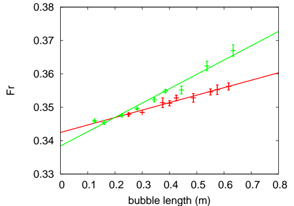
Figure 2: The nondimensionalised rise rates ( Fr ) of bubbles in the 0.29m (red) and 0.121m (green) pipe and their dependence on bubble length. The variation in Fr is due to the bubbles expanding as they rise. Consequently extrapolation to a bubble of zero length gives the rise rate of bubble not undergoing expansion – Fr = 0.342 in the case of the larger pipe and Fr = 0.338 in the case of the narrower one. The different gradients for the two pipes are due to the effect of H on \dot{L} (Equation 3). Error bars represent one standard error.
