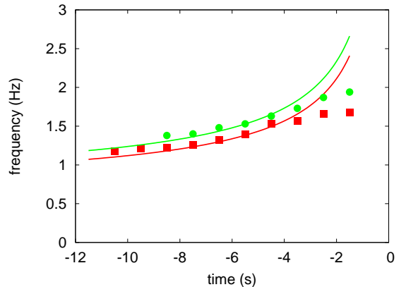
Figure 6: The evolving frequency of oscillating bubbles as they rise up the pipe for two different mean lengths of bubble (red is 0.55m , green is 0.45m ). The points represent experimental data taken from ten runs in the case of the longer bubble and six in the case of the shorter bubble. The lines come from the theoretical model given by equation 14, where the polytropic exponent has been taken to be 1. Time is measure from the bubble bursting at the surface. The model fits well until the bubble approaches the surface.
