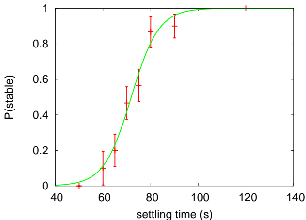
Figure 4: The probability of a Taylor bubble breaking up within a 2m observation window in the 0.290m pipe. The settling time is defined by the delay between the last of the gas from the previous bubble departing the window to the tip of the bubble being considered entering the window. Error bars are found by assuming a binomial distribution to the data's repeated runs and represent one standard deviation. The green line is included to guide the eye.
