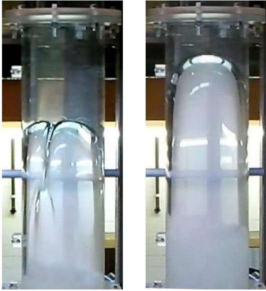
Figure 3: Two Taylor bubbles rising through the 0.29m column. The one on the left is undergoing breakup, while the right-hand bubble is stable.
