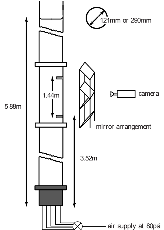
Figure 1: Diagram of experimental apparatus. Gas is injected at the bottom of the column. Velocity measurements are taken using a system of mirrors in conjunction with a high speed camera.
