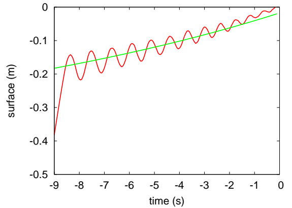
Figure 5: The evolution of the height of the water's surface from the time the surface enters the shot of the highspeed camera until the bubble bursts it at t = 0 and h = 0 . The red line is taken from the rise of a bubble initially 0.55m long. The mean rise of the surface is due to the bubble expanding as it decompresses during the rise. This is captured by the green line which has been calculated by assuming the bubble expands as a perfect gas obeying pV = const. Time is measured from when the bubble will burst at the surface.
