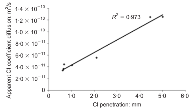
Figure 12. Correlation between the calculated Cl apparent diffusion coefficient and the Cl penetration measured during the test
