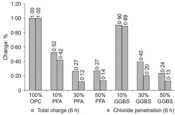
Figure 4. Total charge and chloride penetration (60 V)
