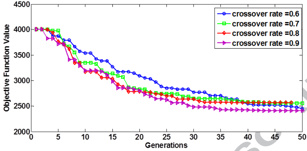
Figure 11: Performance comparison of different crossover rates for an example under Pop = 100 and P_m = 0.02
