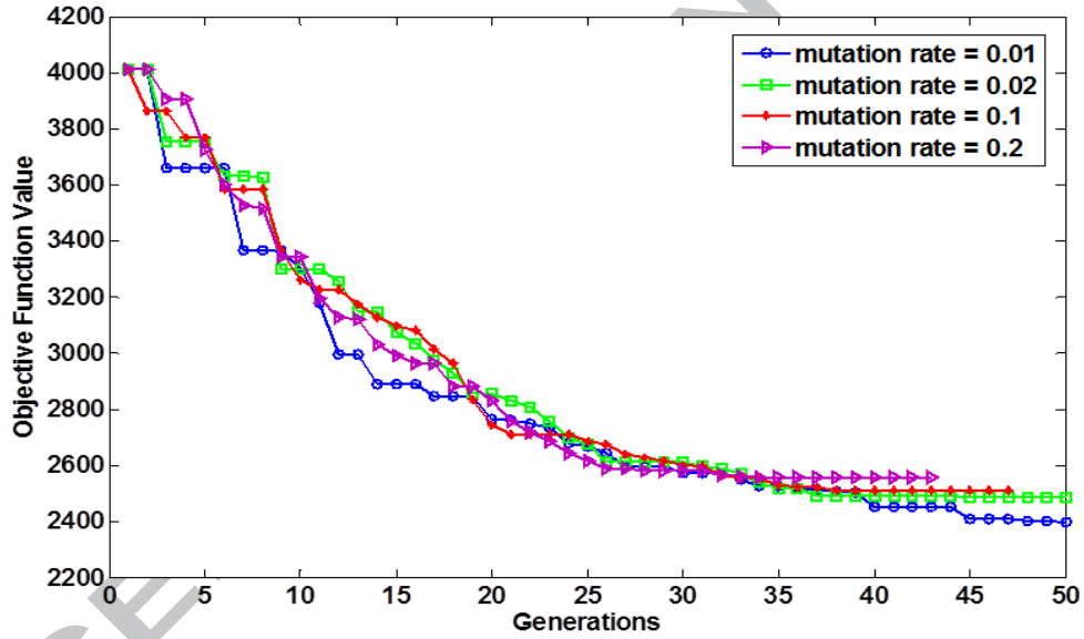
Figure 12: Performance comparison of different mutation rates for an example under Pop = 100 and P_c = 0.9
