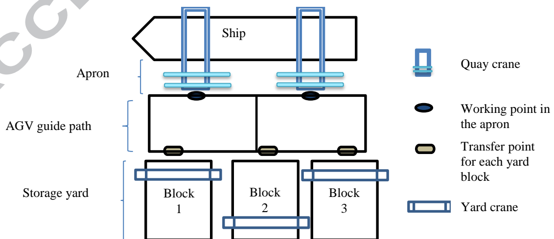
Figure 3: The layout of an automated container terminal
