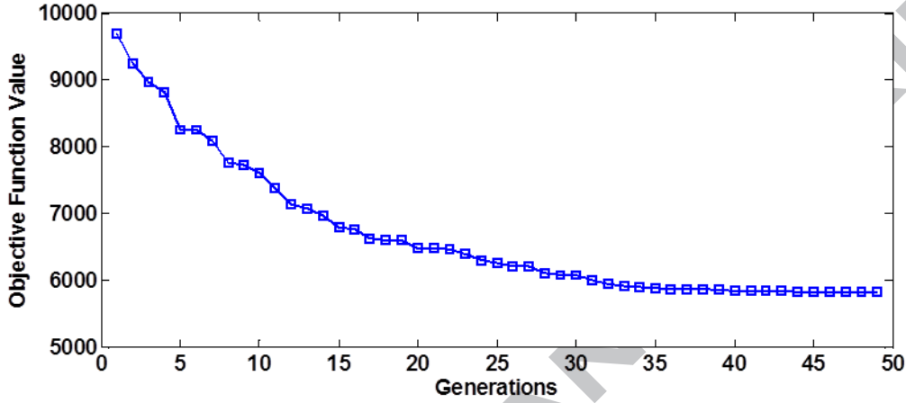
Figure 10: Typical convergence of GA for the case with 100 containers, five AGVs, three QCs and four YCs
