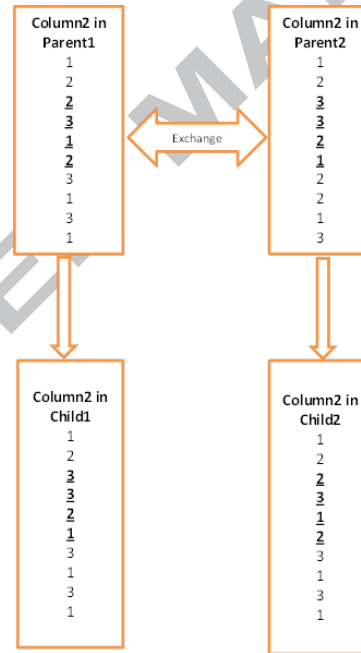
Figure 7: An illustration of two-point crossover for an example of 10 containers
