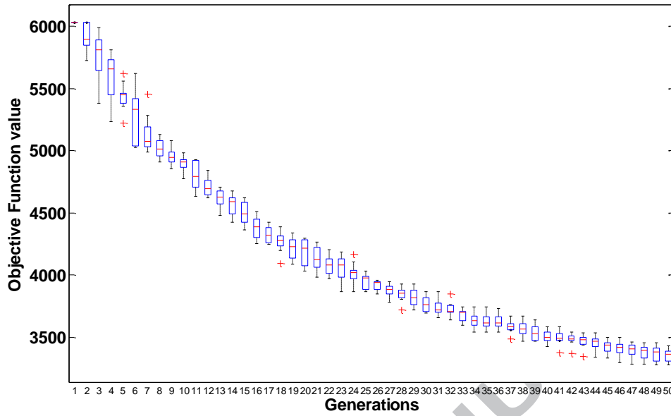
Figure 14: GA performance in 10 runs with P_c = 0.9 , P_m = 0.01 and Pop = 100 for the case with 60 containers, five AGVs, three QCs and four YCs
