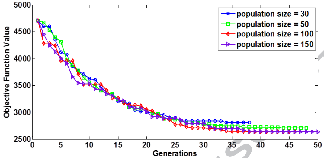
Figure 13: Performance comparison of different population size for an example under P_c = 0.9 and P_m = 0.01 .
