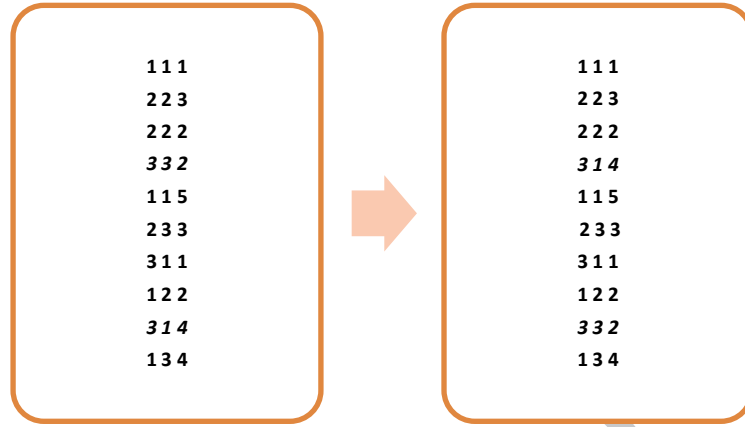
Figure 9: An illustration of swap mutation for an example of 10 containers
