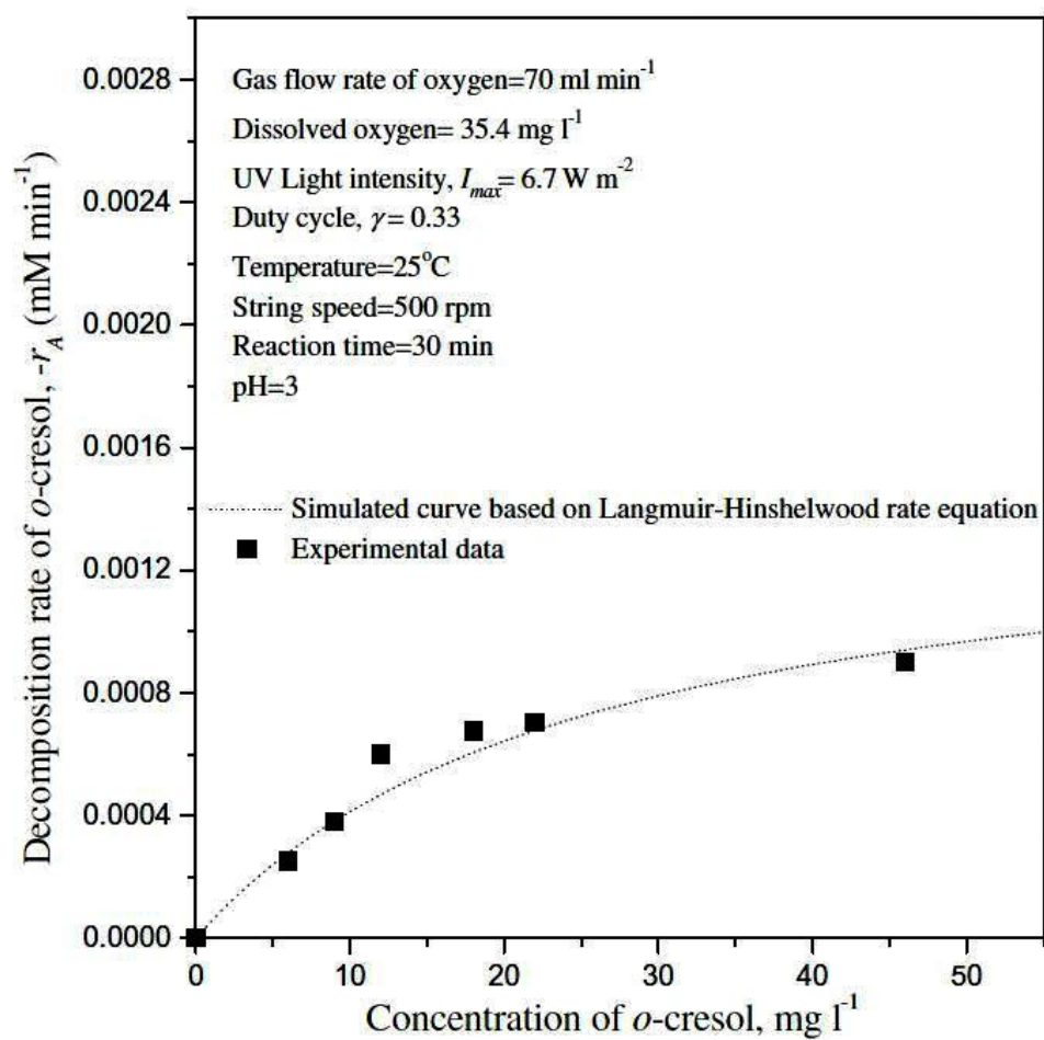
Figure 6: Rate comparison between experimental data and L-H CPI model by Chen et al. [Reprinted with permission from [56]. Copyright 2007, Elsevier].
