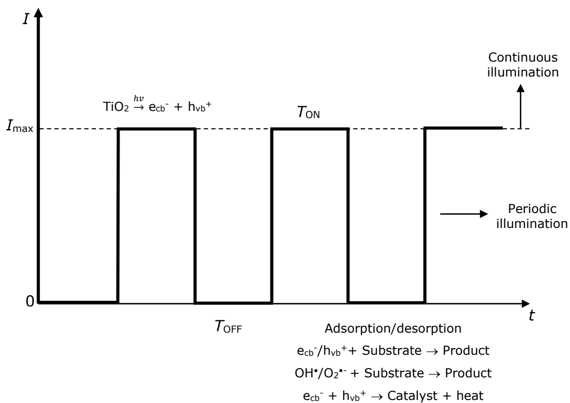
Figure 2: Schematic of CPI according to the original hypothesis by Sczechowski and co-workers.
