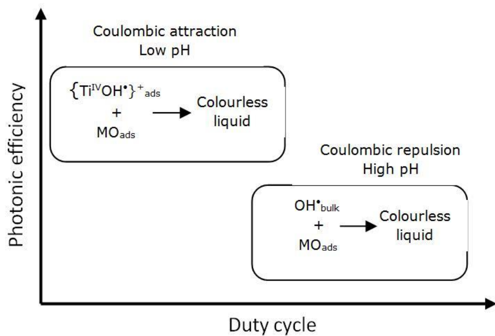
Figure 8: Photonic efficiency regimes due to the triple effect of pH, \gamma and oxidizing species.
