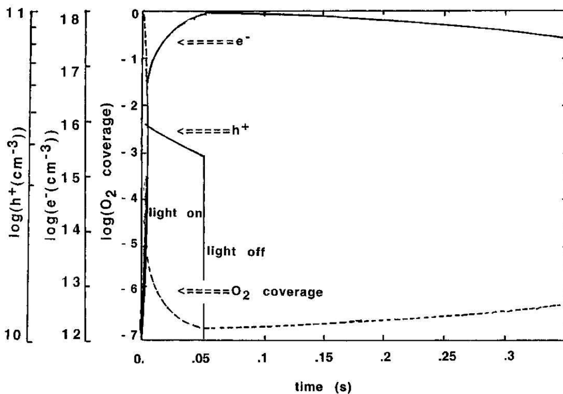
Figure 5: Calculation of dioxygen and net charge concentration as a function of time by Upadhyaya and Ollis. [Reprinted with permission from [59]. Copyright 1997, American Chemical Society].
