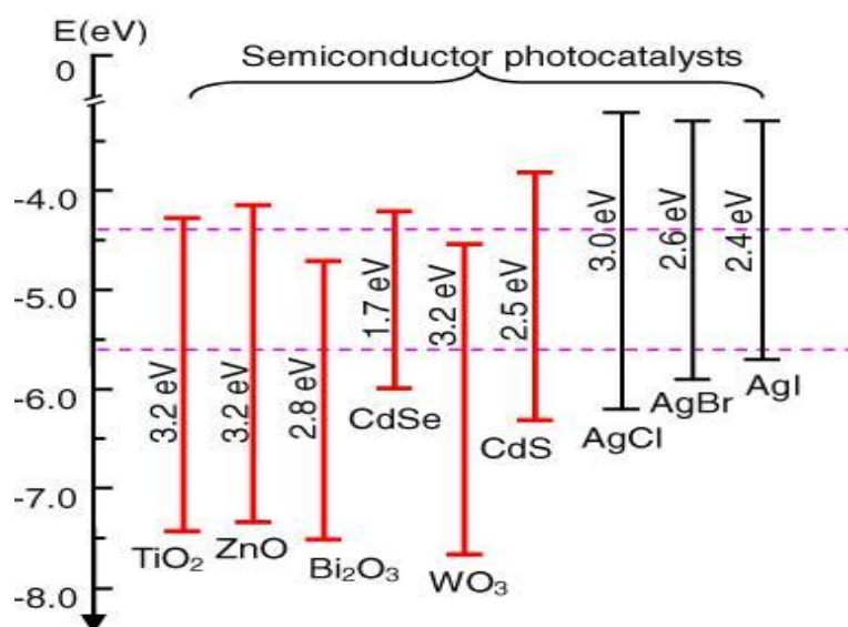
Figure 1: (a) Energy bands in solids: (a) insulator, (b) semiconductor, (c) conductor; (b) band gaps of common semiconductor photocatalysts [Reprinted with permission from [69]. Copyright 2013, IOP publishing].
