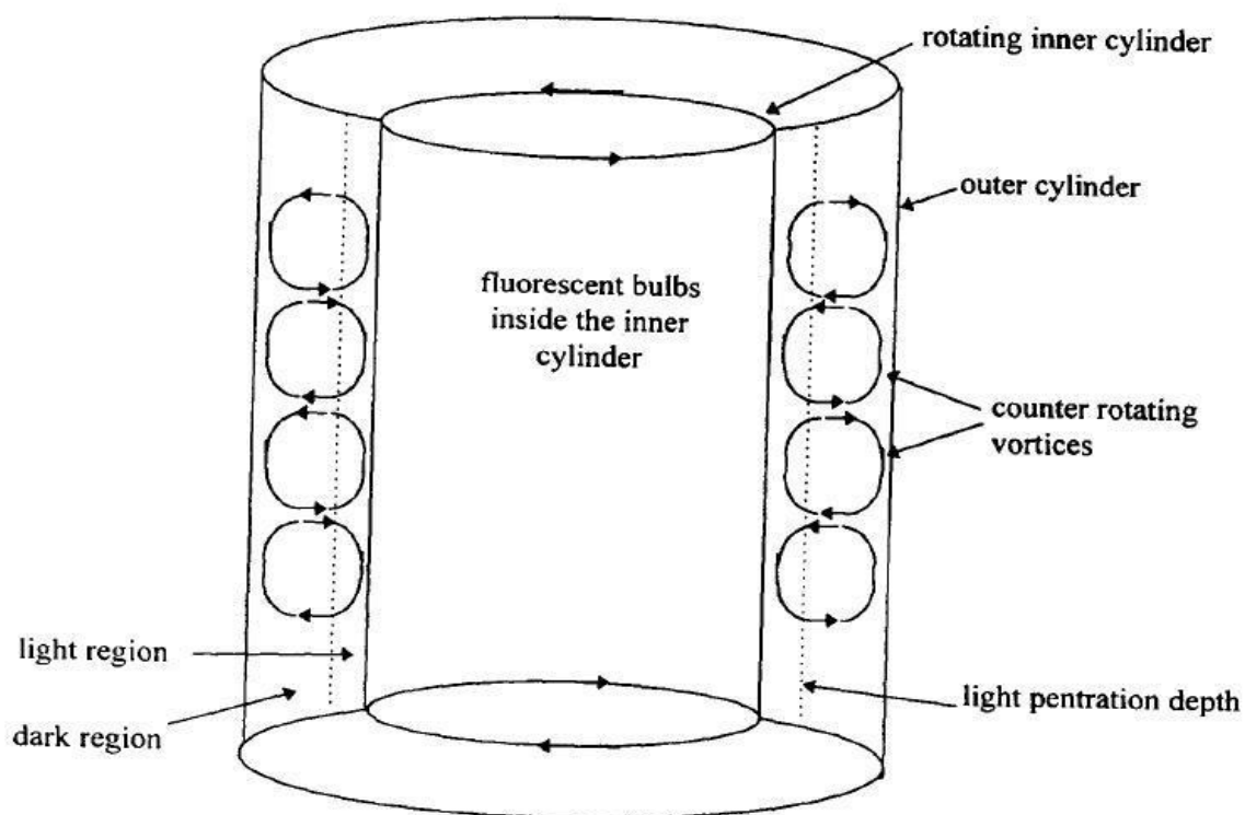
Figure 3: A section through a TVR during operation [Reprinted with permission from [46]. Copyright 1995, Elsevier].
