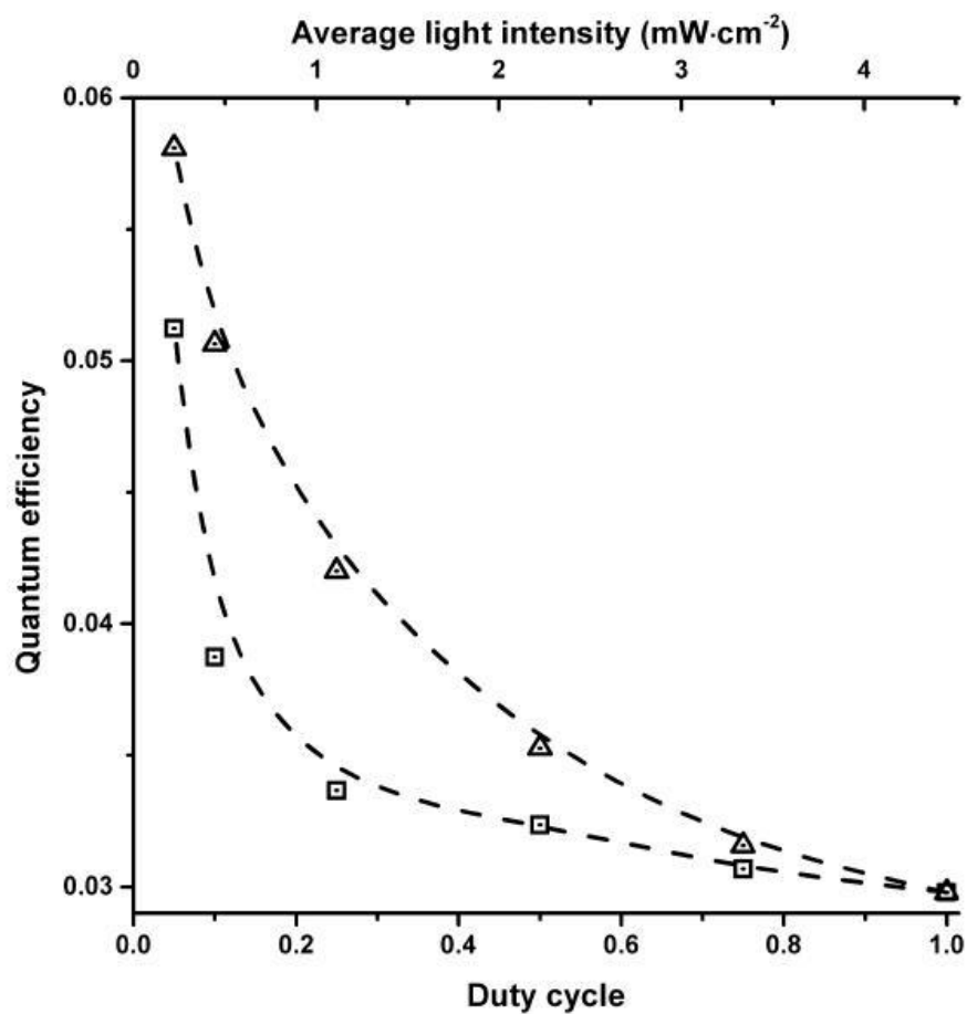
Figure 9: Comparison between photonic efficiencies under CPI (box) and continuous illumination (triangle) at equivalent average light intensities by Korovin et al.
