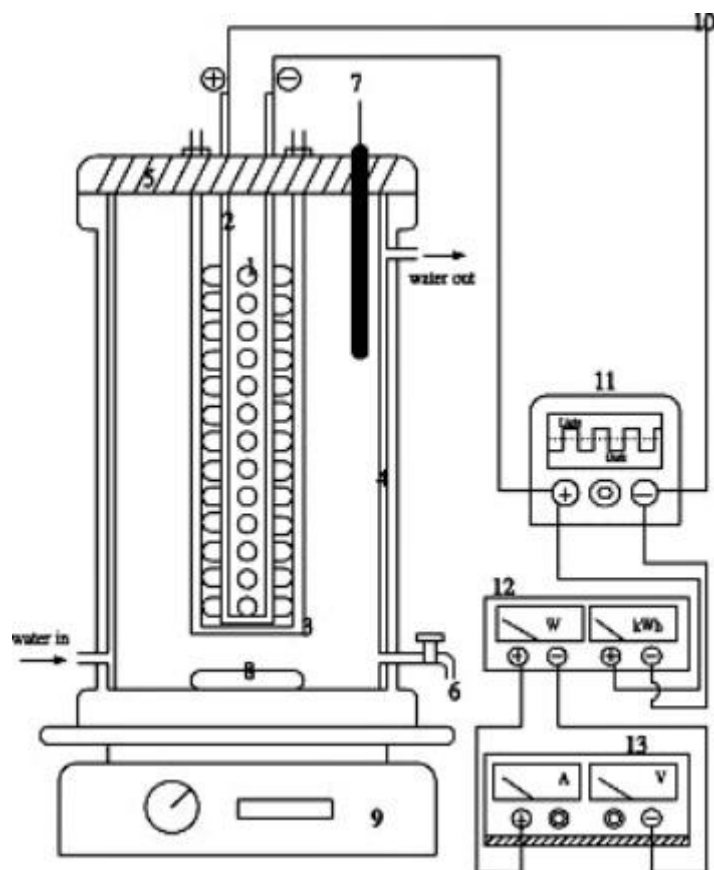
Figure 4: UV LED illuminated photoreactor designed by Chen et al. [Reprinted with permission from [56]. Copyright 2007, Elsevier].
