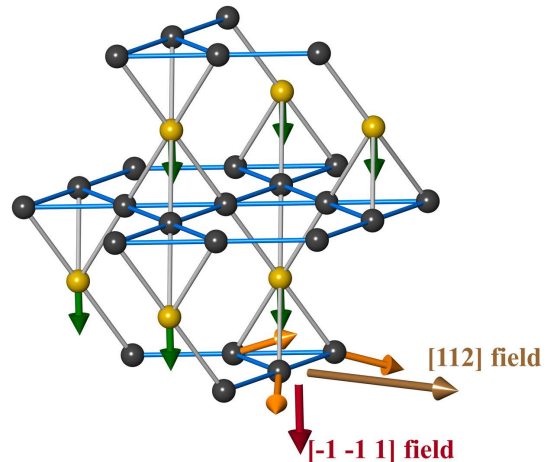
FIG. 2. Schematic illustration of the [112] field magnetization measurement with the structure of the pyrochlore lattice viewed as alternating triangular and kagome planes. An applied field in the [112] direction is shown as a brown arrow. An applied field along [\bar{1}\bar{1}1] is shown in red. This field points along the local Ising axis of the green spin vectors on the triangular planes (yellow sites).
