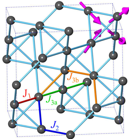
FIG. 1. Set of interacting neighbors on the pyrochlore lattice. The first ( J_1 ), second ( J_2 ) and two distinct third ( J_{3a} and J_{3b} ) nearest-neighbor pathways are indicated by red, blue, green and orange connections, respectively, on the pyrochlore lattice of corner-sharing tetrahedra. A two-in/two-out state of two spins pointing into the center of the tetrahedron and two spins pointing out from the tetrahedron is shown in the upper right hand corner of the lattice. An ice-rule obeying state is characterized by all tetrahedra being in a two-in/two-out spin configuration, but with no other constraint on the orientation of the spins.
