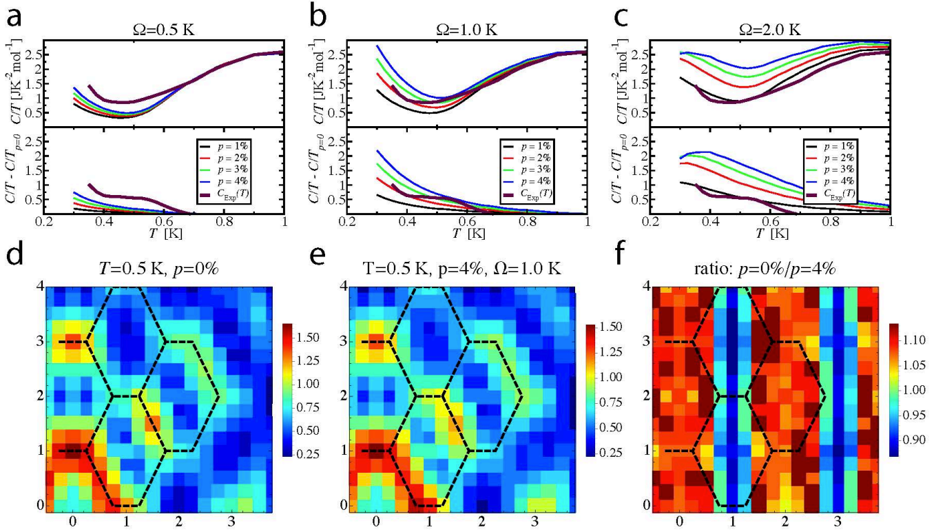
FIG. 10. Effects of impurities on specific heat and neutron scattering. Specific heat, C(T)/T for the \Omega -model with a \Omega = 0.5 K, b \Omega = 1.0 K and c \Omega = 2.0 K with the percentage of stuffed spins p=1,2,3 , and 4%. The upper panel shows the total specific heat, while in the lower panel the specific heat of the clean system ( p = 0 ) has been subtracted from the disorder average of the upper panel revealing the impurity contribution. The neutron structure factor S(\mathbf{q}) for the disorder-free ( p = 0 ) g-DSM model 36 at T = 0.5 K is shown in d , and with p = 4\% stuffed spins included in e . The last panel, f , shows the ratio of the structure factor for the clean ( d ) and stuffed ( e ) systems.
