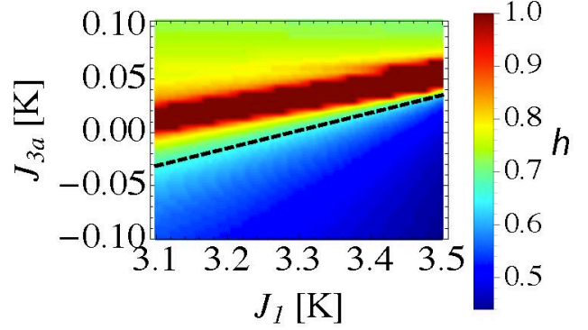
FIG. 12. Mean-field ordering wave vector. Map of the mean-field ordering wave vector, \mathbf{q} , in the constrained J_1 - J_{3a} parameter space, where the system selects a wave vector along the (hk0) direction. The broad red band across the middle indicates the single-chain phase with \mathbf{q} = (1\ 1\ 0) . In the lower part of the figure the order is close to the double-chain ordering wave vector \mathbf{q} = (\frac{1}{2}\ \frac{1}{2}\ 0) . The phase boundary according to Eq. 6 is shown as a dashed black line.
