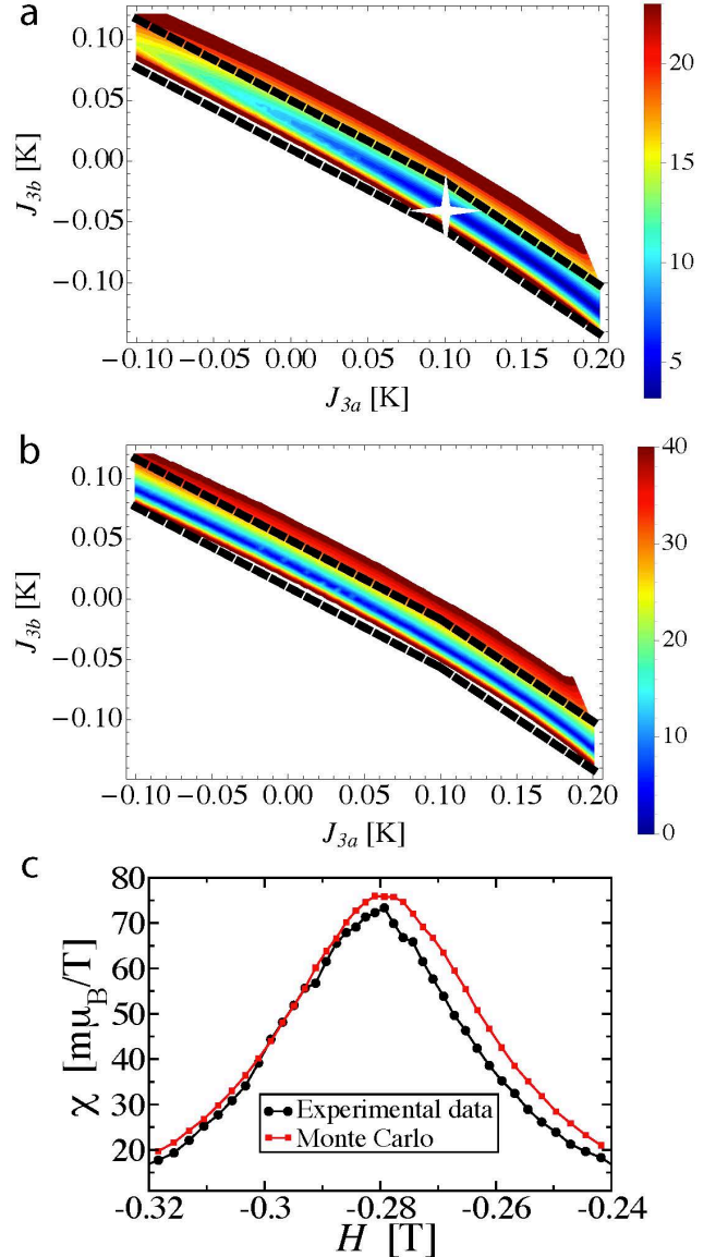
FIG. 11. Determination of the J_{3a} - J_{3b} constraining equation. Deviations of the susceptibility for the FCC sublattice (defined by the spins on triangular planes), calculated in the Monte Carlo simulations, from the experimental data 39 as a function of J_{3a} and J_{3b} . In a , the RMS deviation \sigma_\chi , calculated according to Eq. (A3), is shown, while in b the absolute value of the height difference, determined using Eq. (A4), is displayed. The dashed black lines show the parameter range used in Fig.6 of the main text, while the optimal relationship lies precisely between the two lines. In c , the susceptibility measured in the experiment and calculated in the Monte Carlo simulation at J_{3a} = 0.10 K and J_{3b} = -0.04 K (indicated by a white star in panel a ) is shown on an absolute scale as a representative example.
