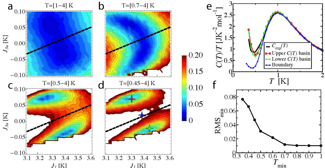
FIG. 5. Goodness of fit of Monte Carlo data compared to experimental specific heat. a-d , RMS error deviation, \sigma_C , of the dipolar spin-ice model in a constrained J_1 - J_{3a} parameter space compared to recently reported specific heat measurements 30 . The experimental specific heat data displayed in panel e are the raw data minus the calculated nuclear portion, C_{\text{exp}}(T) \equiv C_{\text{raw}}(T) - C_{\text{nuc}}(T) (see Appendix D). The label above each panel gives the temperature range of the fit. A dark blue color indicates a good fit, while white regions are off the scale. e , Specific heat divided by temperature for the experimental data (thick black line), a representative point in the upper basin (red open circles and red line), a representative point in the lower basin (filled green up triangles and green line) and a point on the boundary (filled blue squares and blue line). The corresponding J_1 - J_{3a} points are marked by correspondingly colored stars in panel d . f , The minimal RMS error in the entire J_1 - J_{3a} plane as a function of the lower limit of the temperature range of the fit, T_{\min} . Note the rapid increase in the RMS error below T \approx 0.7 K, indicating the rapid onset in the failure of the model to describe the experimental specific heat data, C_{\text{exp}}(T) .
