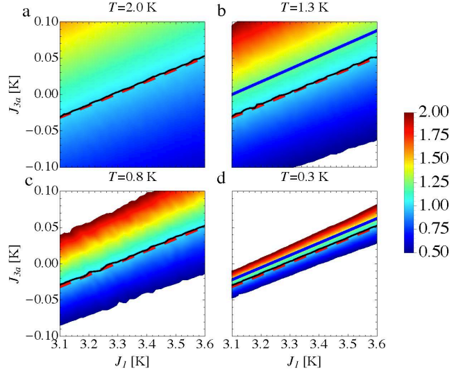
FIG. 17. Ratio of structure factor for single-chain and double-chain order. The ratio r \equiv S(0\ 0\ 3)/S(\frac{3}{2}\ \frac{3}{2}\ \frac{3}{2}) in the constrained J_1 - J_{3a} plane calculated in the Monte Carlo simulations, without the \text{Dy}^{3+} form factor. The phase boundary is marked by a dashed red line, and the r = 1 contour is indicated by a thin black line, which overlaps the phase boundary in all panels. For all temperatures, the ratio is therefore unity at the phase boundary, while it is greater than one in the single-chain region above the boundary and less than one in the double-chain region below the boundary. The blue lines in b and d indicate the ratio for the experimental neutron scattering data at T = 1.3 K and T = 0.3 K.
