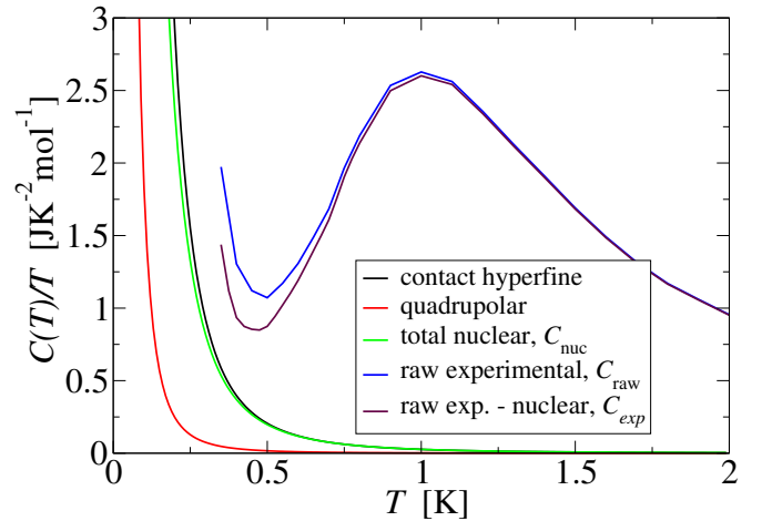
FIG. 18. Nuclear contact contribution (black curve), quadrupolar (red curve) and total, C_{\text{nuc}}/T (green curve) nuclear contribution to the specific heat. The blue curve shows the raw experimental C_{\text{raw}}/T data while the purple curves shows the residual electronic data, C_{\text{exp}}(T)/T data.
