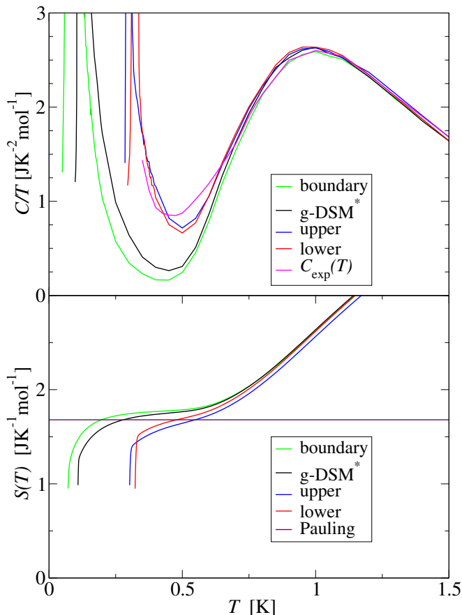
FIG. 9. The specific heat (upper panel) and corresponding entropy, S(T) , (lower panel) for the four parameter sets in Table I. The entropy value of the Pauling plateau at S=(R/2)\ln(3/2) is indicated by a brown horizontal line in the lower panel.
