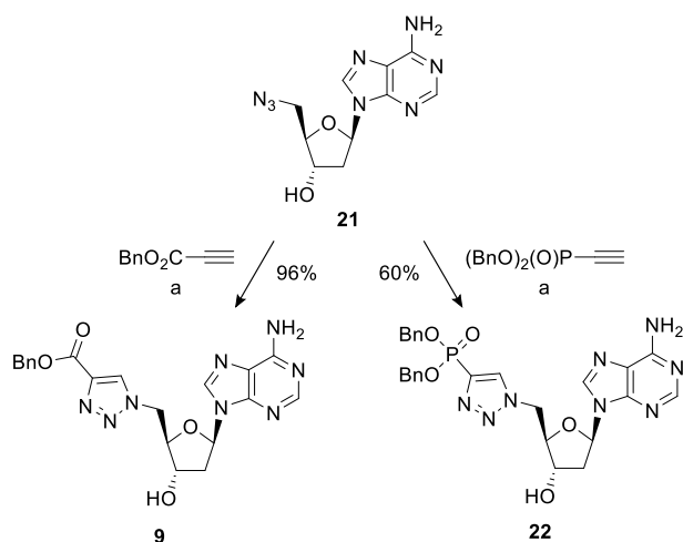
Scheme 4. Reagents and conditions: (a) Alkyne, 5 mol% \text{CuSO}_4 \cdot 5\text{H}_2\text{O} , 10 mol% sodium ascorbate, t\text{-BuOH}/\text{H}_2\text{O} (1:1), RT;
