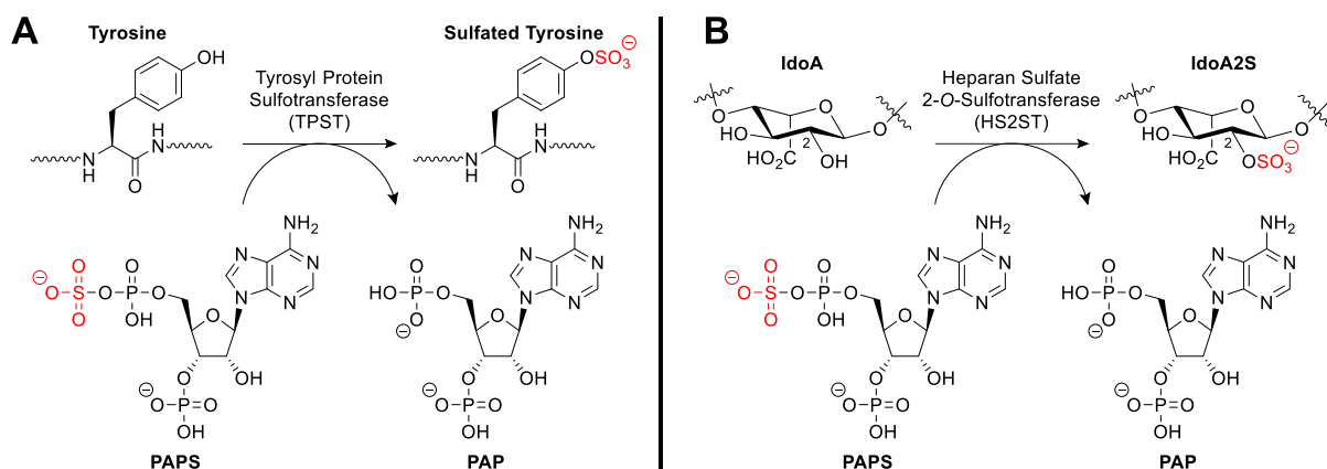
Fig. 1. (A) Tyrosylprotein sulfotransferase catalysed sulfation of a tyrosine residue. (B) Heparan sulfate 2-O-sulfotransferase catalysed sulfation of an iduronic acid (IdoA) subunit of heparan sulfate.
