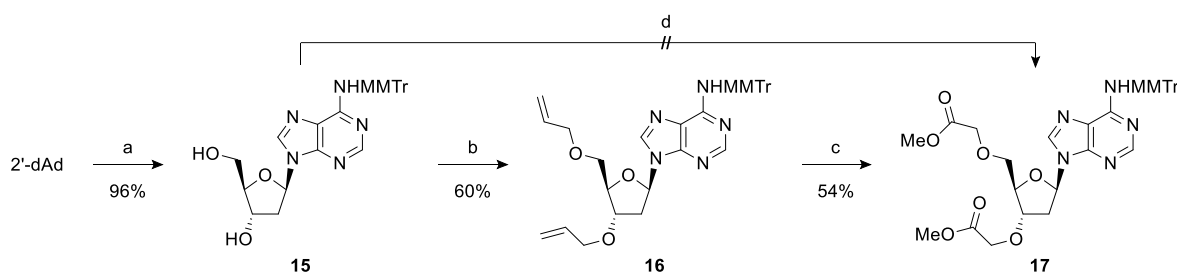
Scheme 1. Reagents and conditions: (a) TMSCl, pyridine, MMTrCl, 0 °C to RT then aq. NH 3 ; (b) NaHMDS, Allyl bromide, TBAI, DMF, -20 °C to RT; (c) O 3 , NaOH, MeOH, DCM, -78 °C, then AcOH; (d) NaHMDS, methyl bromoacetate, TBAI, DMF, -20 °C to RT.
