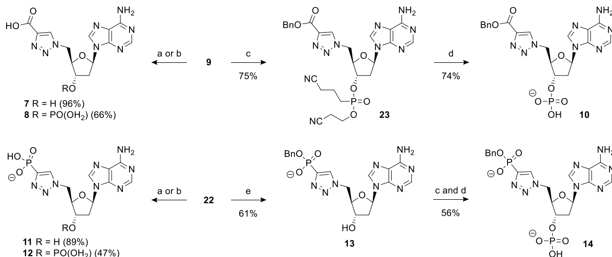
Scheme 5. Reagents and conditions: (a) 10% Pd/C, \text{H}_2 , 1 atm, \text{Et}_3\text{N} , MeOH, RT, then \text{Na}^+ -Dowex ® ; (b) i) i\text{-Pr}_2\text{NP}(\text{OBn})_2 , 1 H -tetrazole, MeCN, 0 °C to RT then m CPBA; ii) 10% Pd/C, \text{H}_2 , 1 atm, \text{Et}_3\text{N} , MeOH, RT, then \text{Na}^+ -Dowex ® ; (c) i\text{-Pr}_2\text{NP}(\text{OCH}_2\text{CH}_2\text{CN})_2 , 1 H -tetrazole, MeCN, 0 °C to RT then m CPBA; (d) TMG, TMSCl, MeCN, RT, then aq. \text{NH}_3 ; (e) NaI, MeCN, 80 °C; abbreviations: TMG = 1,1,3,3-Tetramethylguanidine.
