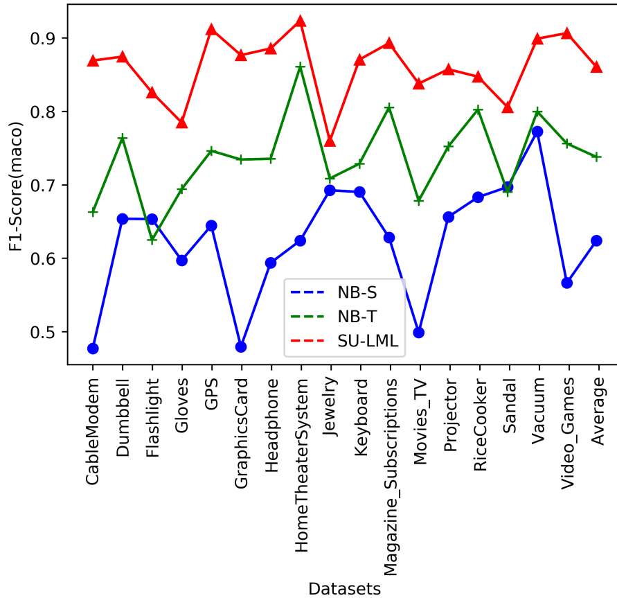
Fig. 2. F1 Score in Self-Study Stage
