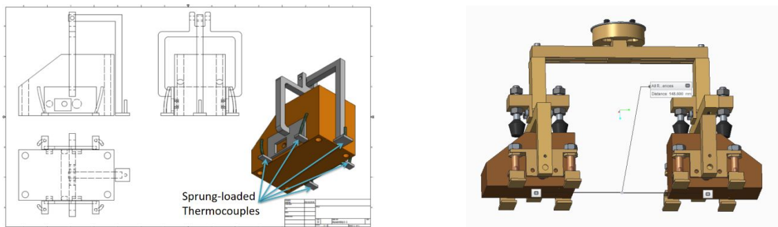
Figure 2. Ultrasound sensor head – acoustic wedge with sprung thermocouples (left) and twin head (right)
