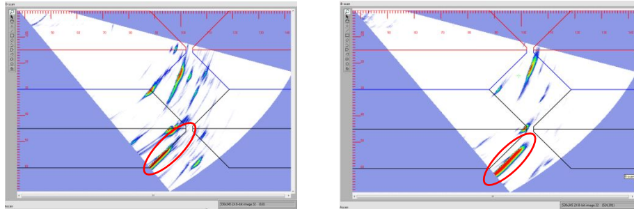
Figure 4. Comparison of reference image at 21.6°C (left) and image at 150°C (right) showing shift in reference feature by around 3mm
