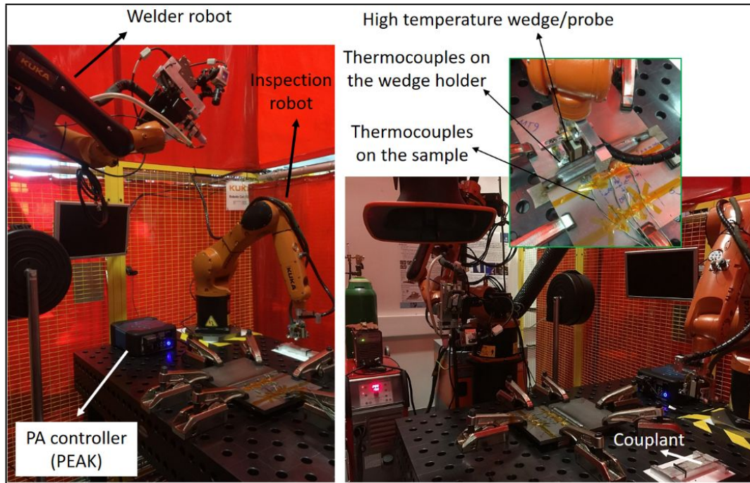
Figure 1. In-process inspection of multi-pass robotic welding
