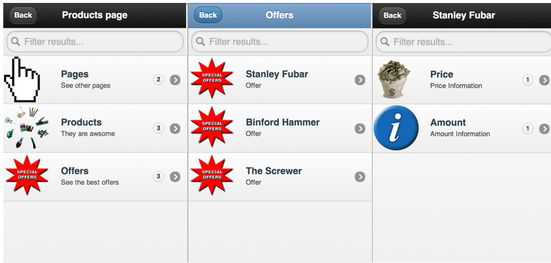
Fig. 9 SWC – an instance-based mobile data browser.
