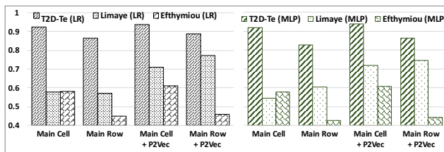
Figure 3: Accuracy with and without P2Vec concatenation. Average word2vec is used for cell embedding.
