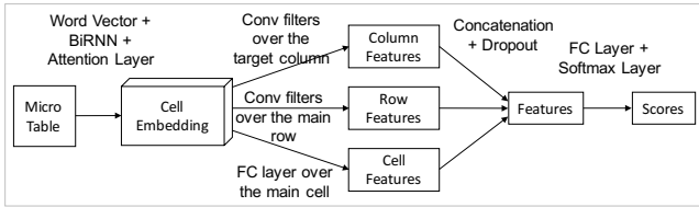
Figure 1: A brief view of the HNN architecture.
