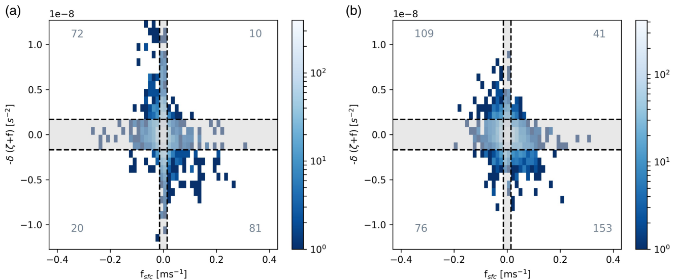
FIGURE 5 Phase space of stretching term versus surface forcing for (a) 1 January 1981 and (b) 17 January 1982. Colours indicate the density of points. Numbers in the corners denote the total number of observed points in each quadrant outside of the grey bars, which represent the thresholds below which data are excluded from the analysis
