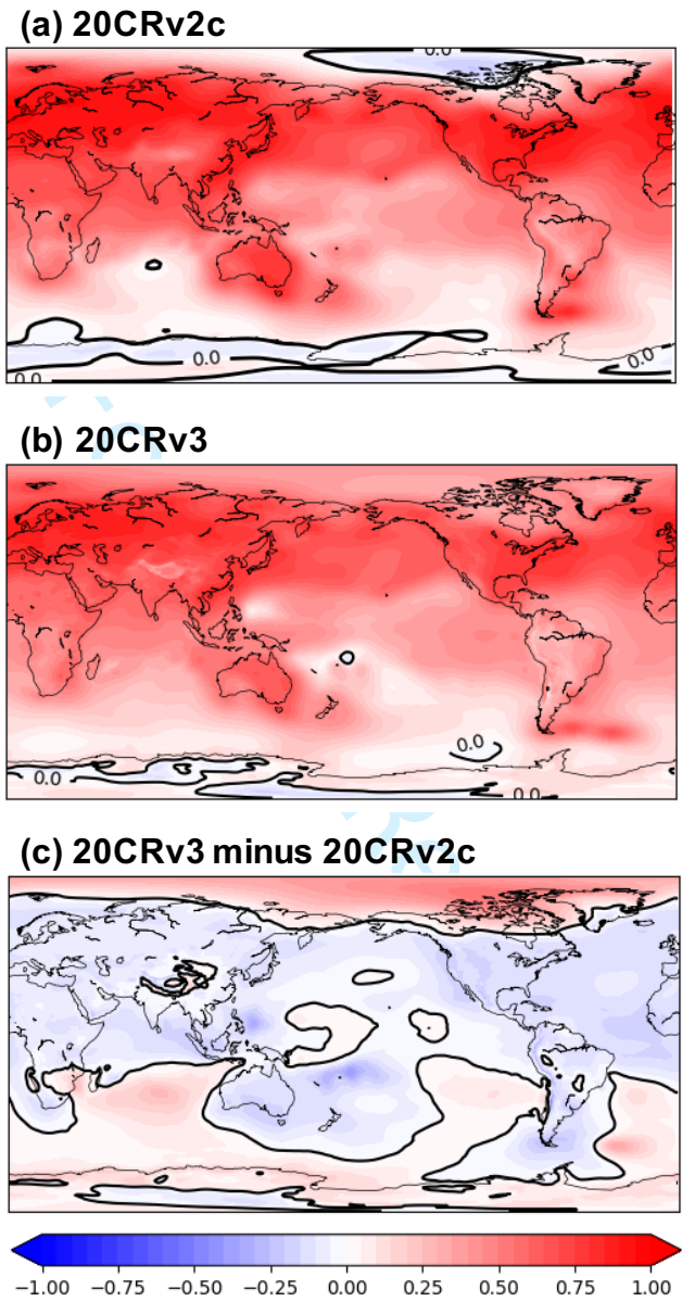
43 FIGURE 4 Maps of normalized confidence of SLP averaged over JFM for 1916-1918 from (a) 20CRv2c and (b) 44 20CRv3, as well as (c) the difference (20CRv3 minus 20CRv2c). In (a)-(b), zero (black contour) represents climatological 45 uncertainty, blue represents less certainty than climatology, and red represents more certainty. In (c), red represents an 46 increase in confidence from 20CRv2c to 20CRv3, and blue a decrease.
