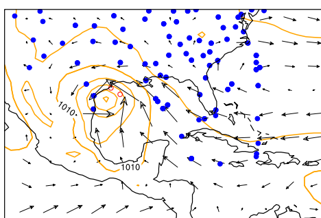
(c) ERA-20C
