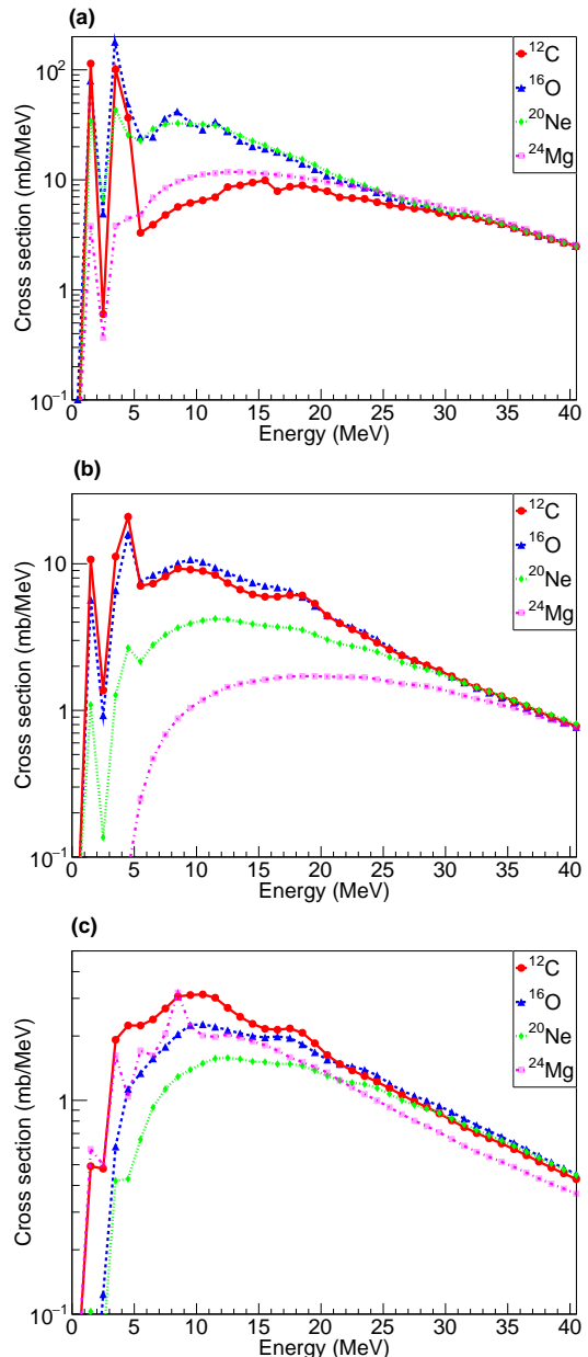
FIG. 5. Distribution of \alpha -particle energies in the center-of-mass system from the EHF for a beam energy of (a) 160 MeV, (b) 280 MeV and (c) 400 MeV. The yields from the population of different initial nuclei are shown in different colors with ^{12}\text{C} (red solid with circles), ^{16}\text{O} (blue short-dashed with triangles), ^{20}\text{Ne} (green dotted with diamonds) and ^{24}\text{Mg} (magenta dot-dashed with squares) with the lines guiding the eye between the data points.
