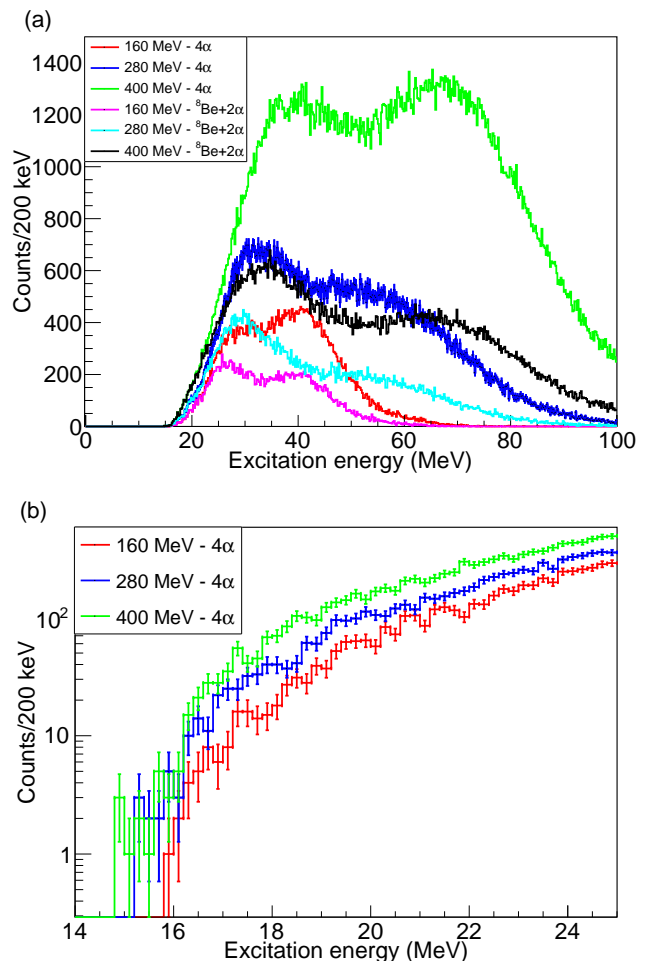
FIG. 21. Excitation for ^{16}\text{O} for the three beam energies showing all decays to 4 \alpha -particles in lin-lin (a) for a wide excitation range and log-lin (b) for near the 4- \alpha threshold. Also shown (top) is the contribution where a pair of the 4 \alpha -particles form ^8\text{Be}(g.s) .
