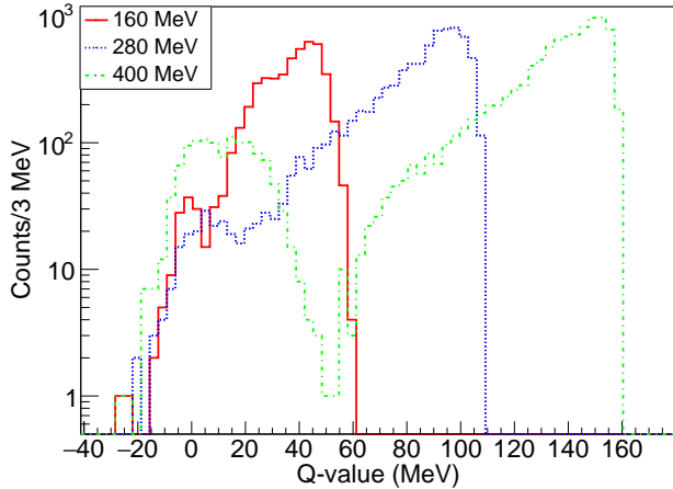
FIG. 27. (Negative) Q-value for the break-up of the compound nucleus into {}^{12}\text{C}(0_2^+) + {}^{16}\text{O} by reconstructing the {}^{16}\text{O} from the measurement of the {}^{12}\text{C}(0_2^+) from 3 \alpha -particles.
