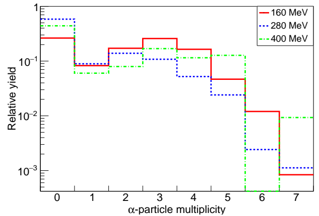
FIG. 17. True \alpha -particle multiplicity for the three beam energies of 160 (red), 280 (blue), and 400 (green) MeV. For each beam energy the total number of counts is normalized to 1.
