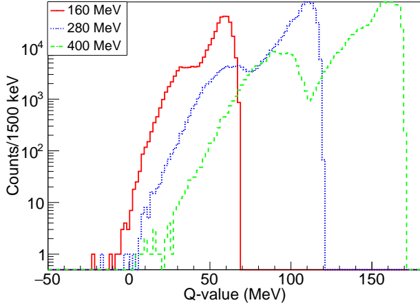
FIG. 26. (Negative) Q-value for the break-up of the compound nucleus into {}^8\text{Be}(\text{g.s.}) + {}^{20}\text{Ne} by reconstructing the {}^{20}\text{Ne} from the measurement of the {}^8\text{Be}(\text{g.s.}) from 2 \alpha -particles.
