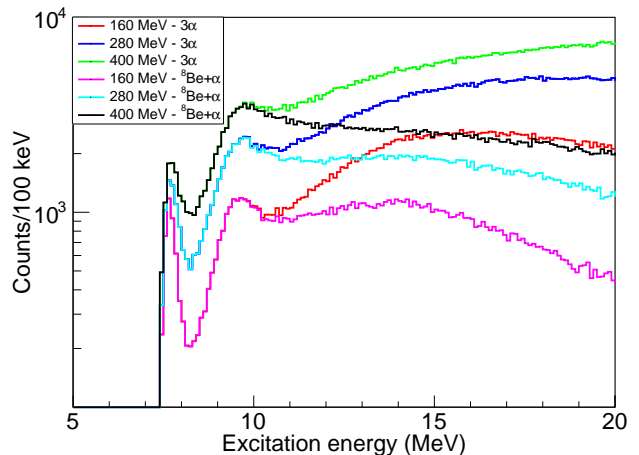
FIG. 19. Excitation function for ^{12}\text{C} showing the results for the three beam energies of 160, 280, and 400 MeV as well as those events where the intermediate decay product corresponds to the ^8\text{Be}(g.s) .
