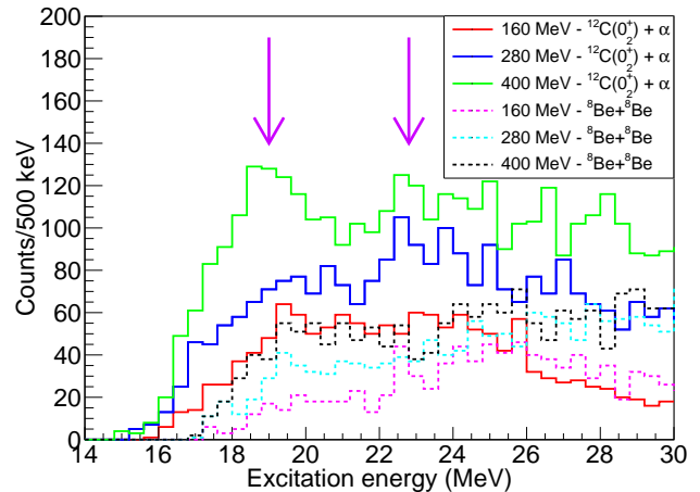
FIG. 23. Excitation function in ^{16}\text{O} for the clustered ^{12}\text{C}(0_2^+)+\alpha (solid lines) and ^8\text{Be}+^8\text{Be} decay paths (dashed) for the 160 (red/magenta), 280 (blue/cyan), and 400 (green/black) MeV data for the (^{12}\text{C}(0_2^+)+\alpha)/^8\text{Be}+^8\text{Be} channel. The violet arrows indicate a possible increased yield in the ^{12}\text{C}(0_2^+)+\alpha channel.
