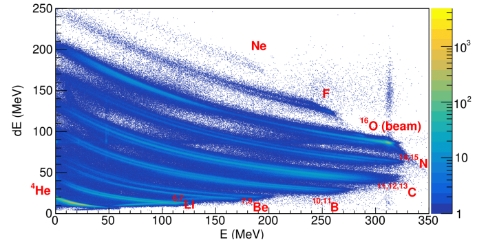
FIG. 7. Yields in the FARCOS detector for E_b = 400 MeV with the different loci labeled.
