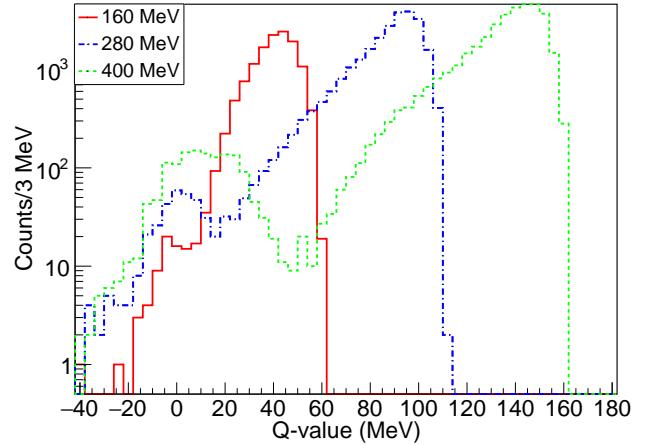
FIG. 28. (Negative) Q-value for the break-up of the compound nucleus into {}^{12}\text{C}(3_1^-) + {}^{16}\text{O}^* by reconstructing the {}^{16}\text{O} from the measurement of the {}^{12}\text{C}(3_1^-) from 3 \alpha -particles.
