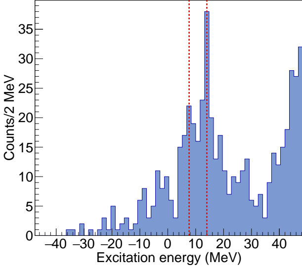
FIG. 30. Projection of the region between the red lines in Fig. 29c showing the excitation energy in ^{12}\text{C} as determined from the measurement of the 4- \alpha breakup with excitation energies between 50 and 95 MeV in ^{16}\text{O} . The two red lines guide the eye to the locations of the enhancements at 7.65 MeV and 14 MeV which may be as a consequence of the highly-clustered states at those excitation energies. A small component corresponding to the ^{12}\text{C}(\text{g.s.}) can also be seen at 0 MeV.
