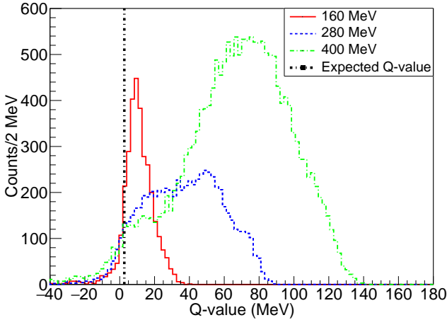
FIG. 31. Q-value for ^{20}\text{Ne}^* + ^8\text{Be}^* while reconstructing the missing ^8\text{Be} from the measured ^{20}\text{Ne} from 5 \alpha -particle events.
