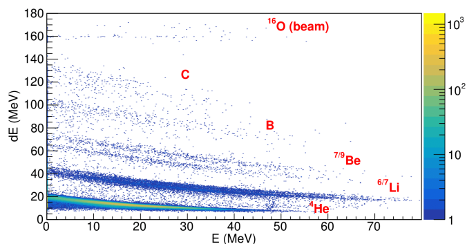
FIG. 9. Yields in the FARCOS detector for E_b = 160 MeV with the different loci labeled.
