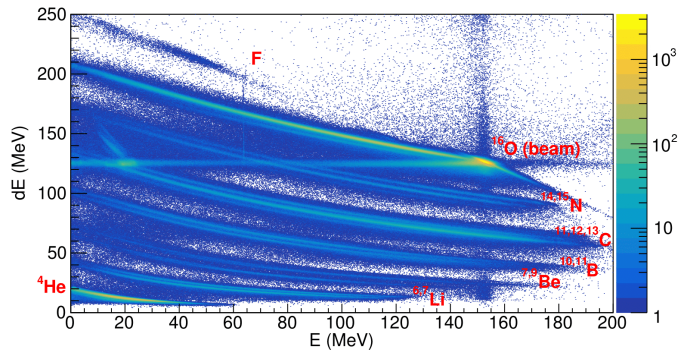
FIG. 8. Yields in the FARCOS detector for E_b = 280 MeV with the different loci labeled.
