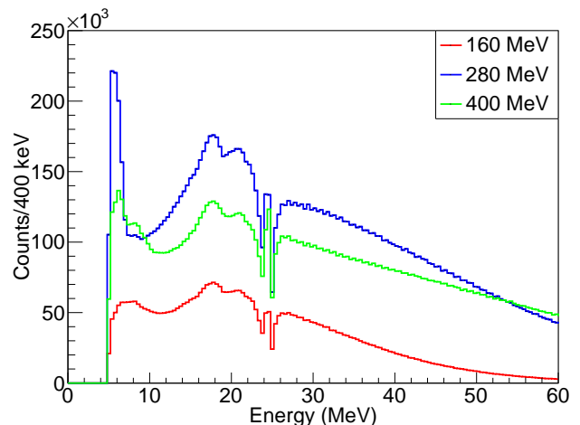
FIG. 15. Kinetic energy distribution of the \alpha -particles measured in CHIMERA and FARCOS. The discontinuities around 24 MeV are due to a gap in the TOF PID and the \Delta E -E PID for varying thicknesses of the silicon ( \Delta E ) detector.
