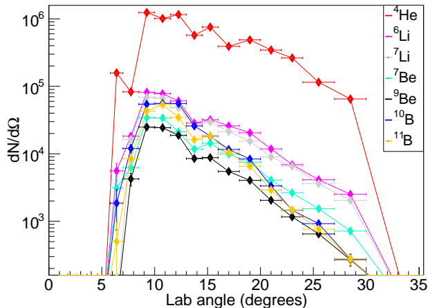
FIG. 10. Yields per solid angle in the CHIMERA detector for E_b = 400 MeV as a function of angle for the non \alpha -conjugate nuclei in comparison to {}^4\text{He} .
