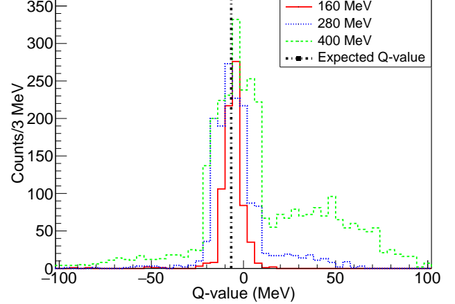
FIG. 32. (Negative) Q-value for ^{12}\text{C}(^{16}\text{O}, ^{24}\text{Mg}^*) while reconstructing the missing \alpha from ^{24}\text{Mg}^* .
