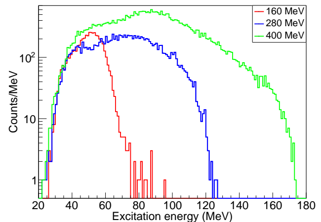
FIG. 24. Excitation function of ^{20}\text{Ne} for states decaying to 5 \alpha -particles.
