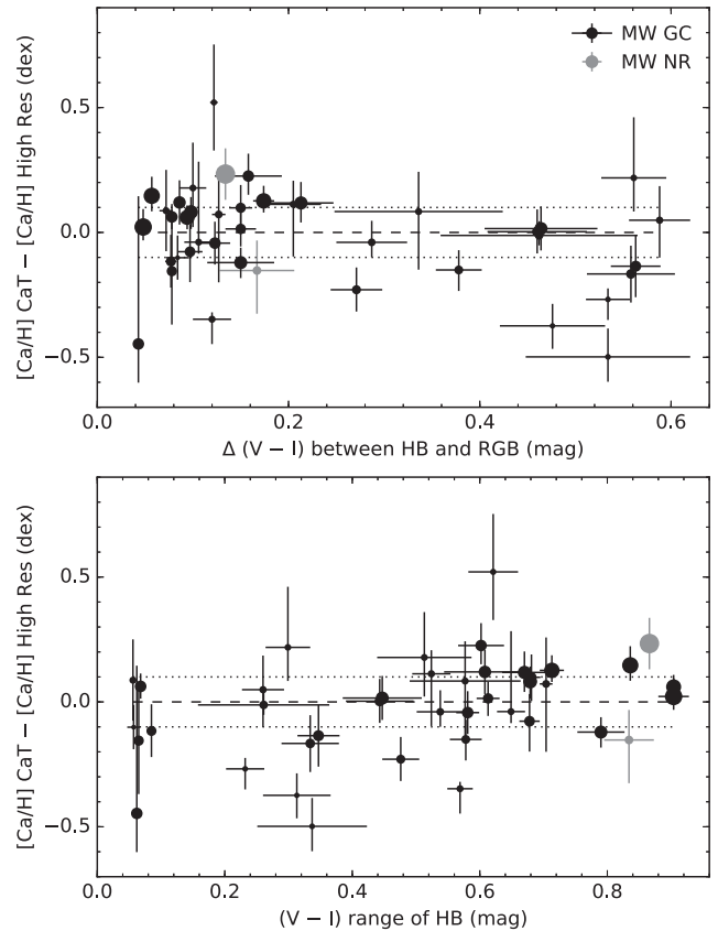
Figure 23. Effects of HB morphology on the CaT. Top: difference between literature and our CaT-based [\text{Ca}/\text{H}] as a function of the (V - I) colour difference between the red edge of HB and the RGB (the L1 parameter from Milone et al. 2014). Bottom: difference between literature and our CaT-based [\text{Ca}/\text{H}] as a function of the (V - I) colour range of the HB (the L2 parameter from Milone et al. 2014). The colours, shapes, and size of the points are the same as in Fig. 18. As in Fig. 19, the dashed line shows \Delta[\text{Ca}/\text{H}] = 0 , while the dotted lines show \Delta[\text{Ca}/\text{H}] = \pm 0.1 . The strength of the CaT does not significantly depend on the HB morphology.
