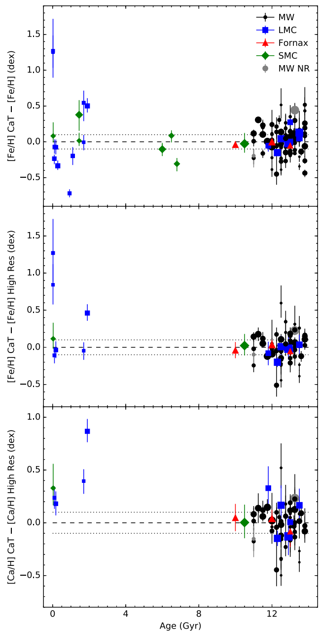
Figure 21. Top: differences in CaT-based [\text{Fe}/\text{H}] with all literature [\text{Fe}/\text{H}] as a function of age. Middle: differences in [\text{Fe}/\text{H}] between CaT-based and high-resolution spectroscopy values. Bottom: differences in [\text{Ca}/\text{H}] between CaT-based and literature values. The dashed line shows \Delta[\text{Fe}/\text{H}] or \Delta[\text{Ca}/\text{H}] = 0 , while the dotted lines show \Delta[\text{Fe}/\text{H}] or \Delta[\text{Ca}/\text{H}] = \pm 0.1 . For ages older than 3 Gyr, the strength of the CaT is independent of age. GCs between 1.4 and 2 Gyr with significant contributions from C stars show significantly stronger CaT strengths than predicted by our CaT–metallicity relations but GCs without significant numbers of C stars in this age range show the same CaT strengths as old GCs with the same [\text{Fe}/\text{H}] . GCs younger than 1.4 Gyr show CaT strengths slightly weaker than old GCs with the same [\text{Fe}/\text{H}] except for the youngest GCs ( < 25 Myr) which are dominated by RSGs. The CaT values of young ( < 3 Gyr) GCs are larger than their [\text{Ca}/\text{H}] would predict.
