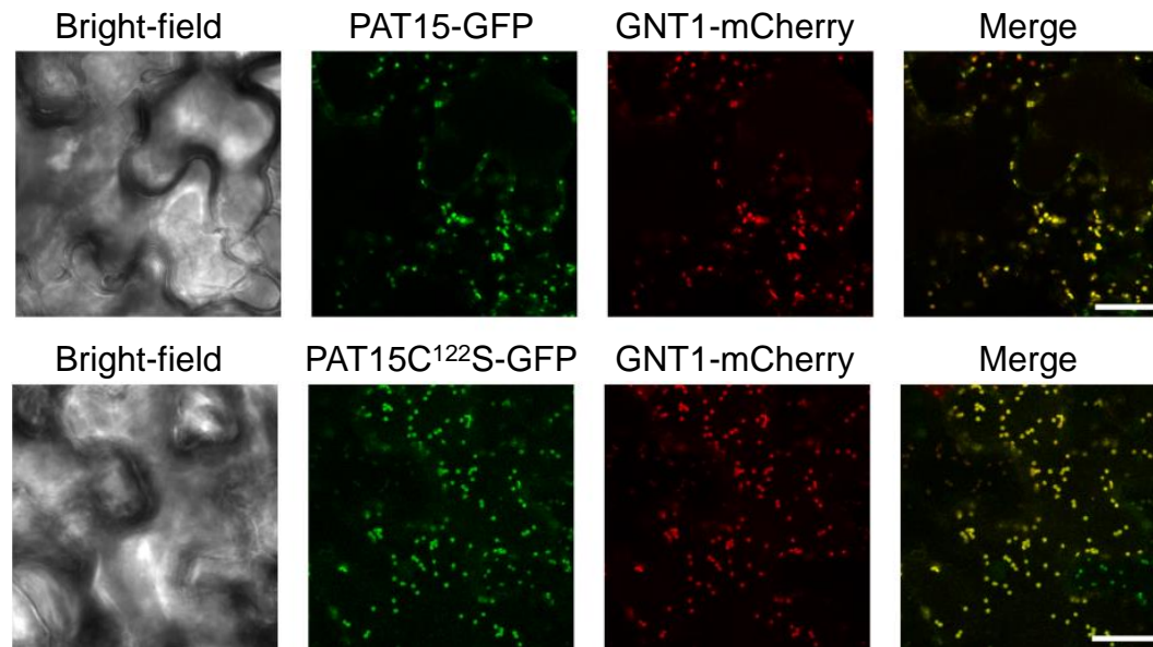
Fig 4. PAT15 is targeted to the Golgi. AtPAT15-GFP or AtPAT15C 122 S-GFP were co-expressed with AtGNT1-mCherry transiently in Arabidopsis seedlings. Localization of the fluorescent proteins were observed by laser scanning confocal microscopy. Bars = 15 \mu m.
