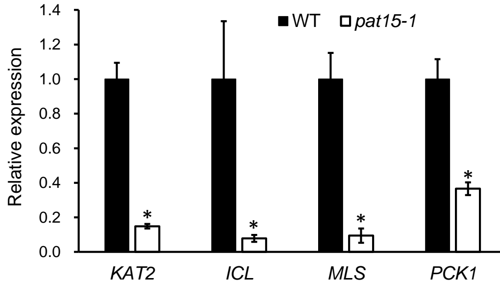
Fig. 8. Transcript levels of the key genes involved in lipid breakdown pathway were down-regulated during early seedling growth. Total RNA was extracted from 10 seedlings of WT or pat15-1 that were grown on \frac{1}{2} MS+1% Suc for 10 days in the dark. The relative expression level of each gene in the mutant was calculated where the transcript level of WT was regarded as 1. The experiments were repeated three times. * p < 0.05 in Student's t -test. KAT2 , 3-ketoacyl-CoA thiolase 2; ICL , isocitrate lyase; MLS , malate synthase; PCK1 , phosphoenolpyruvate carboxykinase 1.
