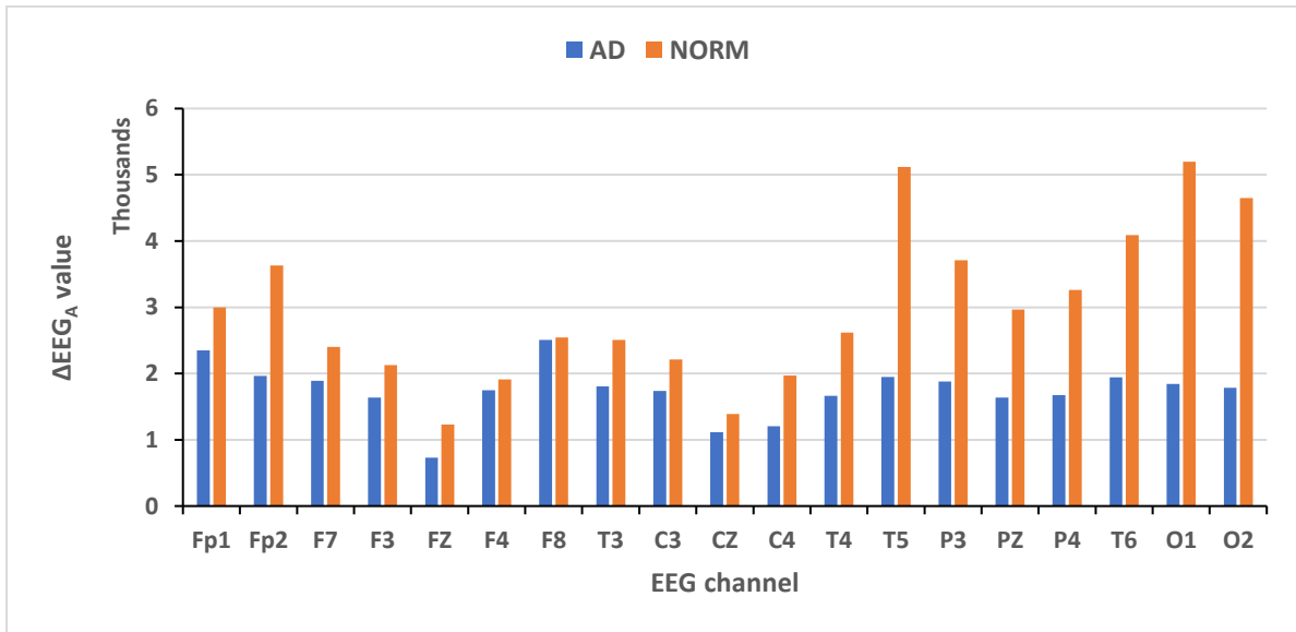
Figure 4-3: \Delta EEG_A values for one AD patient and one normal subject
