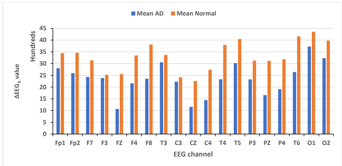
Figure 4-4: Mean \Delta EEG_A for AD patients and normal subjects
