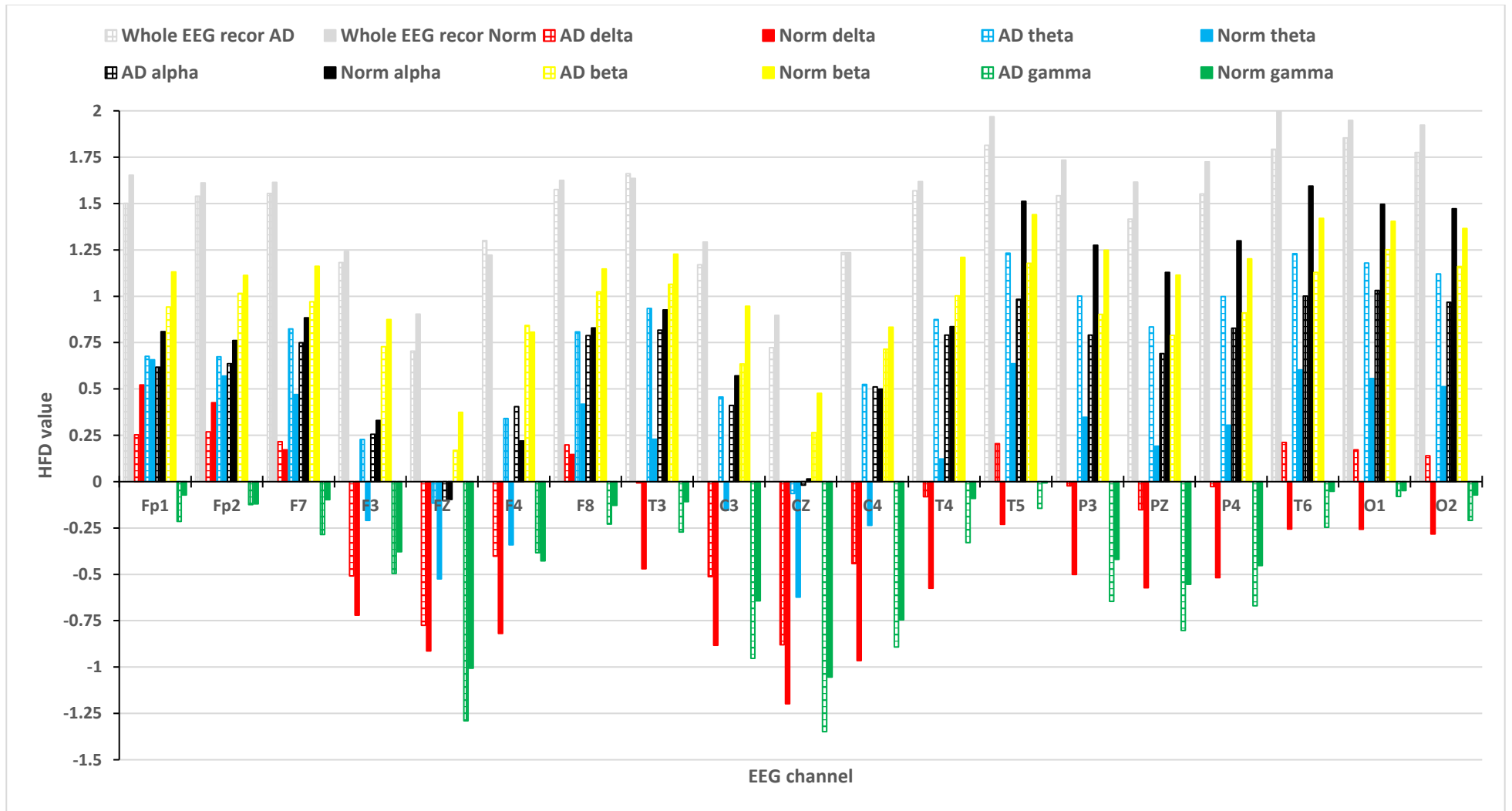
Figure 5-2: EEG biomarkers for HFD
