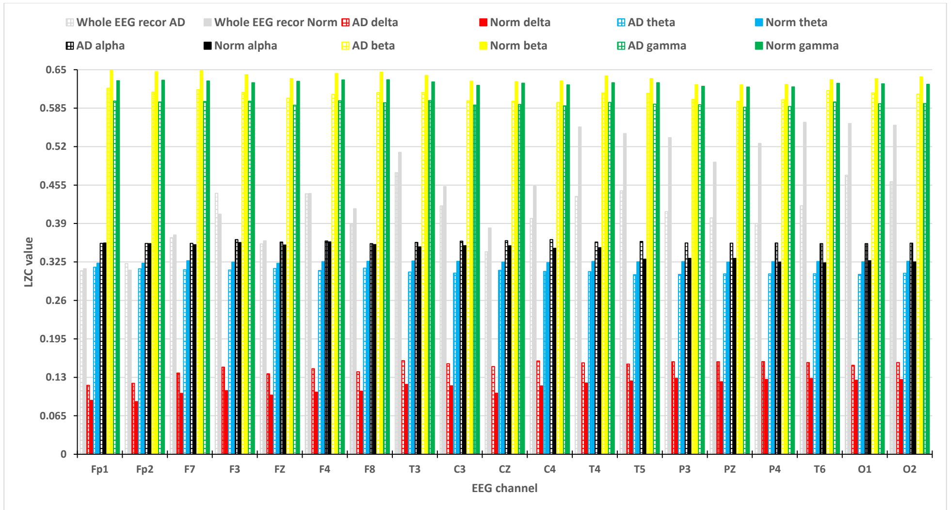
Figure 5-3: EEG biomarkers for LZC
