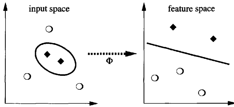
Figure 2-9: The idea of SVM
