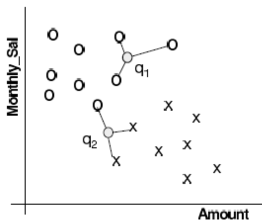
Figure 2-12: Example of 3-nearest neighbour classification
