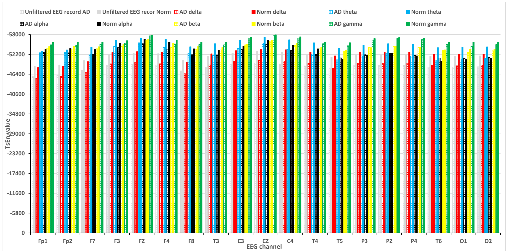
Figure 5-1: EEG biomarkers for TsEn
